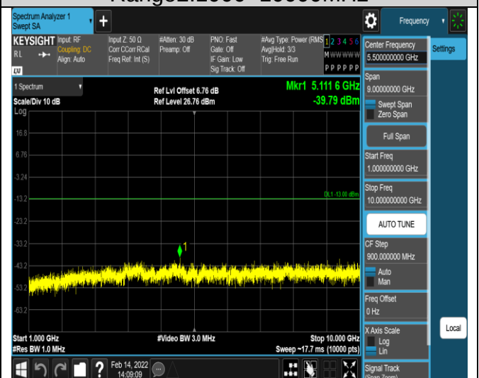
Band17-10MHz-QPSK-23800-1RB#0- Range2:1000~10000MHz
