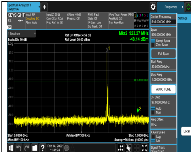
Band12-10MHz-QPSK-23095-1RB#0- Range1:30~1000MHz
