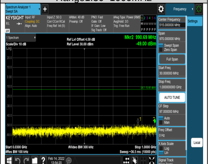
Band13-5MHz-16QAM-23205-1RB#0-
