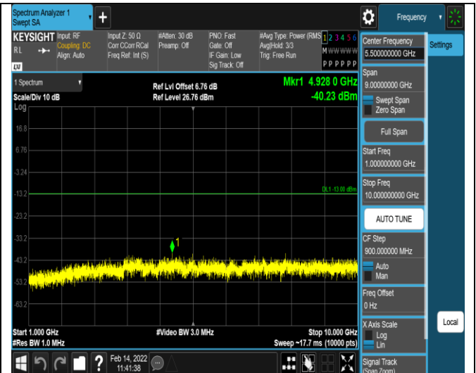
Band12-10MHz-QPSK-23095-1RB#0- Range2:1000~10000MHz
