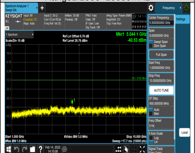
Band17-10MHz-16QAM-23780-1RB#0-
