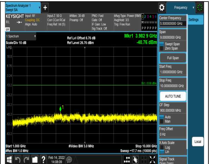
Band17-10MHz-QPSK-23790-1RB#0- Range2:1000~10000MHz
