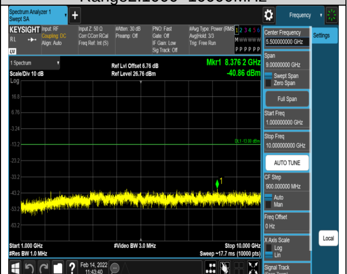
Band12-10MHz-16QAM-23060-1RB#0-
