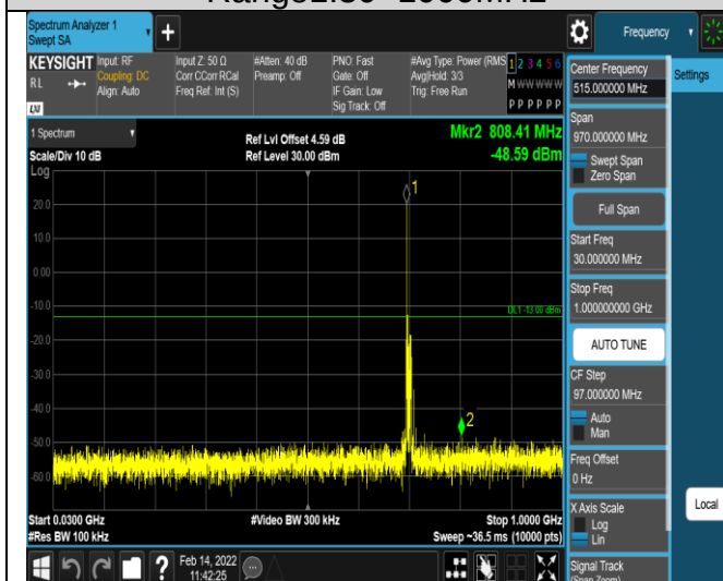
Band12-10MHz-QPSK-23130-1RB#0- Range1:30~1000MHz
