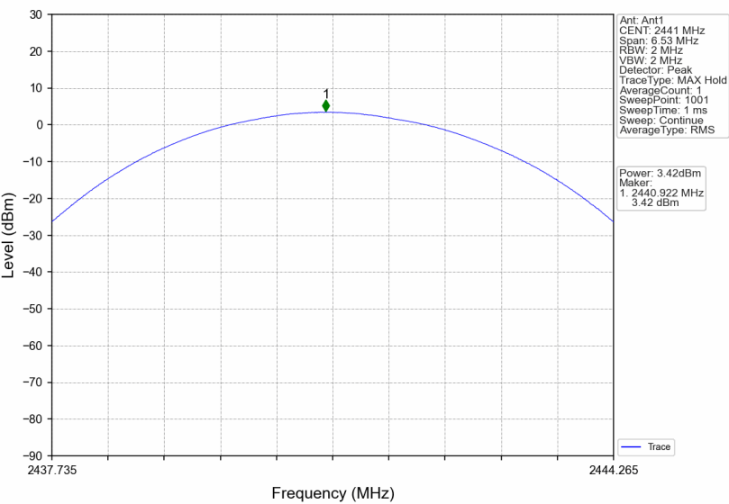
8DPSK_3DH5_MCH_2441MHz_Ant1_NTNV
