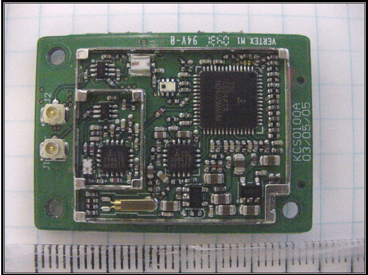
PHOTOGRAPH 25: TOP OF MODULE WITHOUT SHIELDS
