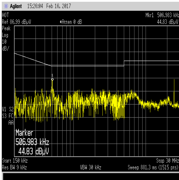
Hot Line at 120 V 60Hz
