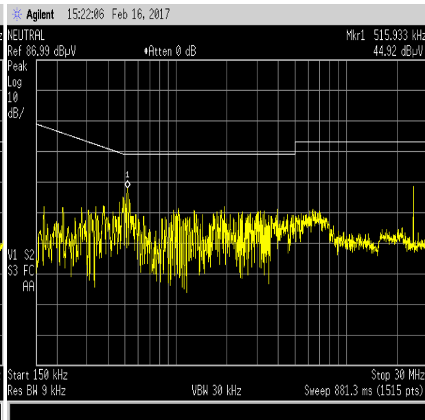
Neutral Line at 120 V 60 Hz
