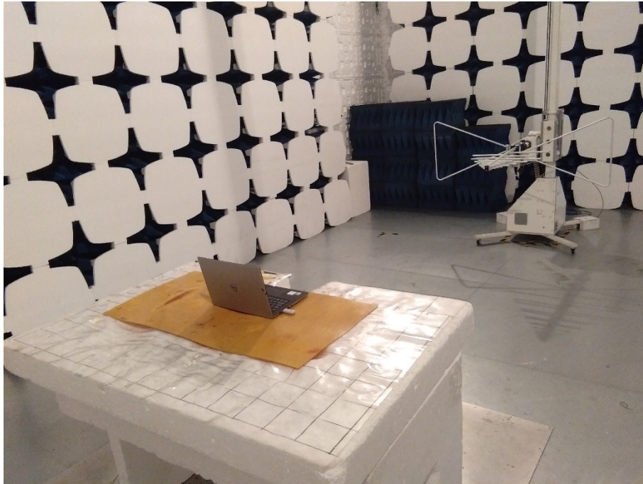
Radiated emissions below 1G
