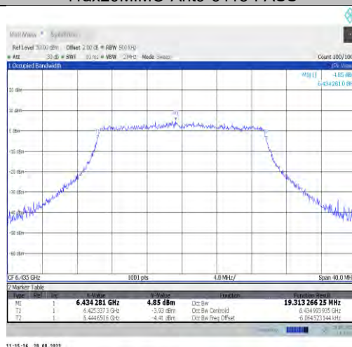
11ax20MIMO-Ant9-6435-PASS
