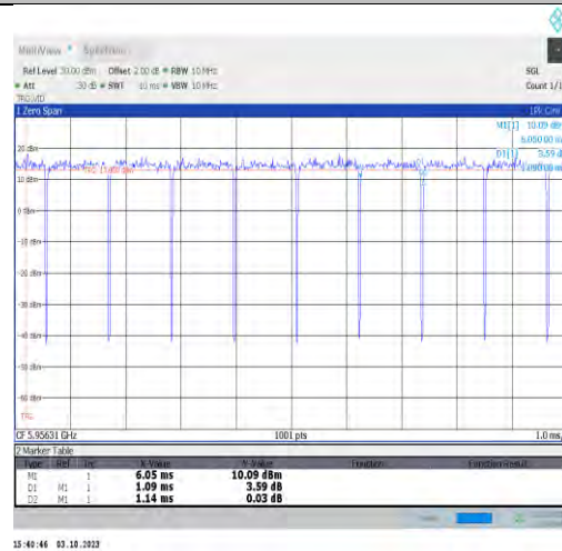
NTNV-11ax40MIMO-Ant9-5965
