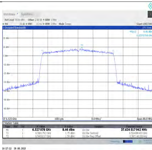
11ax40MIMO-Ant7-6525-PASS
