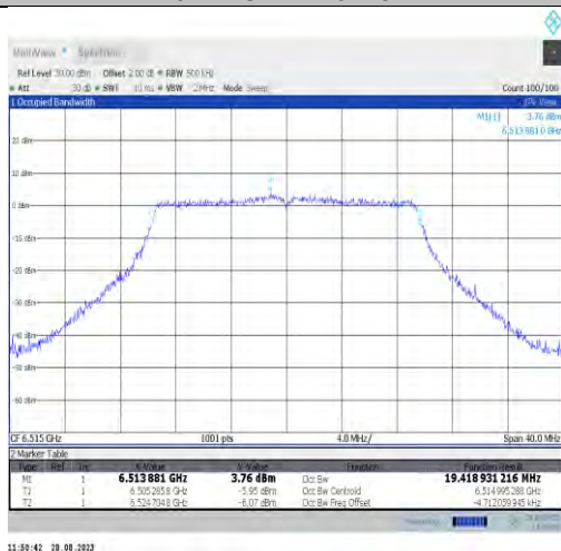
11ax20MIMO-Ant7-6515-PASS
