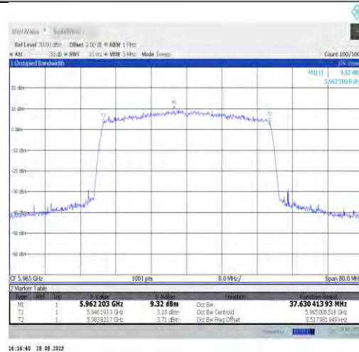
11x40MIMO-Ant9-5965-PASS
