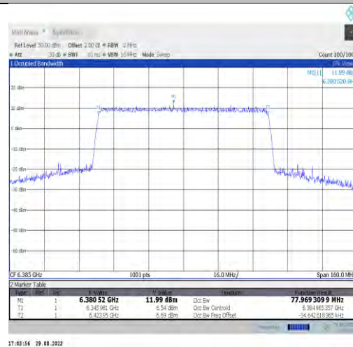
11x80MIMO-Ant9-6385-PASS
