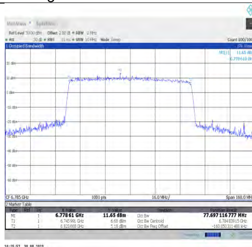
11x80MIMO-Ant9-6785-PASS
