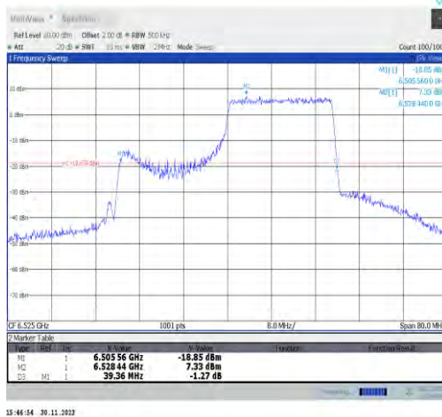
11ax40MIMO-Ant7-6525-242Tone-RU62
