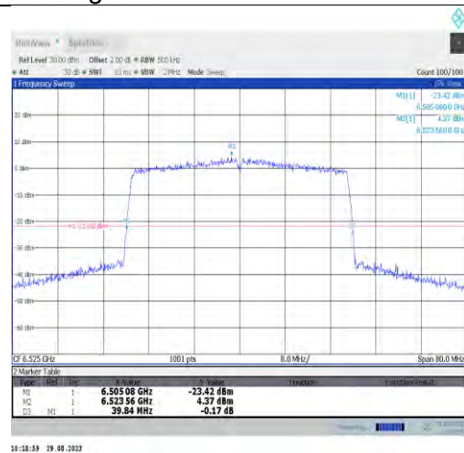
11ax40MIMO-Ant9-6525
