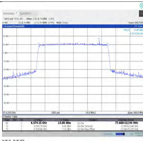
11ax80MIMO-Ant7-6545-PASS
