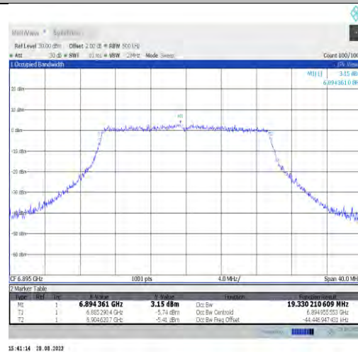
11ax20MIMO-Ant9-6895-PASS
