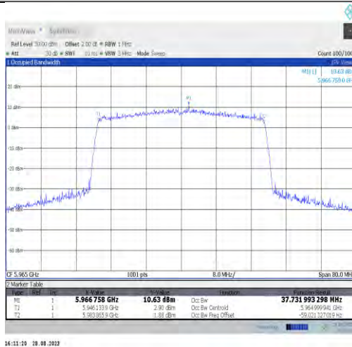
11x40MIMO-Ant7-5965-PASS
