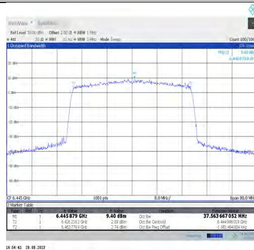
11ax40MIMO-Ant9-6445-PASS
