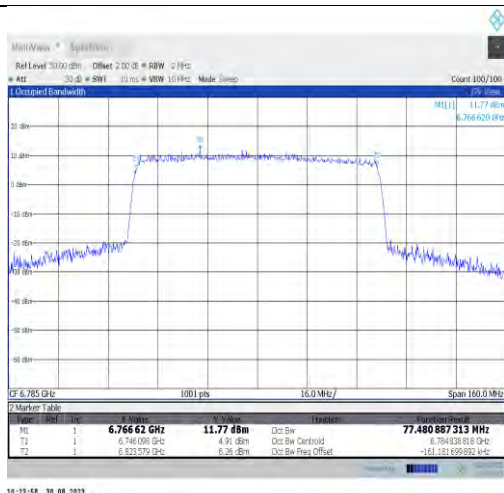
11x80MIMO-Ant7-6785-PASS
