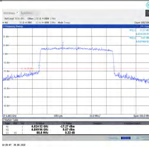
11ax80MIMO-Ant7-6865
