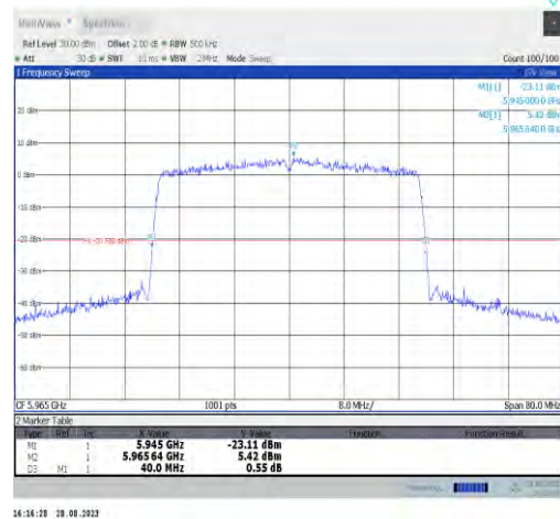
11ax40MIMO-Ant9-5965
