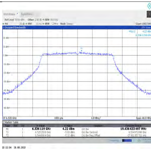
11x20MIMO-Ant7-6535-PASS
