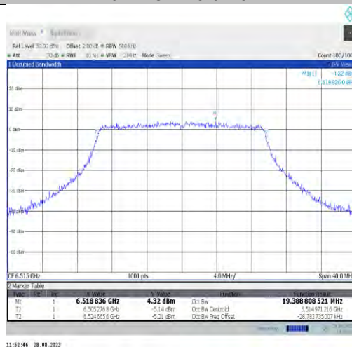
11ax20MIMO-Ant9-6515-PASS
