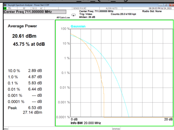
Band 17_50_Q16_High
