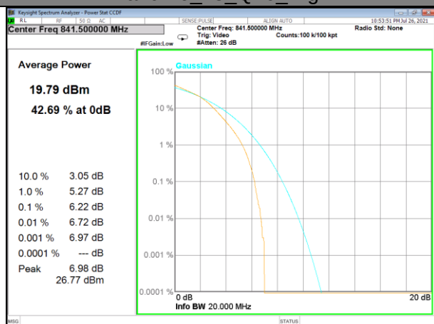
Band 26_75_Q16_High
