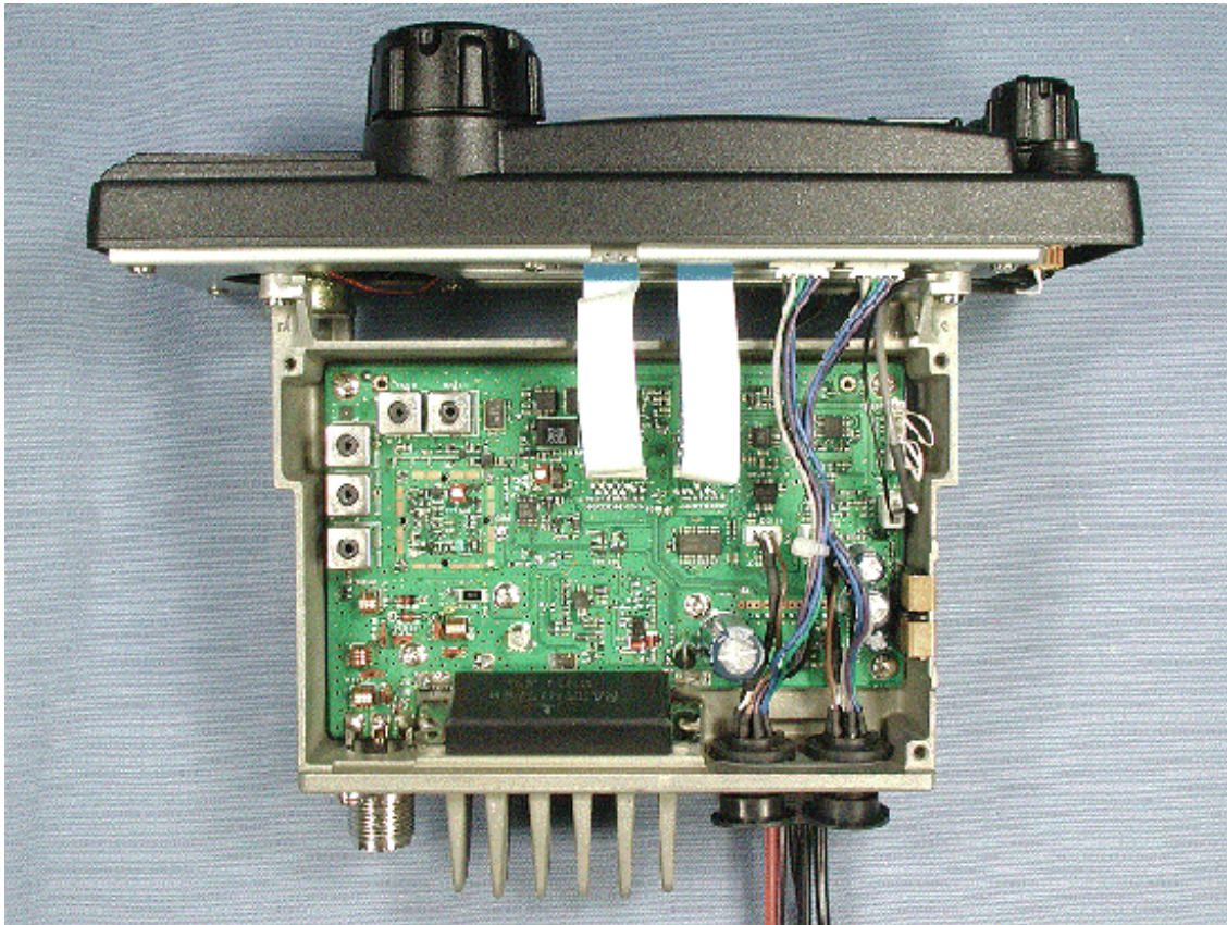
Bottom of EUT without Case (without Shield Cases)
