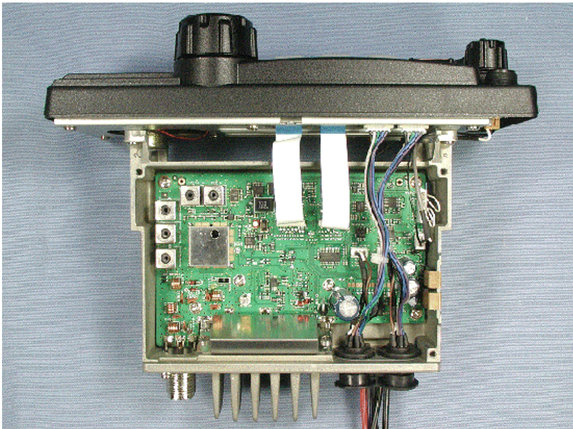
Bottom of EUT without Case (with Shield Cases)
