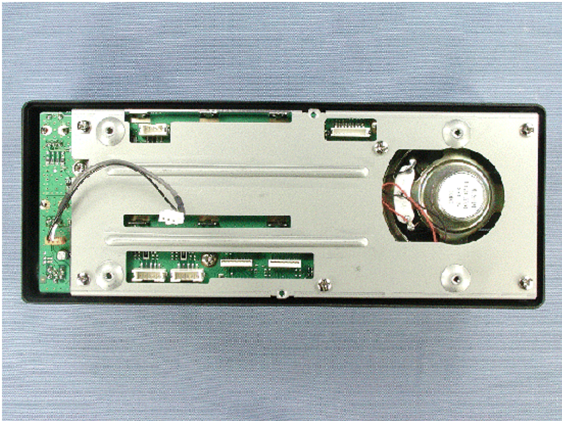
Inside of Panel with PWB (1)
