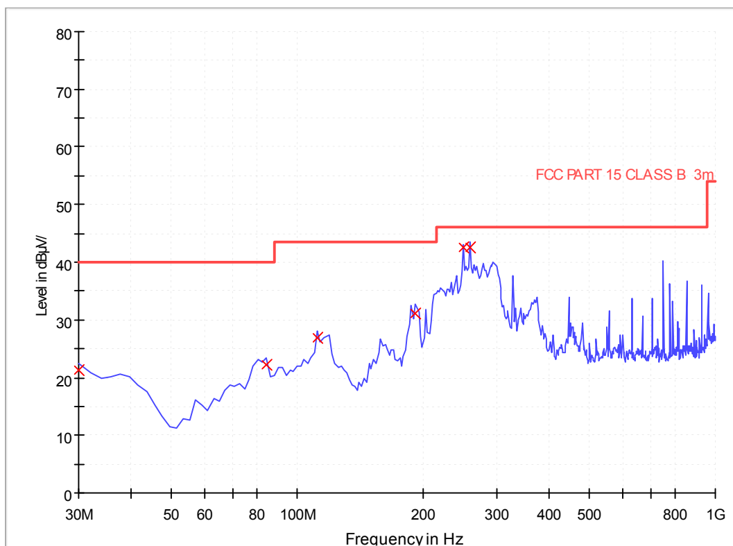
EMI Sweep-3M(30-1G)
