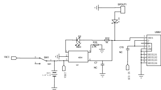
Charging, AUX circuit
