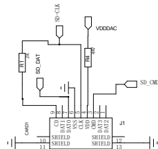
TF card socket circuit
