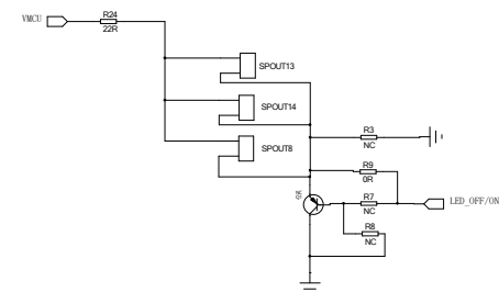
Lamp circuit
