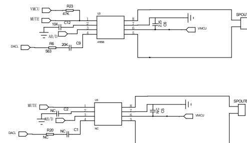
Power amplifier circuit
