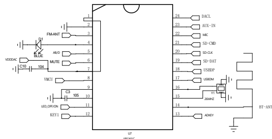
Main control, blue light, schematic diagram
