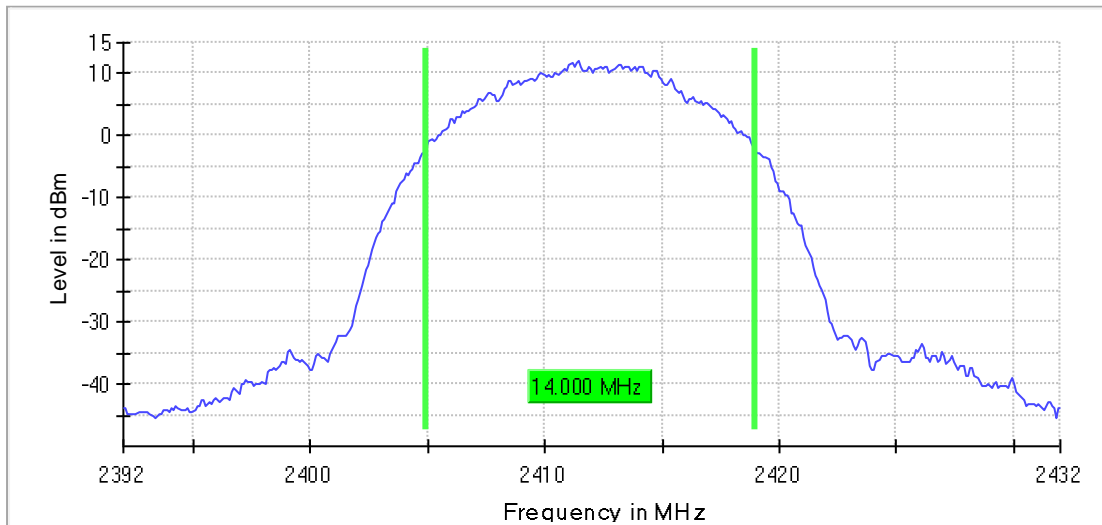
99% Occupied Bandwidth Mode 1 / CH0 (2412 MHz)
