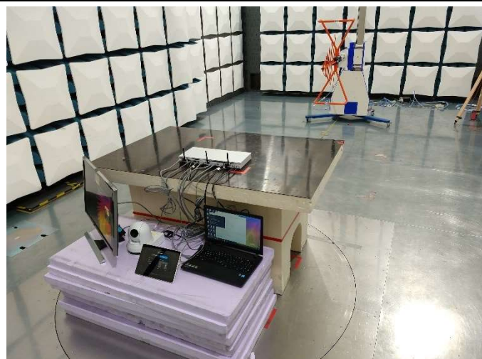
Test set-up for Radiated emissions measurements (Below 1GHz, CISPR)
