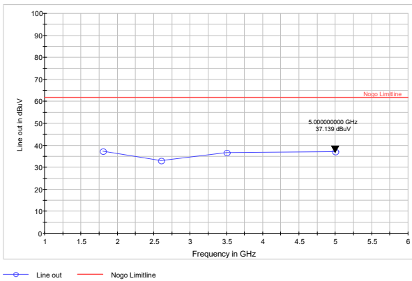
1800, 2600, 3500, 5000 MHz, 270 deg, horizontal polarization
