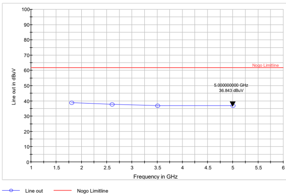
1800, 2600, 3500, 5000 MHz, 90 deg, horizontal polarization
