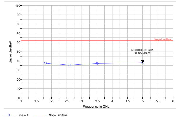
1800, 2600, 3500, 5000 MHz, 0 deg, vertical polarization
