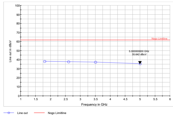
1800, 2600, 3500, 5000 MHz, 180 deg, vertical polarization
