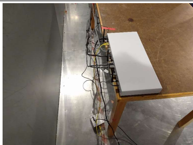
Test set-up for Conducted emissions measurements (Ethernet ports)
