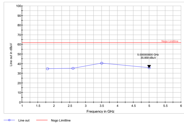
1800, 2600, 3500, 5000 MHz, 90 deg, vertical polarization
