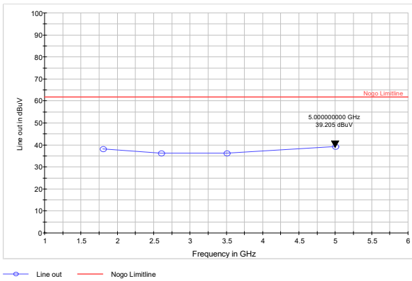
1800, 2600, 3500, 5000 MHz, 0 deg, horizontal polarization
