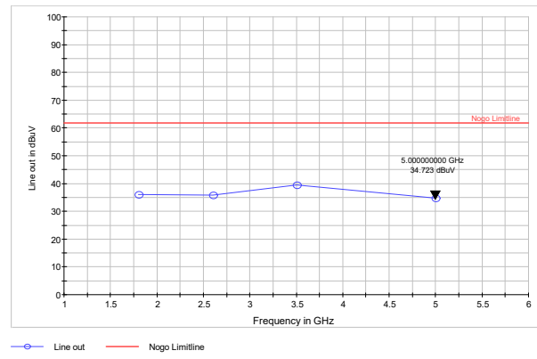
1800, 2600, 3500, 5000 MHz, 270 deg, vertical polarization
