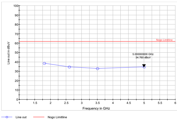
1800, 2600, 3500, 5000 MHz, 180 deg, horizontal polarization
