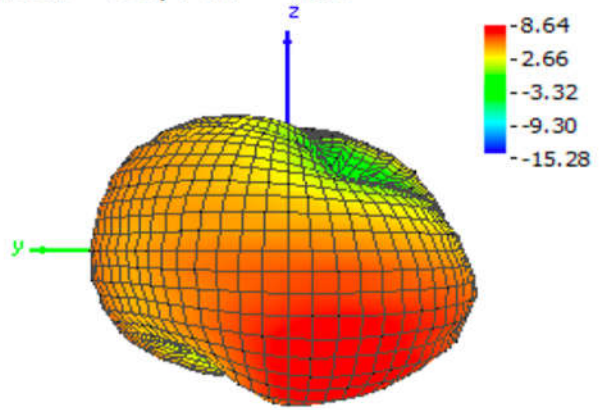
Theta = 90, Phi = 180
