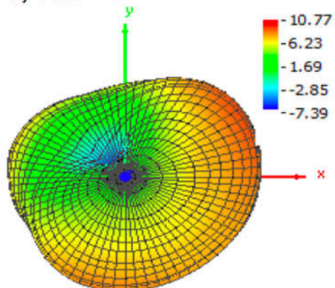
Theta = 0, Phi = 0
