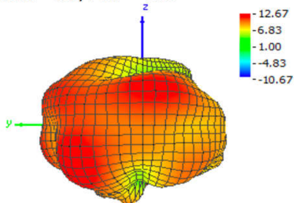
Theta = 90, Phi = 180
