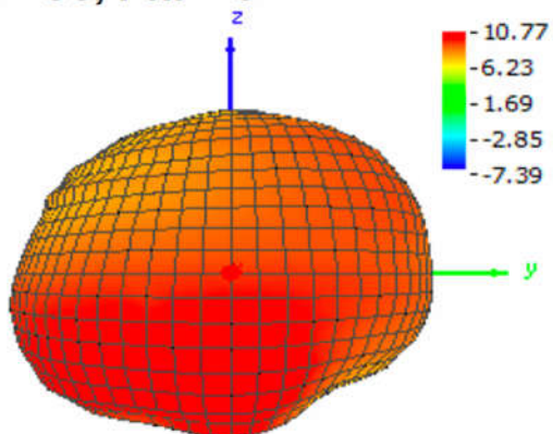
Theta = 90, Phi = 0
