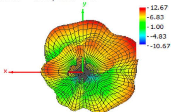
Theta = 180, Phi = 0
