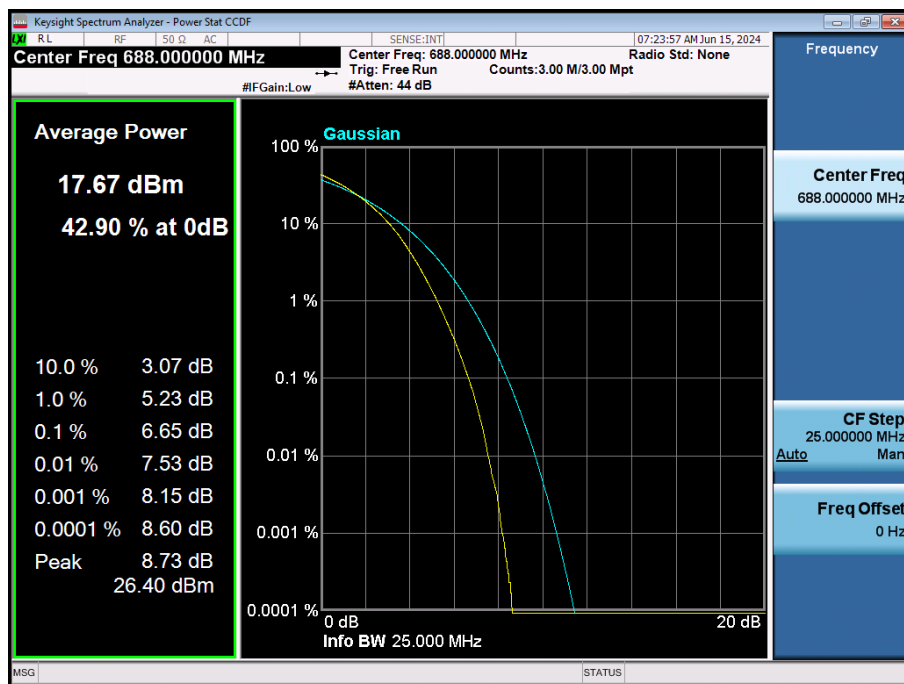
LTE Band 71 / 20 MHz / 256QAM / FULL RB Size
