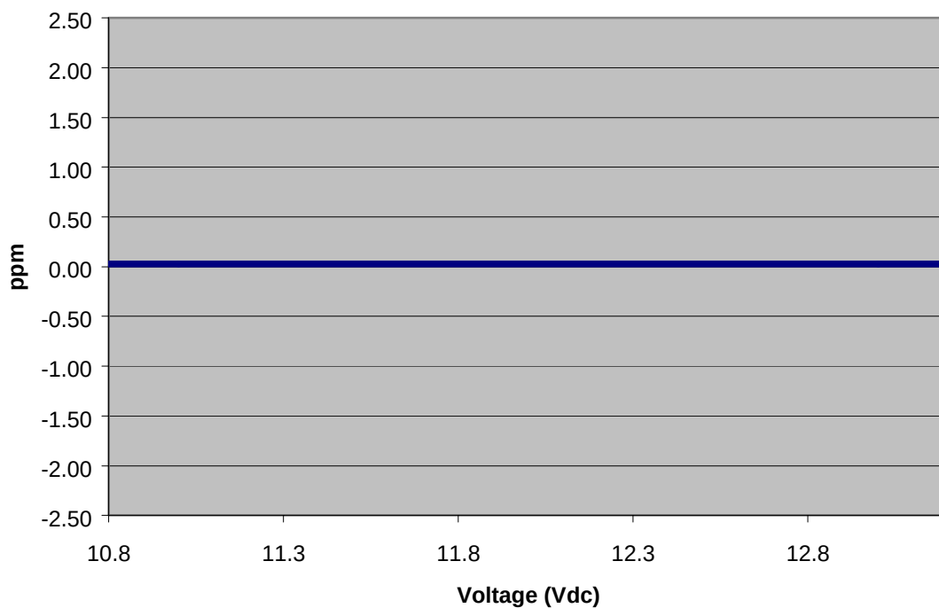
AMPS 800 Frequency Stability vs. Voltage (12.0 VDC Nominal) Carrier Frequency = 836.52 MHz Maximum Power Level (1.5 Watt)
