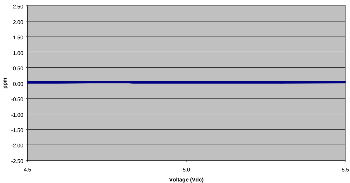
DAMPS 800 Frequency Stability vs. Voltage (5 VDC nominal) Carrier Frequency = 836.52 MHz Maximum Power Level (1.5 Watt)
