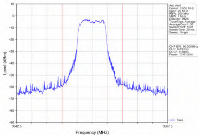
n78d_30kHz_SISO_NTNV_10MHz_DFT-s-OFDM 64 QAM_3555MHz_Inner_Full
