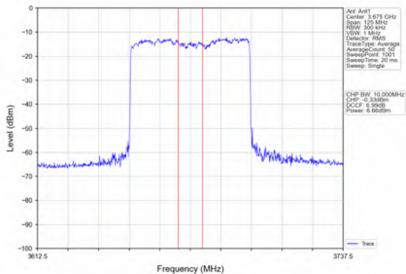
n78d_15kHz_SISO_NTNV_50MHz_CP-OFDM 256 QAM_3675MHz_Inner_Full
