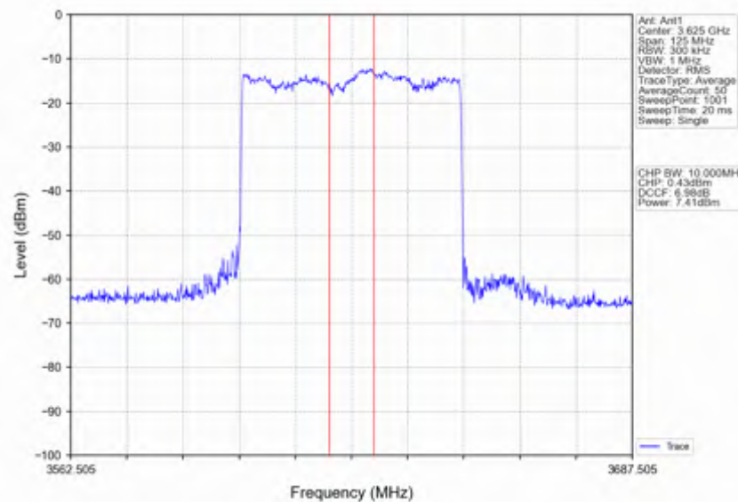
n78d 15kHz SISO NTNV 50MHz CP-OFDM 64 QAM 3625.005MHz Inner Full
