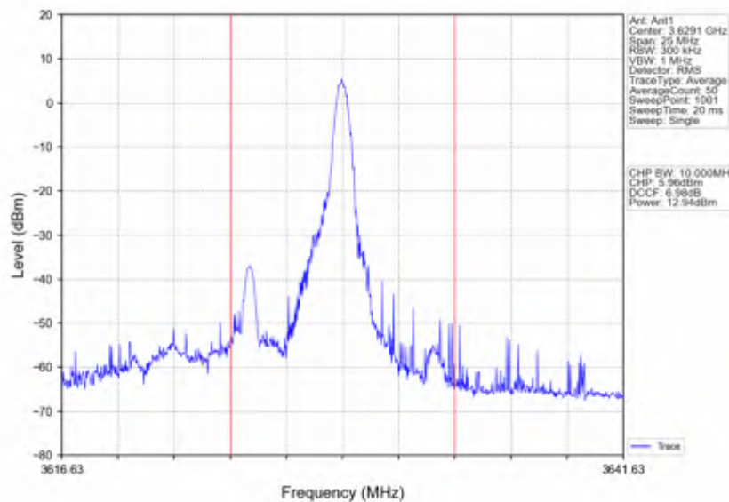
n78d_30kHz_SISO_NTNV_10MHz_DFT-s-OFDM_64_QAM_3624.99MHz_Edge_1RB_Right
