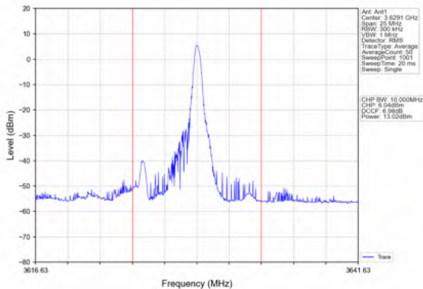
n78d_30kHz_SISO_NTNV_10MHz_DFT-s-OFDM PI/2 BPSK_3624.99MHz_Edge_1RB_Right
