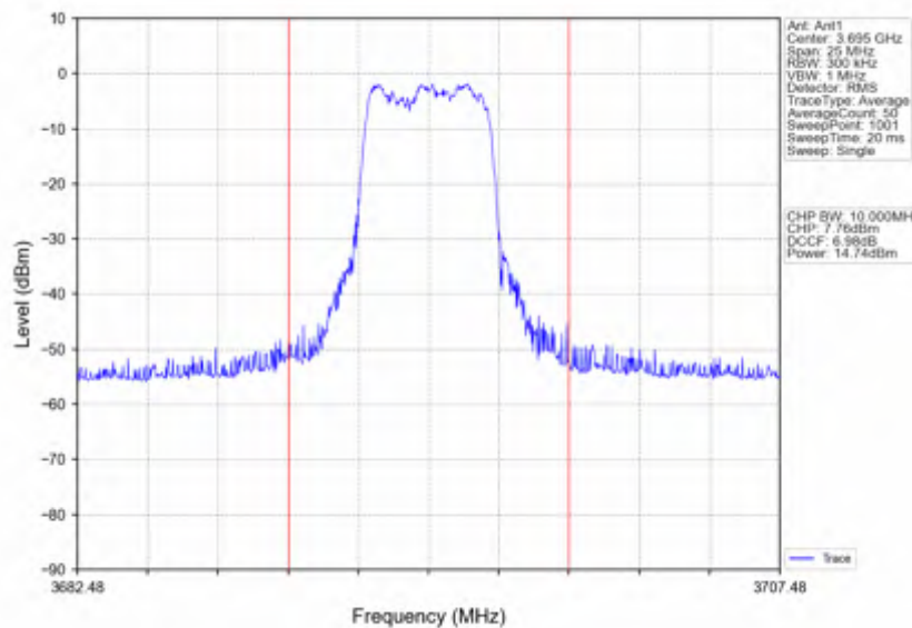
n78d_30kHz_SISO_NTNV_10MHz_CP-OFDM QPSK_3694.98MHz_Inner_Full
