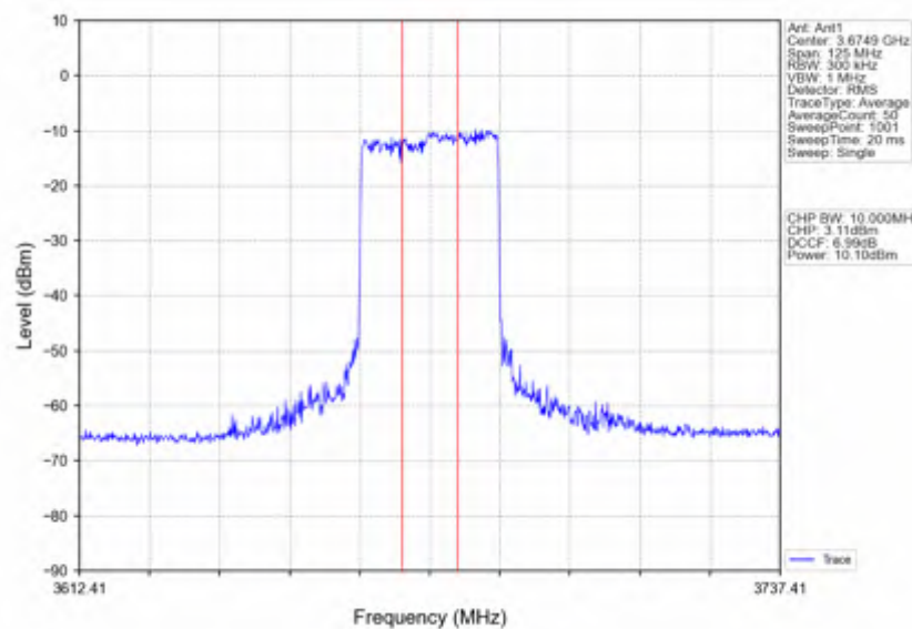
n78d_15kHz_SISO_NTNV_50MHz_DFT-s-OFDM QPSK_3675MHz_Inner_Full
