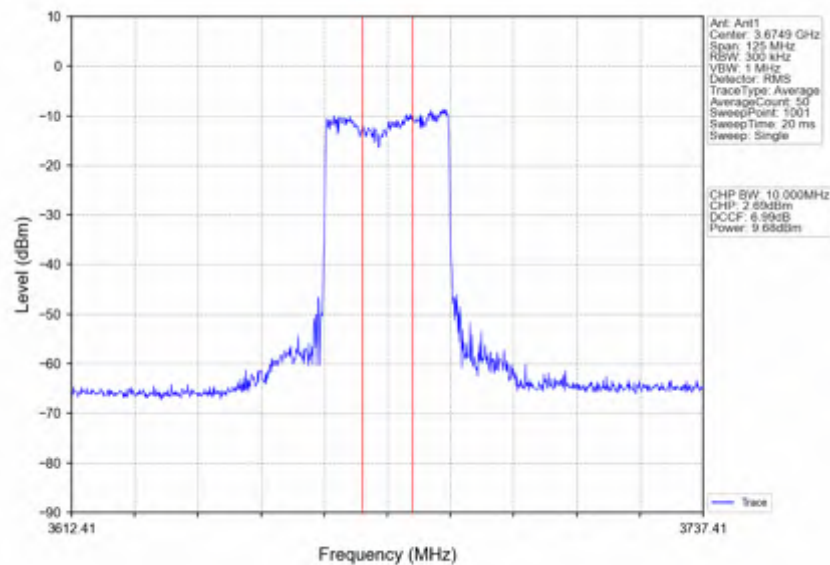
n78d_15kHz_SISO_NTNV_50MHz_DFT-s-OFDM_256_QAM_3675MHz_Inner_Full
