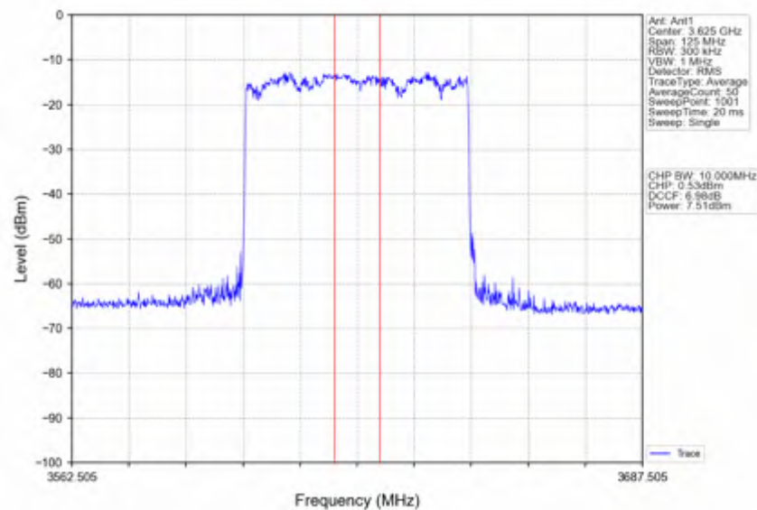
n78d_15kHz_SISO_NTNV_50MHz_DFT-s-OFDM_16_QAM_3625.005MHz_Inner_Full
