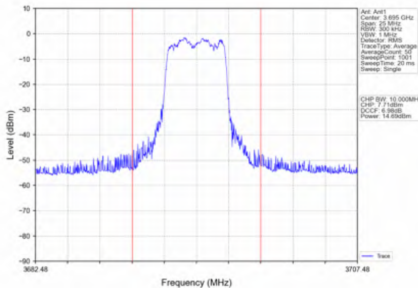
n78d_30kHz_SISO_NTNV_10MHz_CP-OFDM 64 QAM_3694.98MHz_Inner_Full
