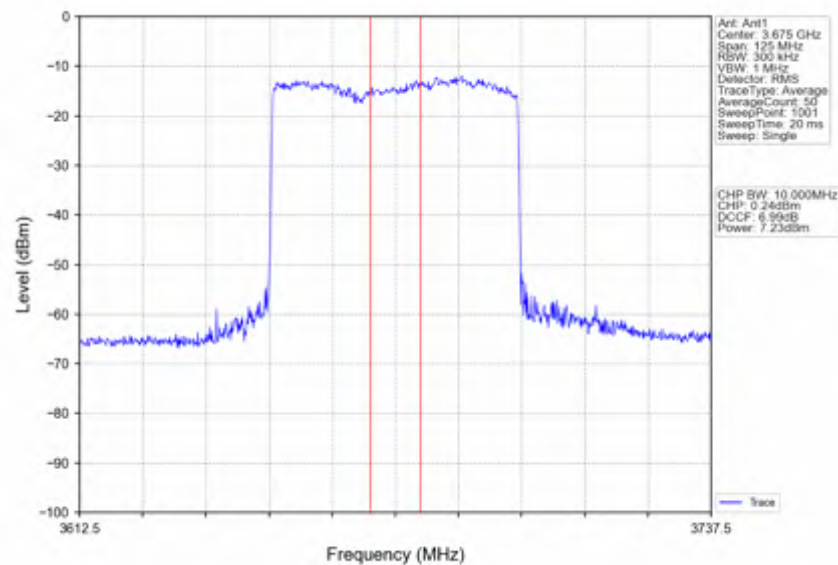
n78d_15kHz_SISO_NTNV_50MHz_CP-OFDM 16 QAM_3675MHz_Inner_Full
