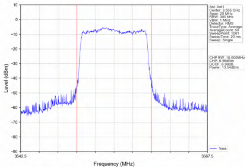
n78d_30kHz_SISO_NTNV_10MHz_CP-OFDM_256_QAM_3555MHz_Inner_Full
