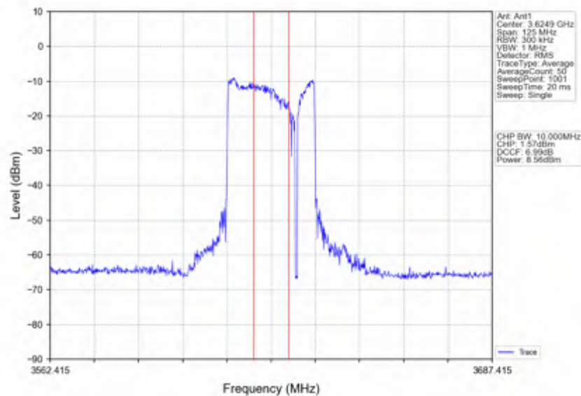
n78d_15kHz_SISO_NTNV_50MHz_DFT-s-OFDM 64 QAM_3625.005MHz_Inner_Full
