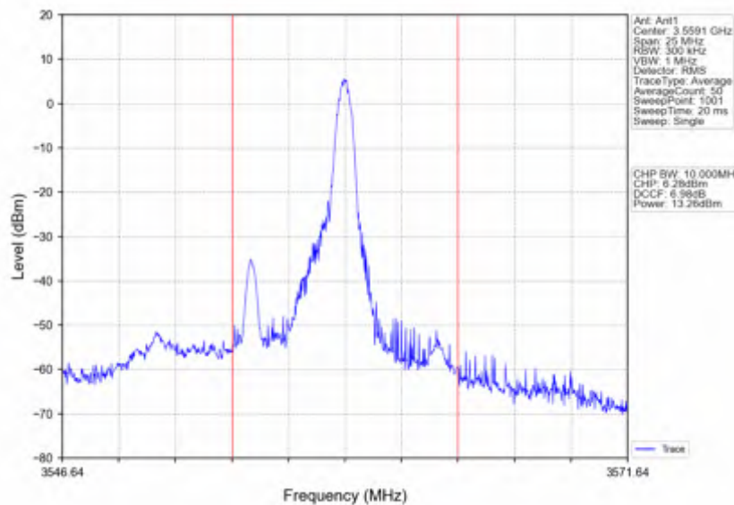
n78d_30kHz_SISO_NTNV_10MHz_CP-OFDM 256 QAM_3555MHz_Edge_1RB_Right
