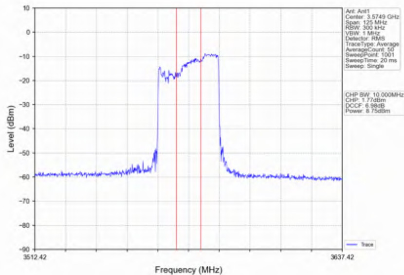
n78d_15kHz_SISO_NTNV_50MHz_CP-OFDM 256 QAM_3575.01MHz_Inner_Full
