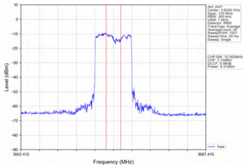
n78d_15kHz_SISO_NTNV_50MHz_DFT-s-OFDM_16_QAM_3625.005MHz_Inner_Full
