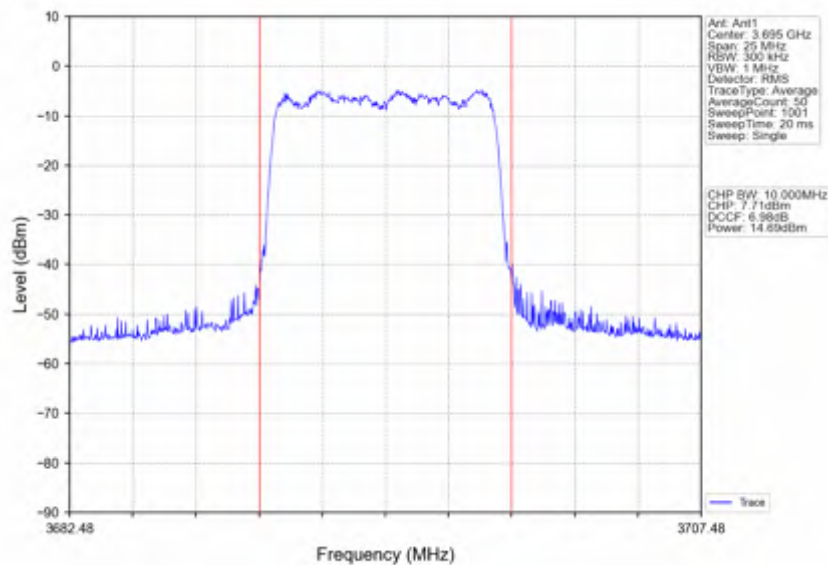
n78d_30kHz_SISO_NTNV_10MHz_CP-OFDM QPSK_3694.98MHz_Inner_Full
