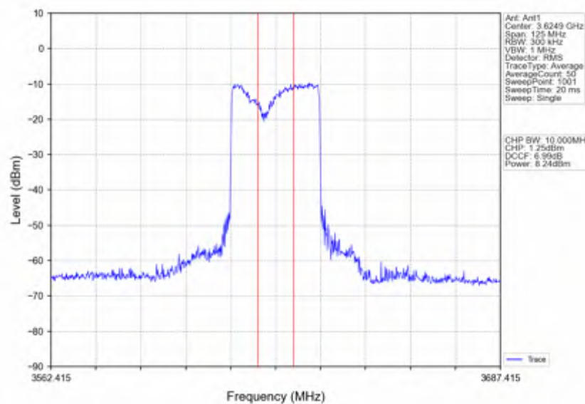
n78d 15kHz SISO NTNV 50MHz CP-OFDM 64 QAM 3625.005MHz Inner Full
