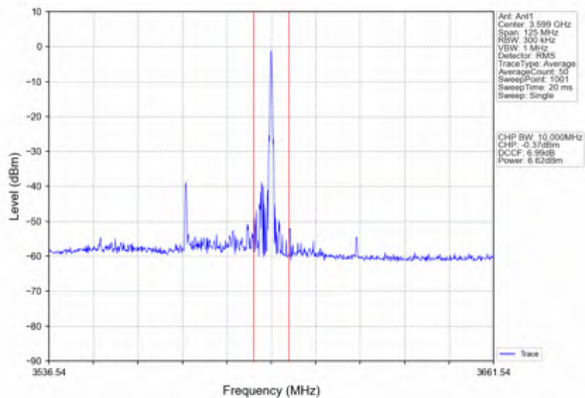
n78d_15kHz_SISO_NTNV_50MHz_CP-OFDM 256 QAM 3575.01MHz Inner_1RB_Right
