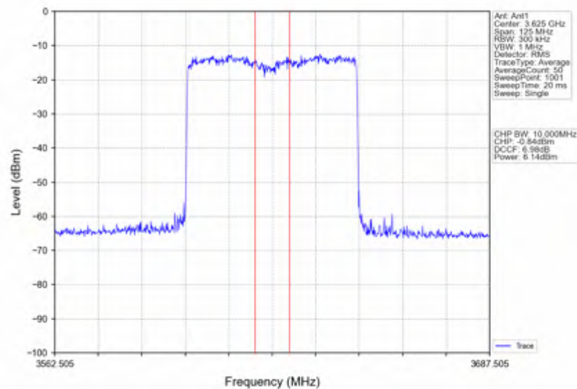
n78d_15kHz_SISO_NTNV_50MHz_DFT-s-OFDM 64 QAM_3625.005MHz_Inner_Full
