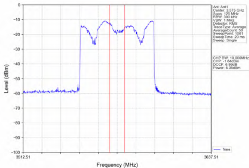
n78d_15kHz_SISO_NTNV_50MHz_CP-OFDM QPSK_3575.01MHz_Inner_Full
