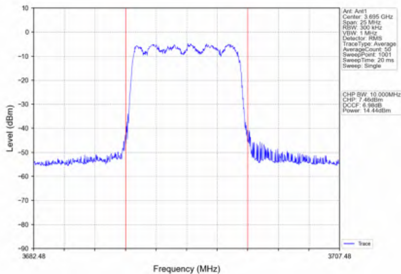
n78d_30kHz_SISO_NTNV_10MHz_DFT-s-OFDM_QPSK_3694.98MHz_Inner_Full
