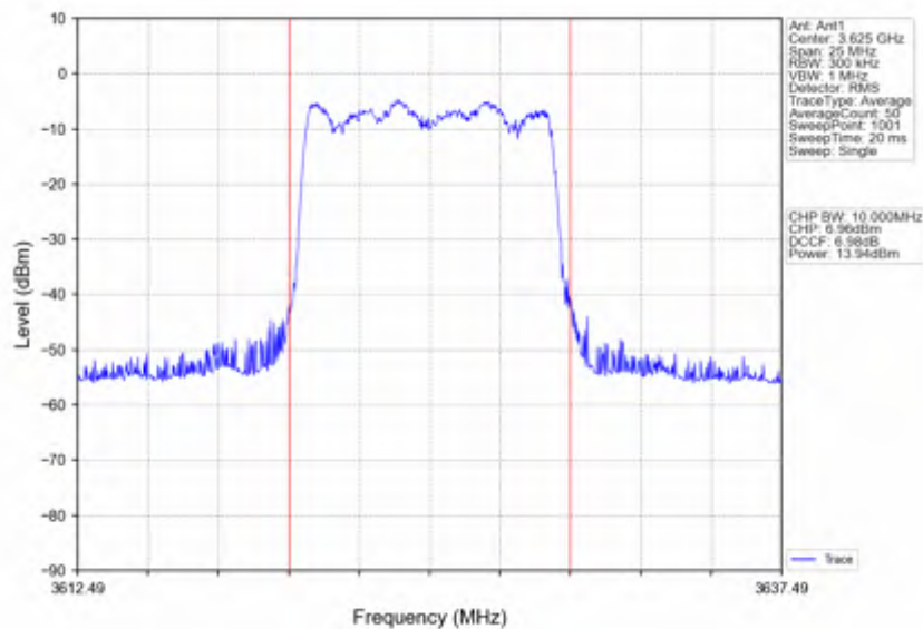
n78d_30kHz_SISO_NTNV_10MHz_CP-OFDM 64 QAM_3624.99MHz_Inner_Full
