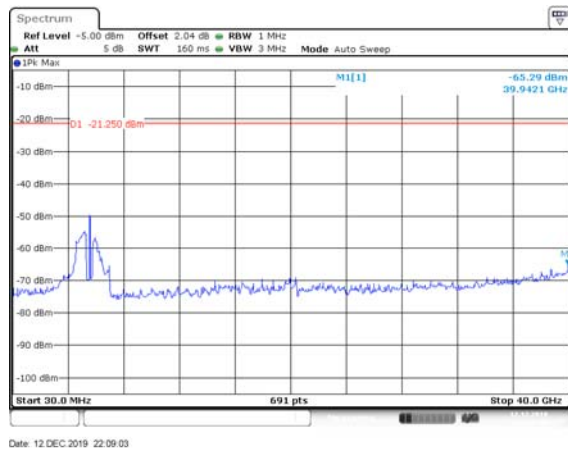
HE40, M0.1 to M11.1-BF 5710 MHz Peak
