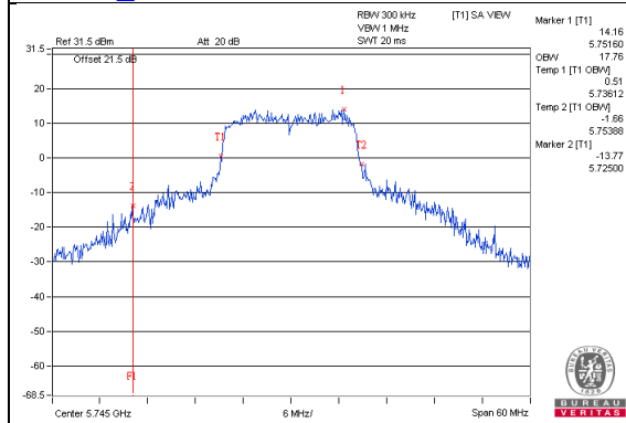
802.11ac(VHT20)_Chain0 / CH149
