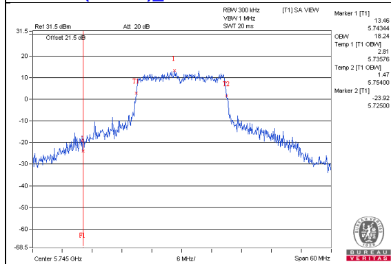
802.11ac(VHT20)_Chain2 / CH149
