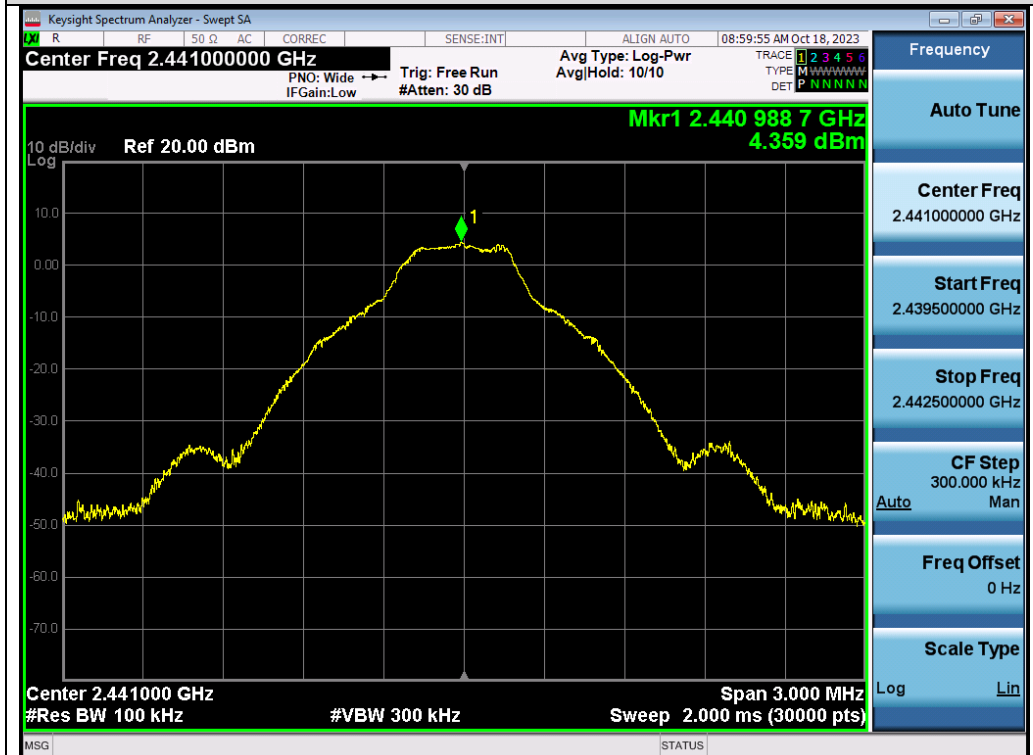
Test_Graph_BR_ANT1_2441_1Mbps_Reference Level
