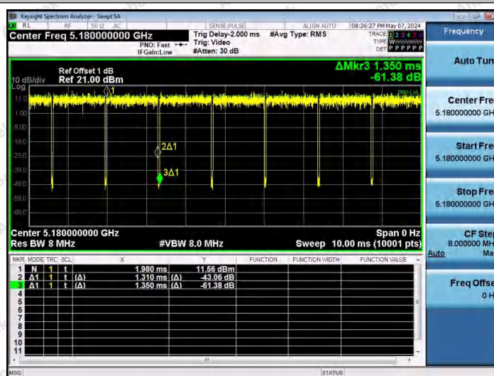
NTNV-11AC20SISO-Ant1-5180
