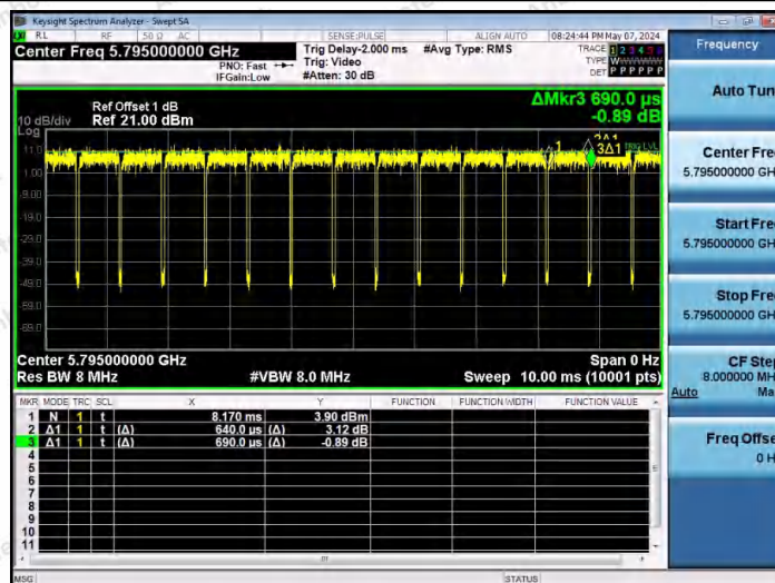
NTNV-11N40SISO-Ant1-5795
