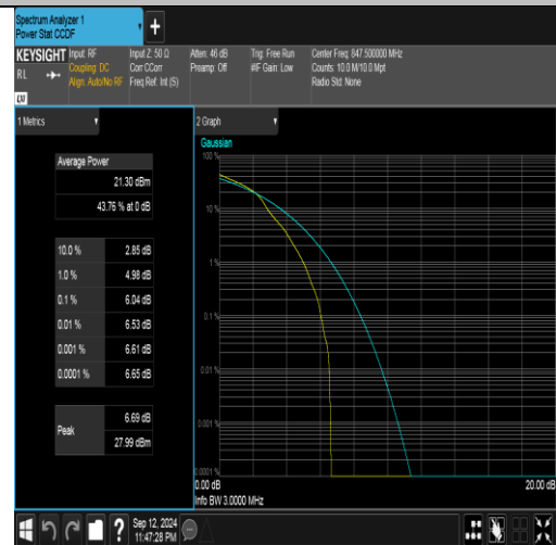
Band5-3MHz-16QAM-20635-1RB#0-PASS
