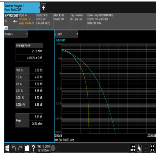
Band5-5MHz-16QAM-20425-1RB#0-PASS
