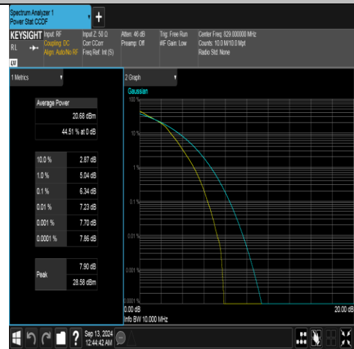
Band5-10MHz-16QAM-20450-50RB#0-PASS
