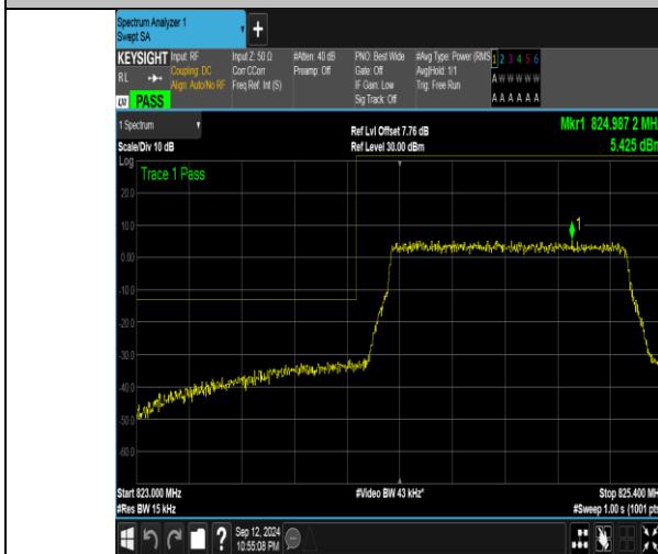
Band5_1.4MHz_QPSK_20407_6RB#0
