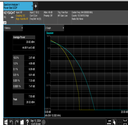
Band5-10MHz-16QAM-20600-50RB#0-PASS
