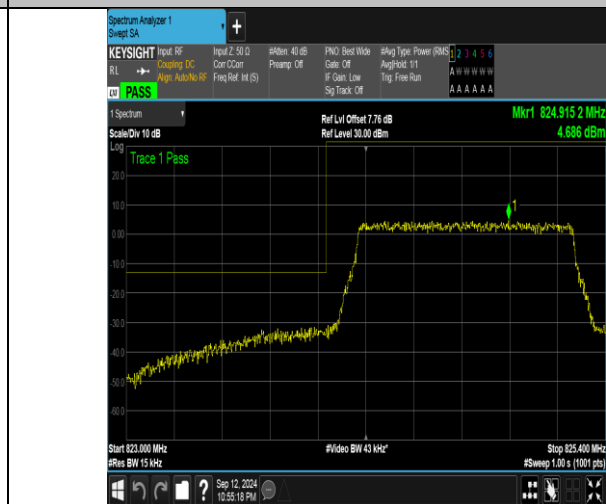
Band5_1.4MHz_16QAM_20407_6RB#0
