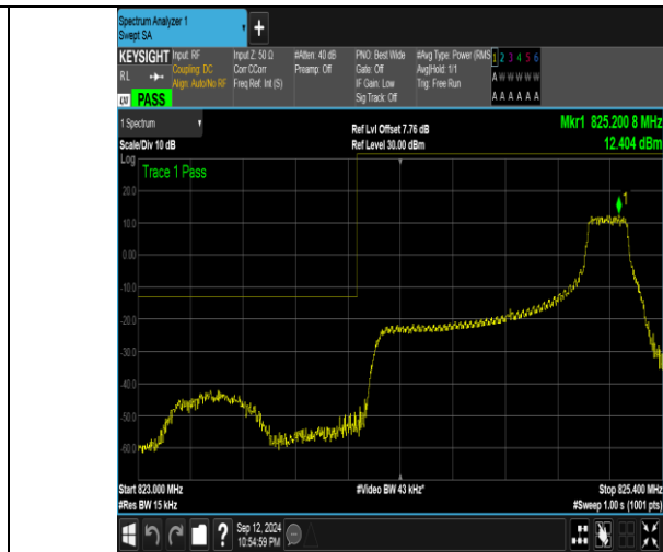
Band5_1.4MHz_16QAM_20407_1RB#5
