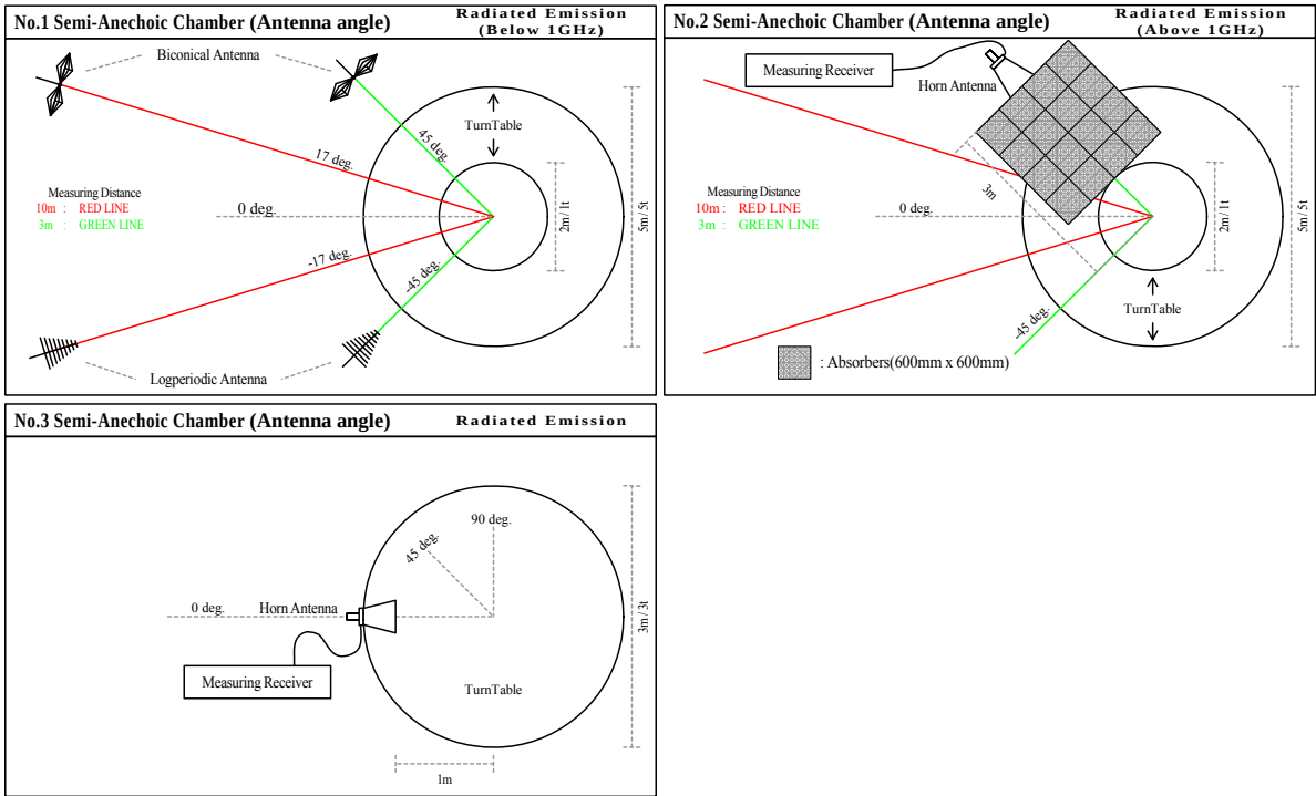
Figure 1. Antenna angle
