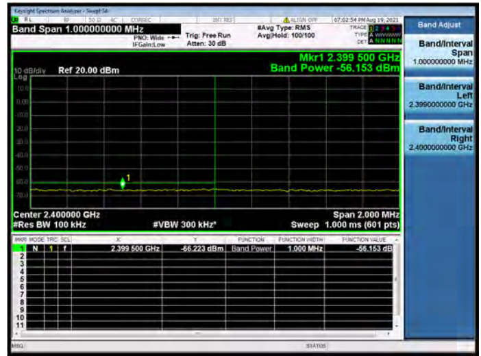
802.11b CHANNEL 5, Reference level
