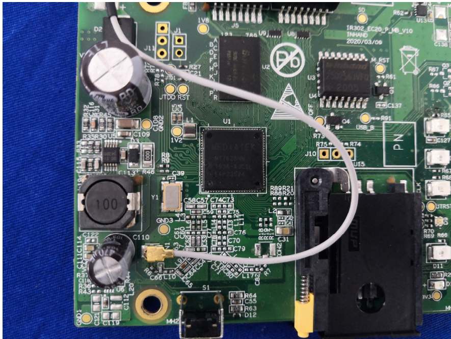
2.4G WiFi Chip View
