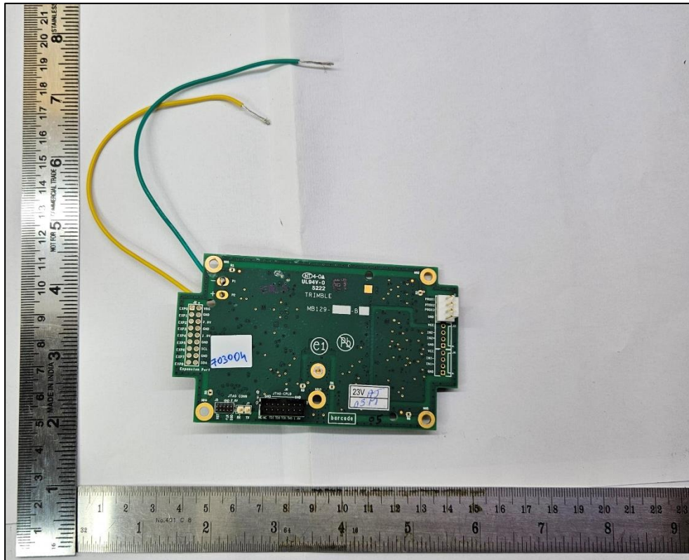
PCB dimensional View
