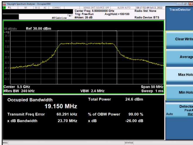
Plot 7-7. 26dB BW & 99% OBW (20MHz BW 202.11n – Ch. 100, MCS0)
