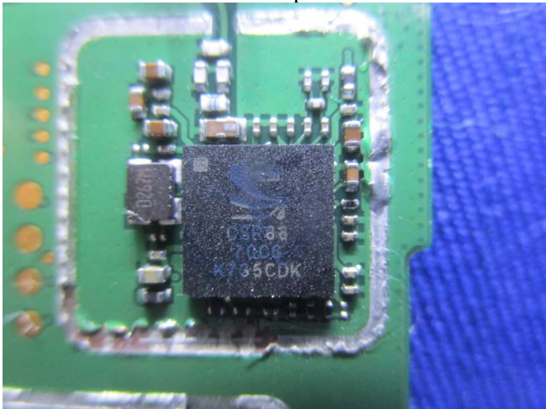
BT Chip
