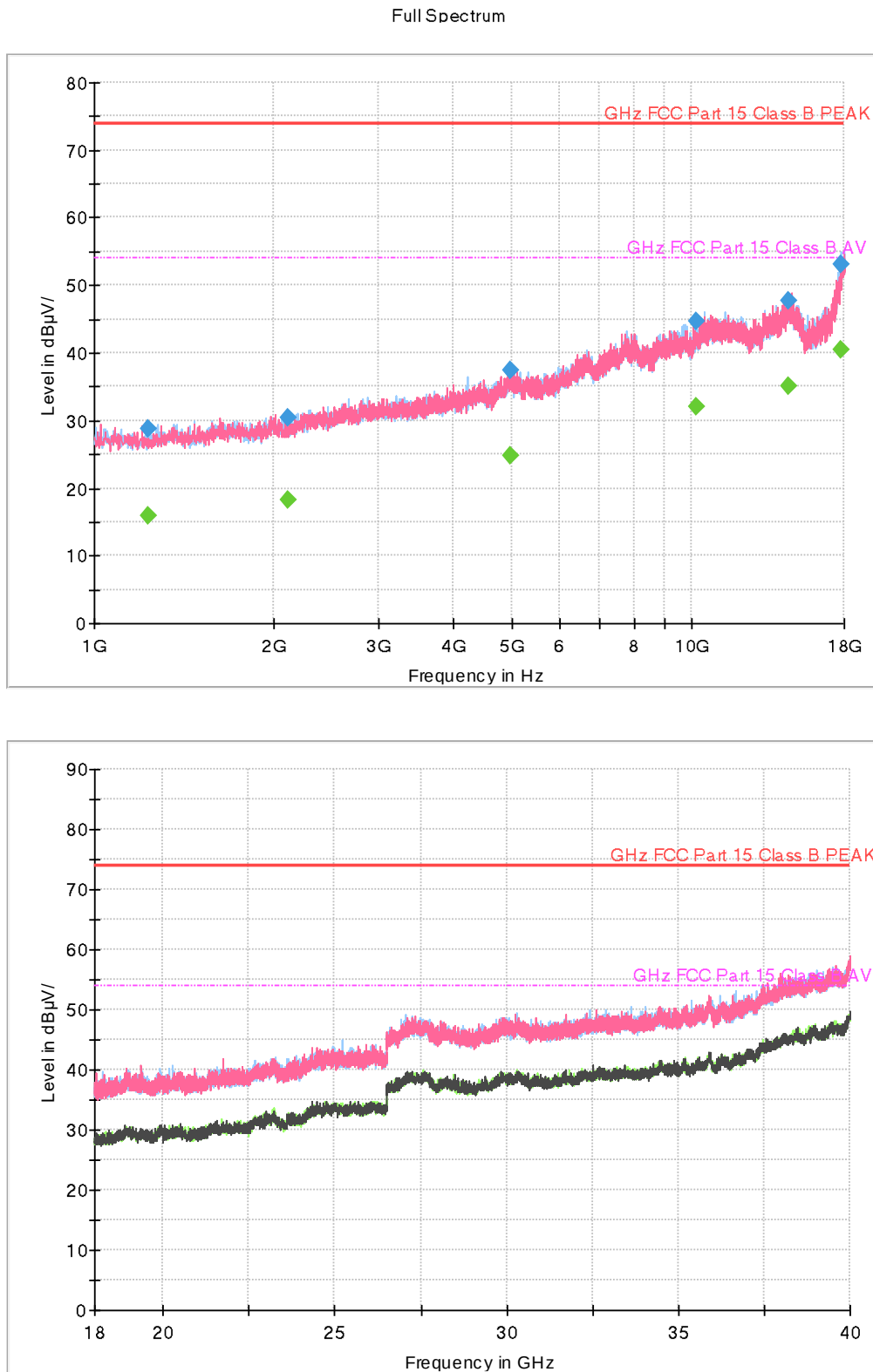
Figure 6: [EUT+ Earphone] LTE B5+5G NR n5 Low ch Idle
