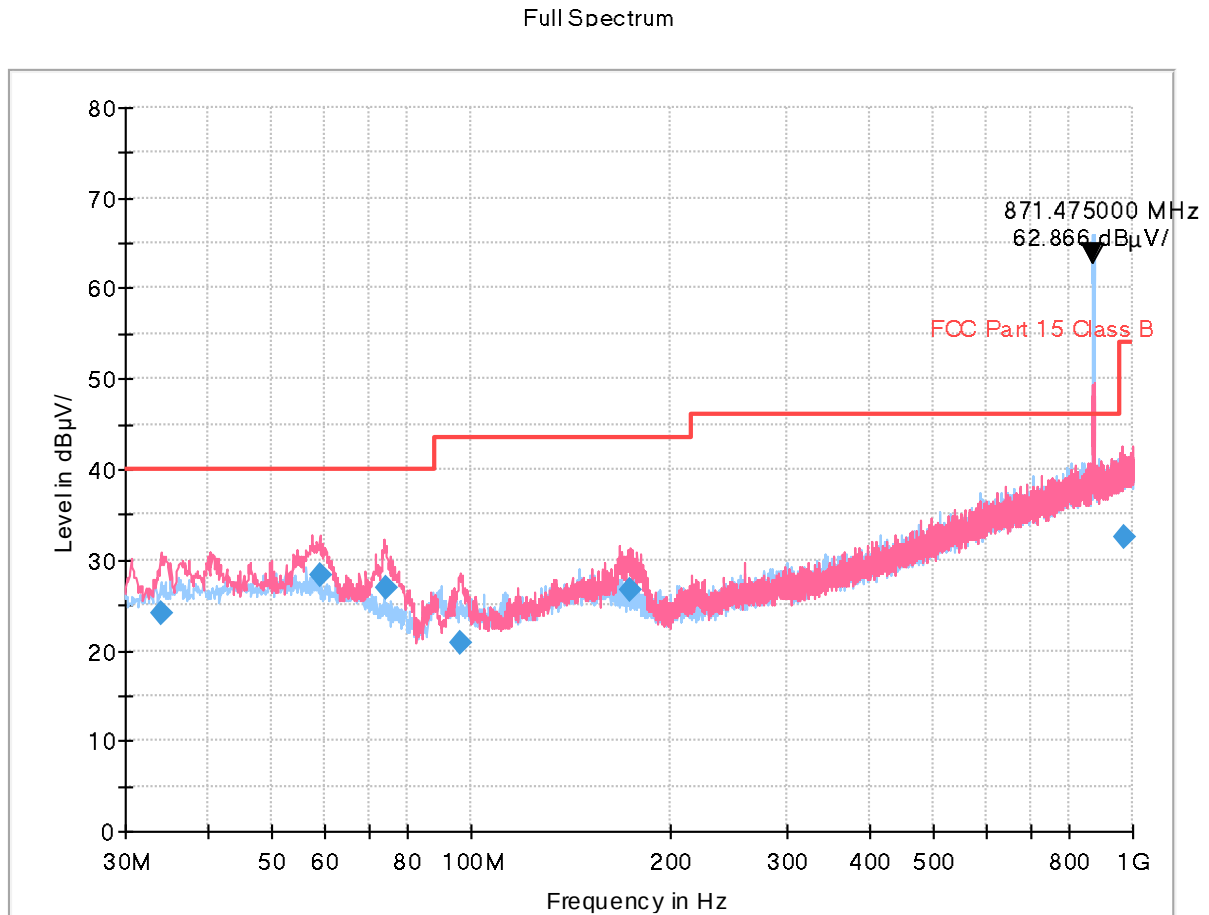
Figure 1: [EUT+TA] LTE B5+5G NR n5 Low ch Idle
