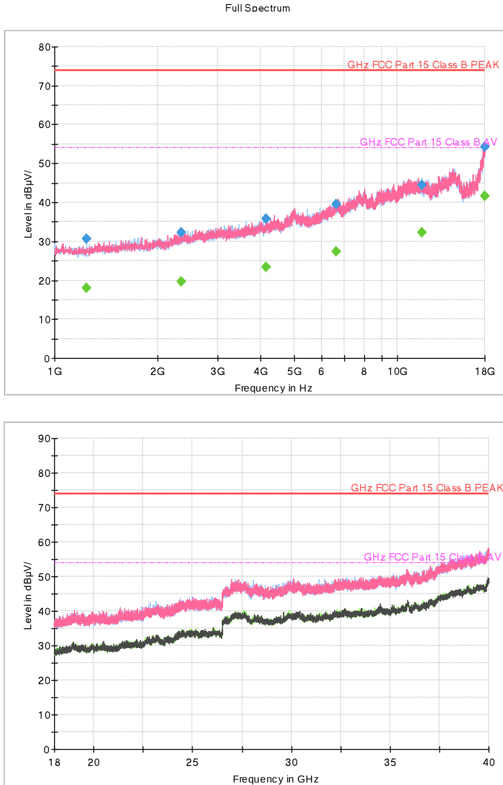
Figure 5: [EUT+TA] LTE B5+5G NR n5 Low ch Idle
