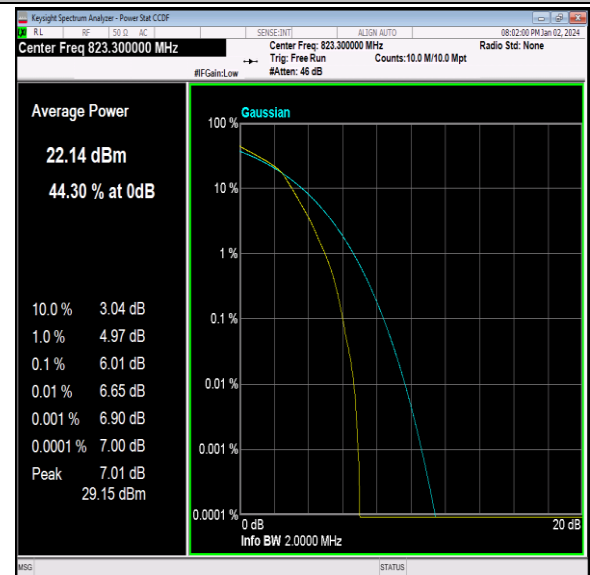
26(814-824)-1.4MHz-16QAM-26783-6RB#0-PASS
