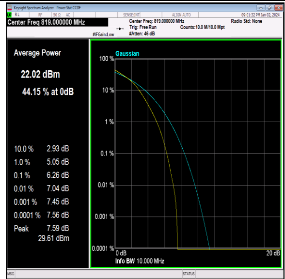
26(814-824)-10MHz-16QAM-26740-50RB#0-PASS
