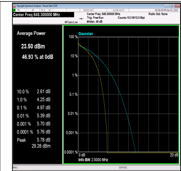
26(824-849)-1.4MHz-QPSK-27033-6RB#0-PASS
