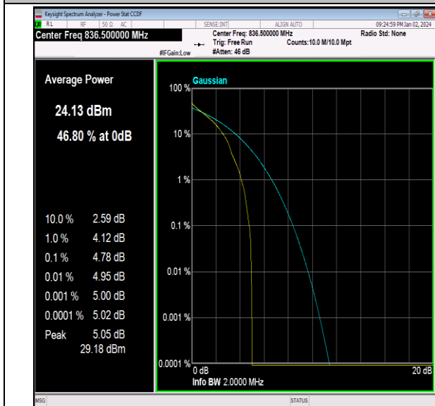
26(824-849)-1.4MHz-QPSK-26915-1RB#0-PASS
