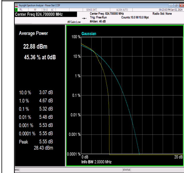
26(824-849)-1.4MHz-16QAM-26797-1RB#0-PASS
