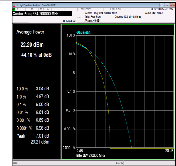
26(824-849)-1.4MHz-16QAM-26797-6RB#0-PASS
