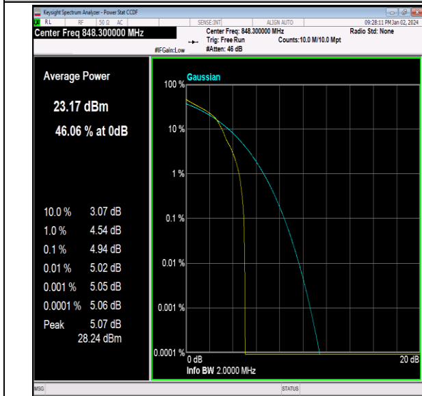
26(824-849)-1.4MHz-16QAM-27033-1RB#0-PASS
