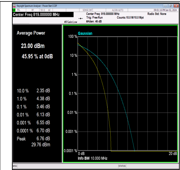
26(814-824)-10MHz-QPSK-26740-50RB#0-PASS
