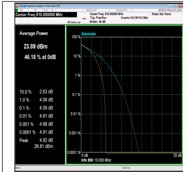
26(814-824)-10MHz-QPSK-26740-1RB#0-PASS
