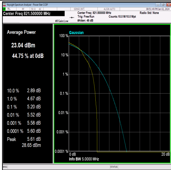
26(814-824)-5MHz-16QAM-26765-1RB#0-PASS
