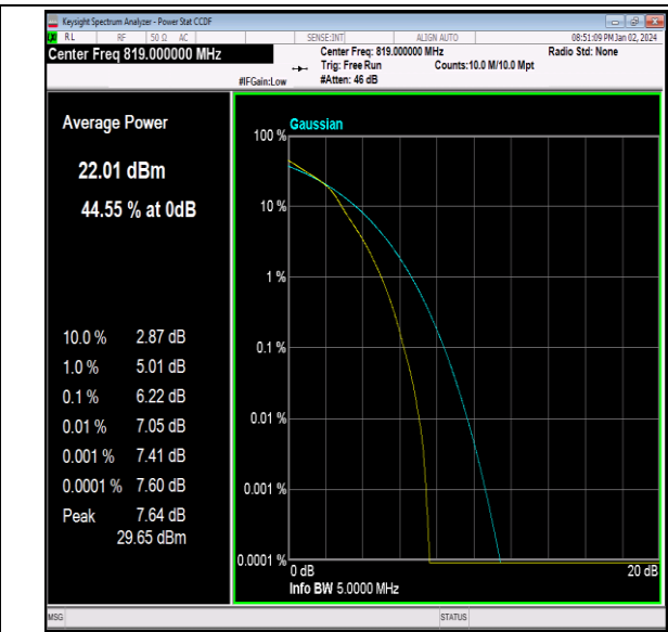
26(814-824)-5MHz-16QAM-26740-25RB#0-PASS
