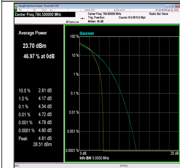
Band13-5MHz-16QAM-23255-1RB#0-PASS
