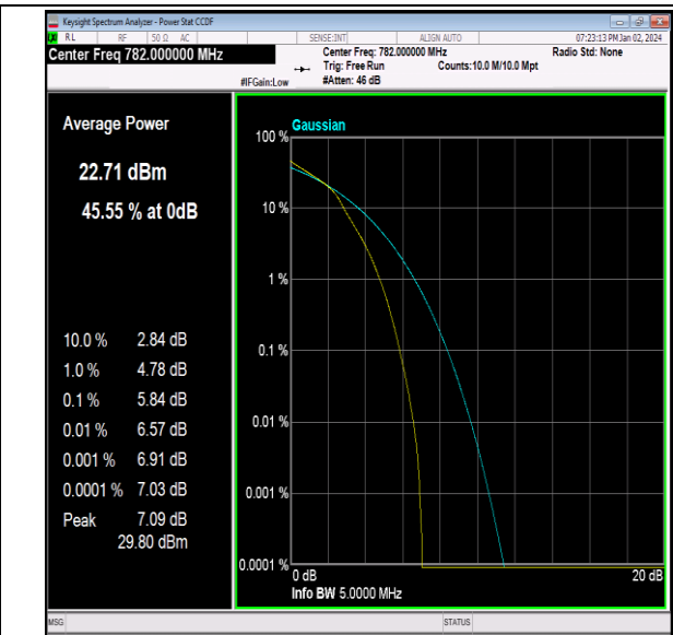
Band13-5MHz-16QAM-23230-25RB#0-PASS
