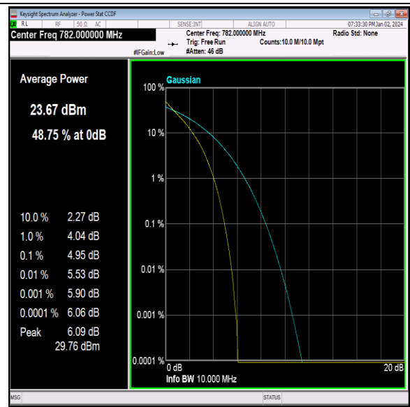
Band13-10MHz-QPSK-23230-50RB#0-PASS
