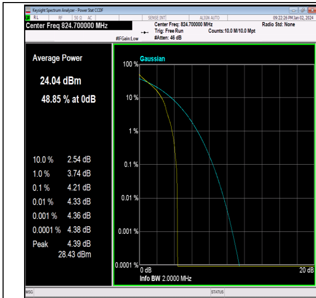
26(824-849)-1.4MHz-QPSK-26797-1RB#0-PASS
