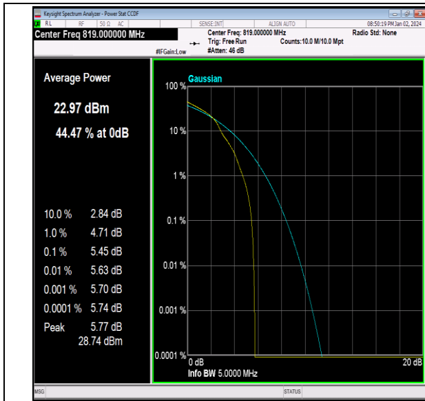
26(814-824)-5MHz-16QAM-26740-1RB#0-PASS
