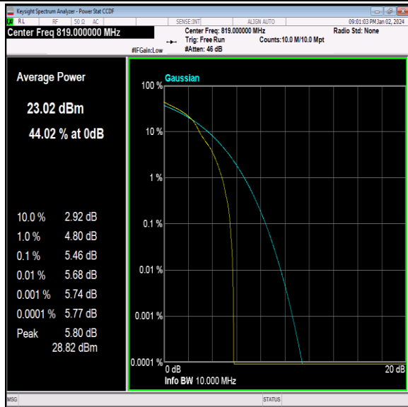
26(814-824)-10MHz-16QAM-26740-1RB#0-PASS
