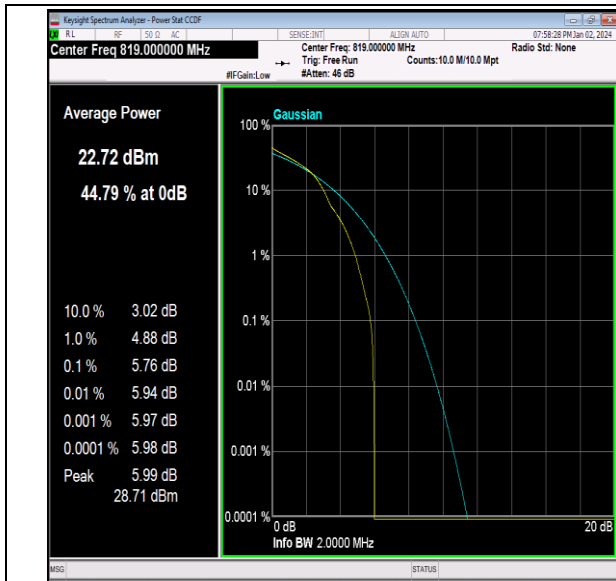
26(814-824)-1.4MHz-16QAM-26740-1RB#0-PASS
