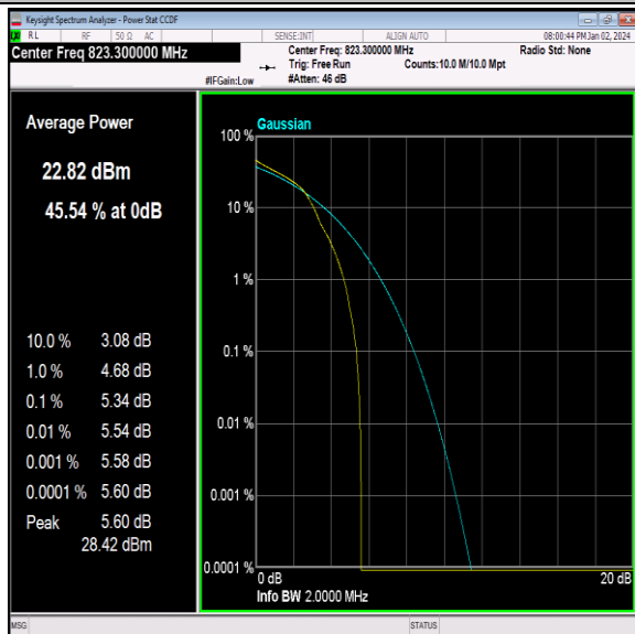
26(814-824)-1.4MHz-16QAM-26783-1RB#0-PASS
