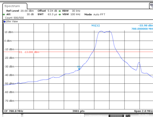
Band14-5MHz-QPSK-23305-1-0-Low--33.98-PASS
