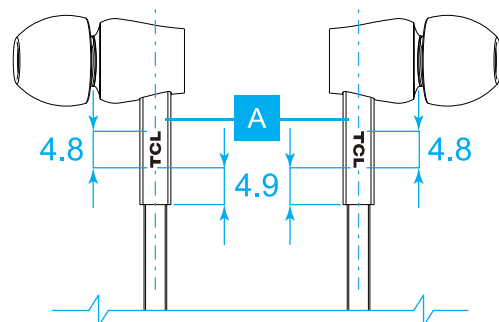
LHS earpiece outer surfaces
