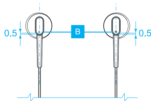
LHS earpiece inner surfaces
