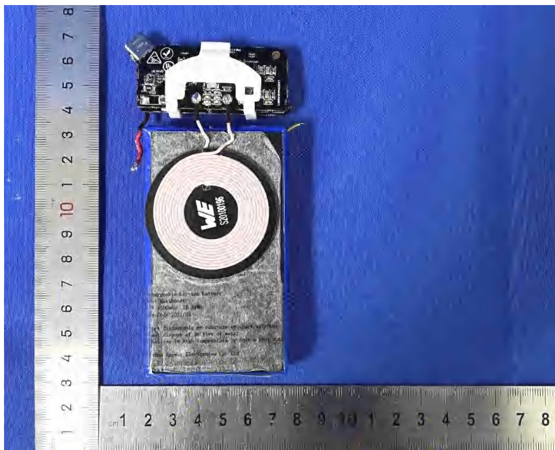
Figure 4 Internal electronics unit view with cover removed -1
