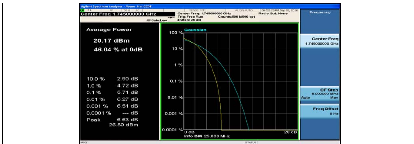
(Channel Bandwidth:20 MHz)_HCH_16QAM_50RB#0
