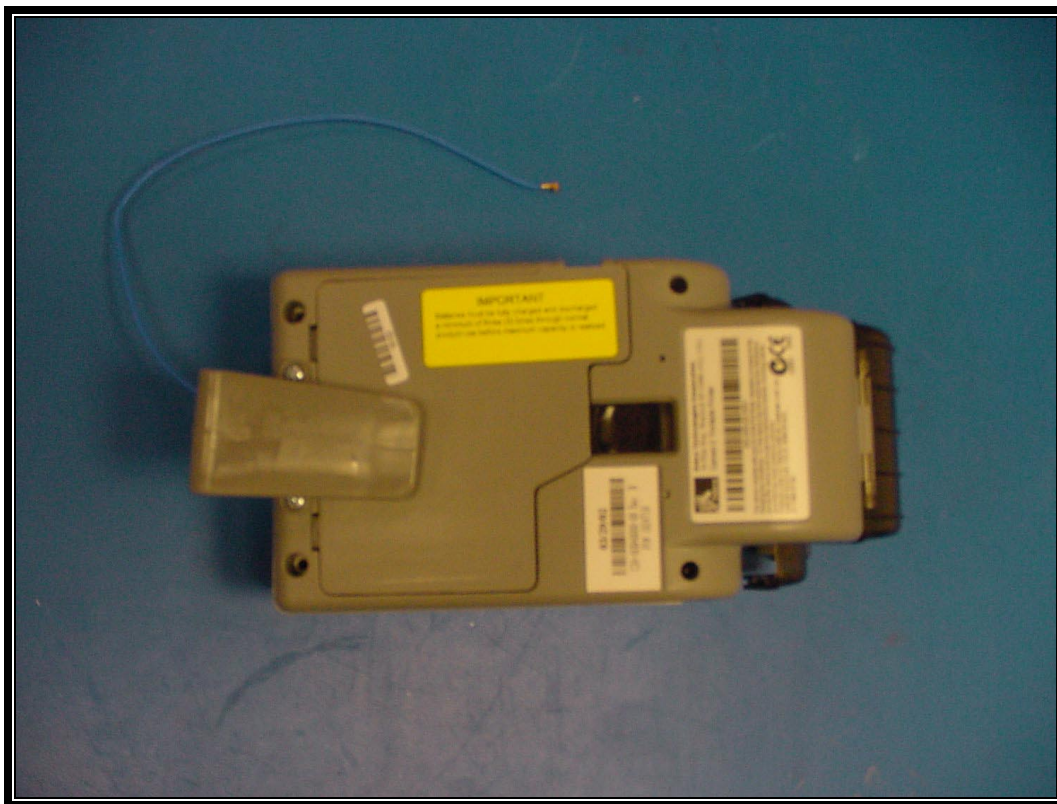
PHOTOGRAPH 19: REAR VIEW CAMEO 2 ANTENNA INSTALLED IN TYPICAL HOST
