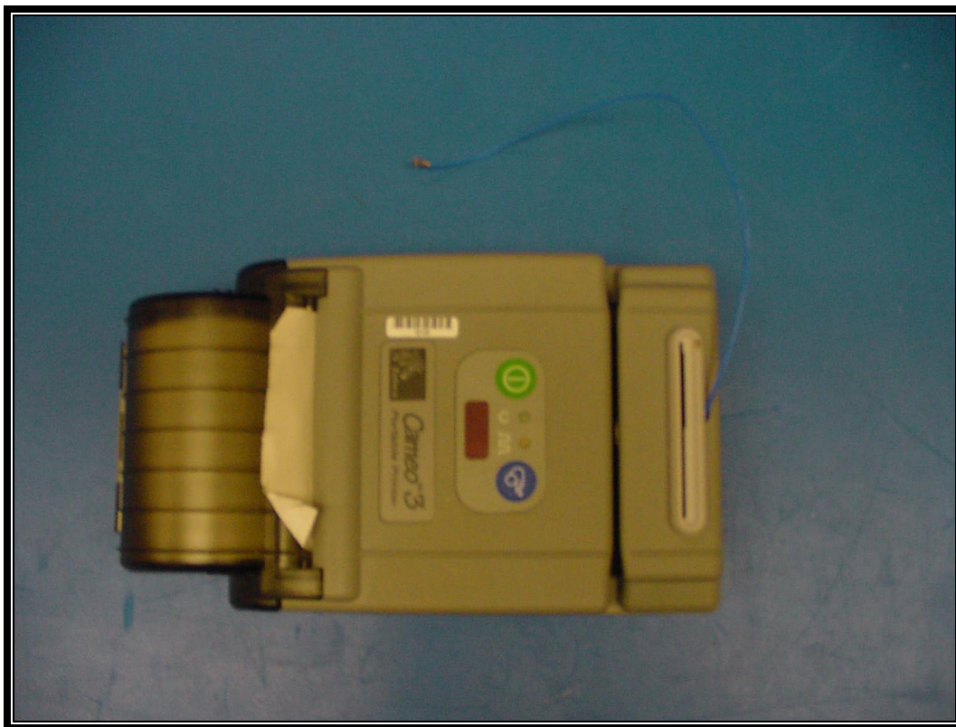
PHOTOGRAPH 16: TOP VIEW CAMEO 3 ANTENNA INSTALLED IN TYPICAL HOST
