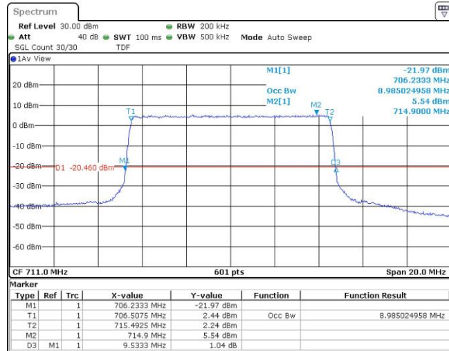
Band12-10MHz-16QAM-23060-25RB#0
