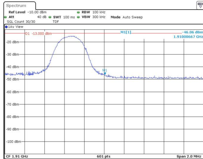
Band2-5MHz-16QAM-19175-1RB#24
