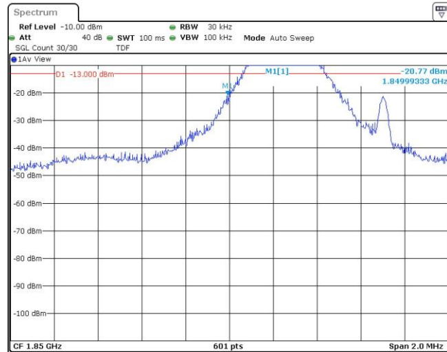
Band2-1.4MHz-16QAM-18607-1RB#5
