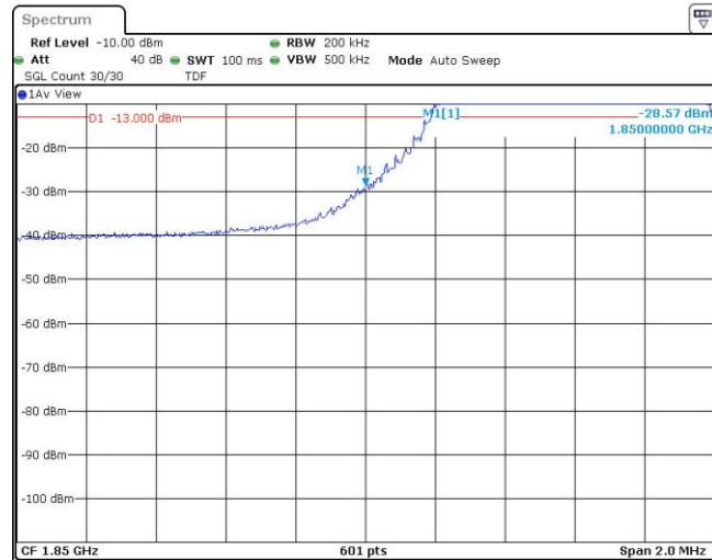
Band2-10MHz-QPSK-18650-1RB#49
