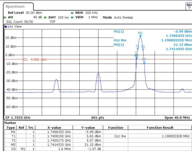
Band4-20MHz-16QAM-20175-1RB#99
