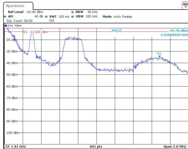
Band2-1.4MHz-16QAM-19193-1RB#5
