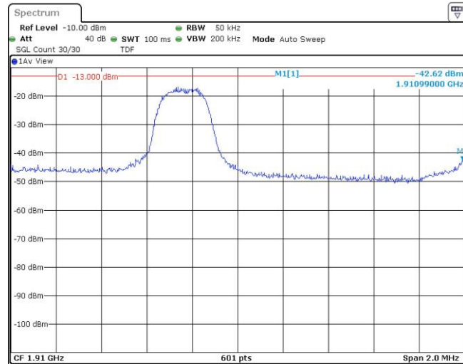
Band2-3MHz-16QAM-19185-1RB#14
