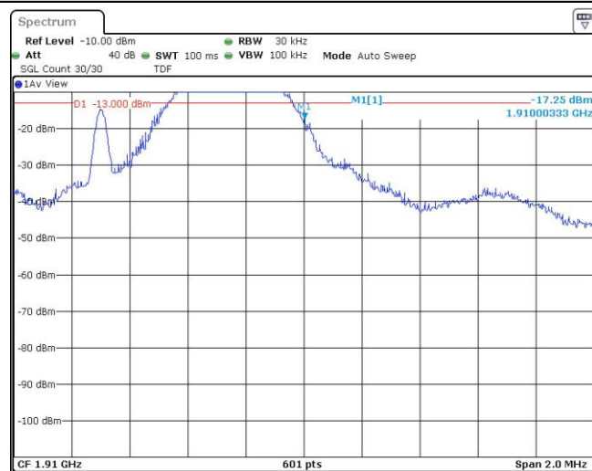
Band2-1.4MHz-QPSK-19193-6RB#0
