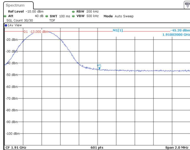
Band2-10MHz-QPSK-19150-1RB#49
