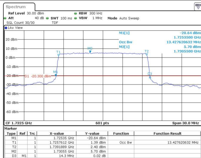
Band4-15MHz-16QAM-20175-38RB#0
