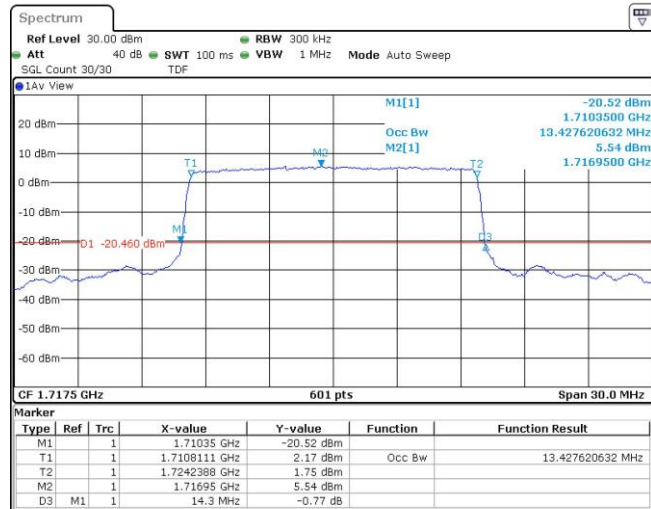
Band4-15MHz-16QAM-20175-38RB#0
