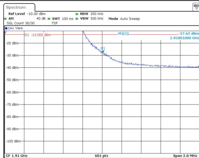
Band2-10MHz-QPSK-19150-25RB#0
