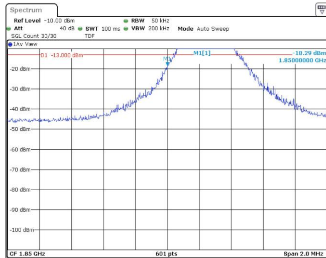
Band2-3MHz-16QAM-18615-1RB#14
