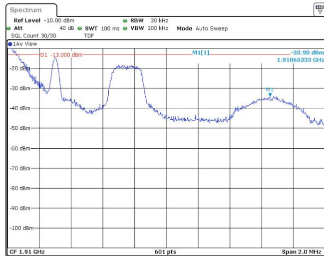
Band2-1.4MHz-QPSK-19193-1RB#5
