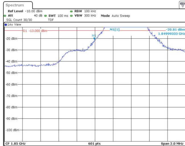
Band2-5MHz-16QAM-18625-1RB#24
