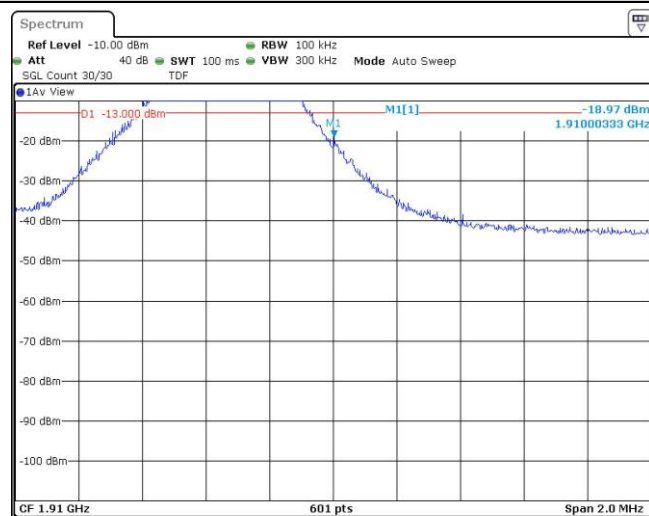
Band2-5MHz-16QAM-19175-25RB#0
