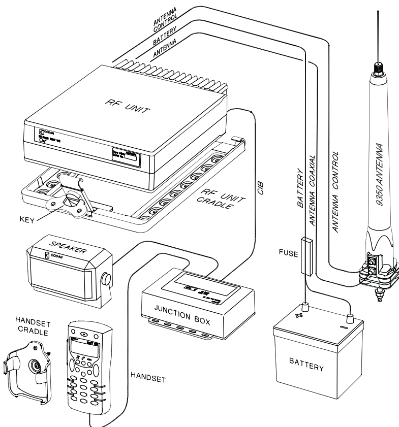
Figure 1: Typical NGT ASR mobile station
