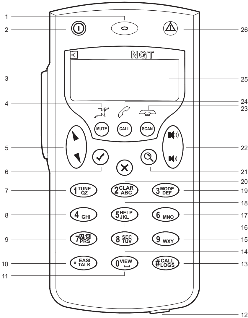
Figure 3: The handset
