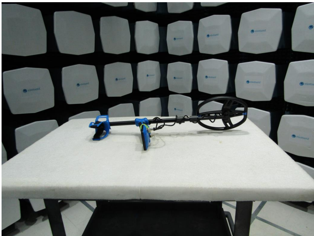
EUT on Side
