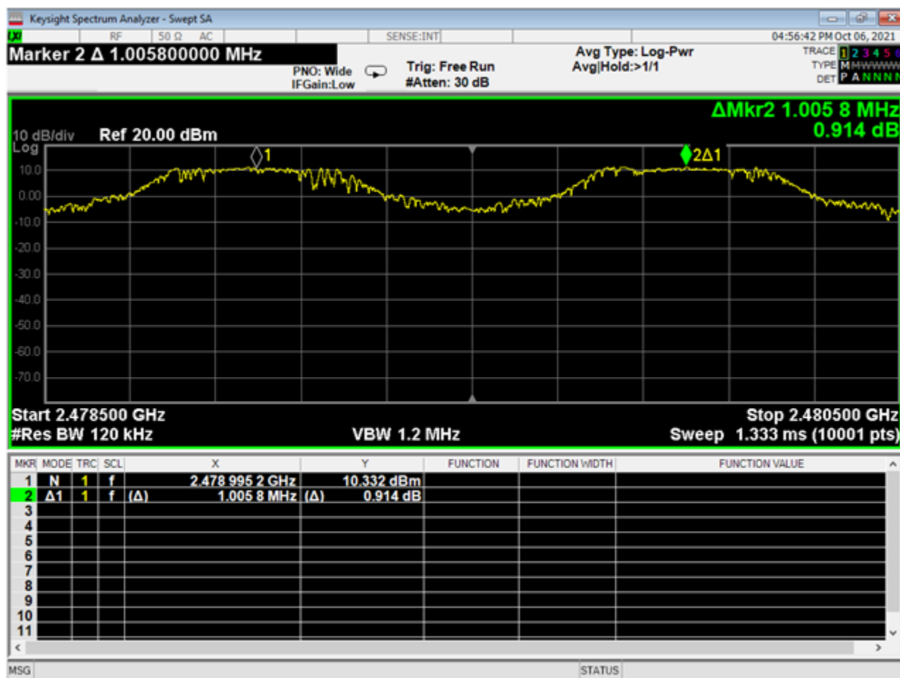
15 Frequency Separation.png
