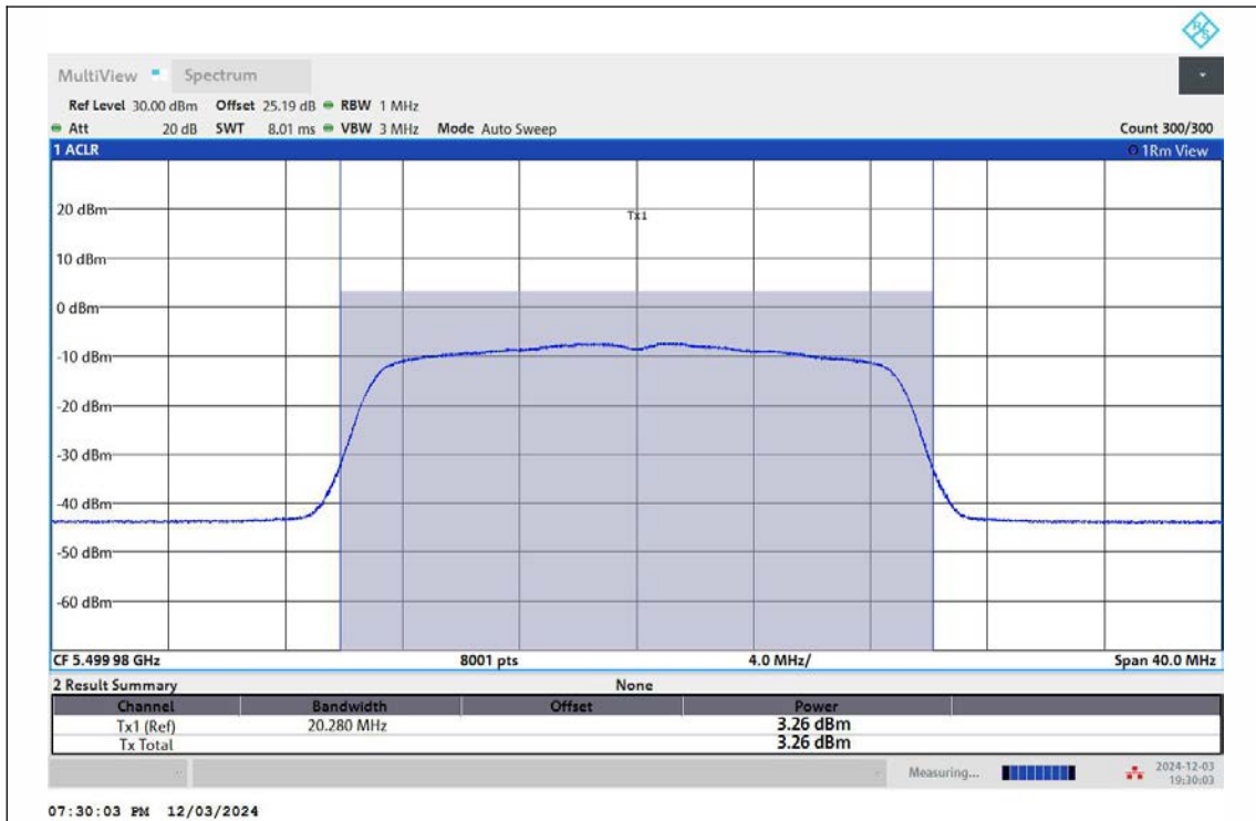
11N20MIMO-Ant1-5500-TPC_L-PASS
