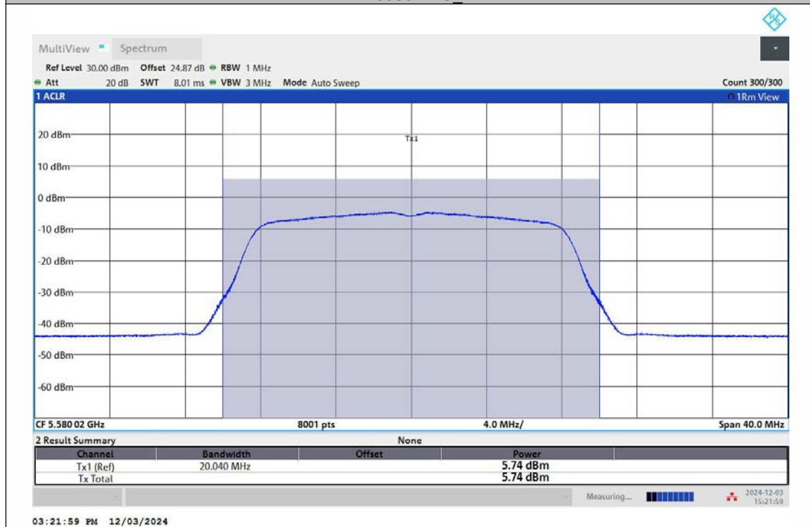
11A-Ant1-5580-TPC_L-PASS
