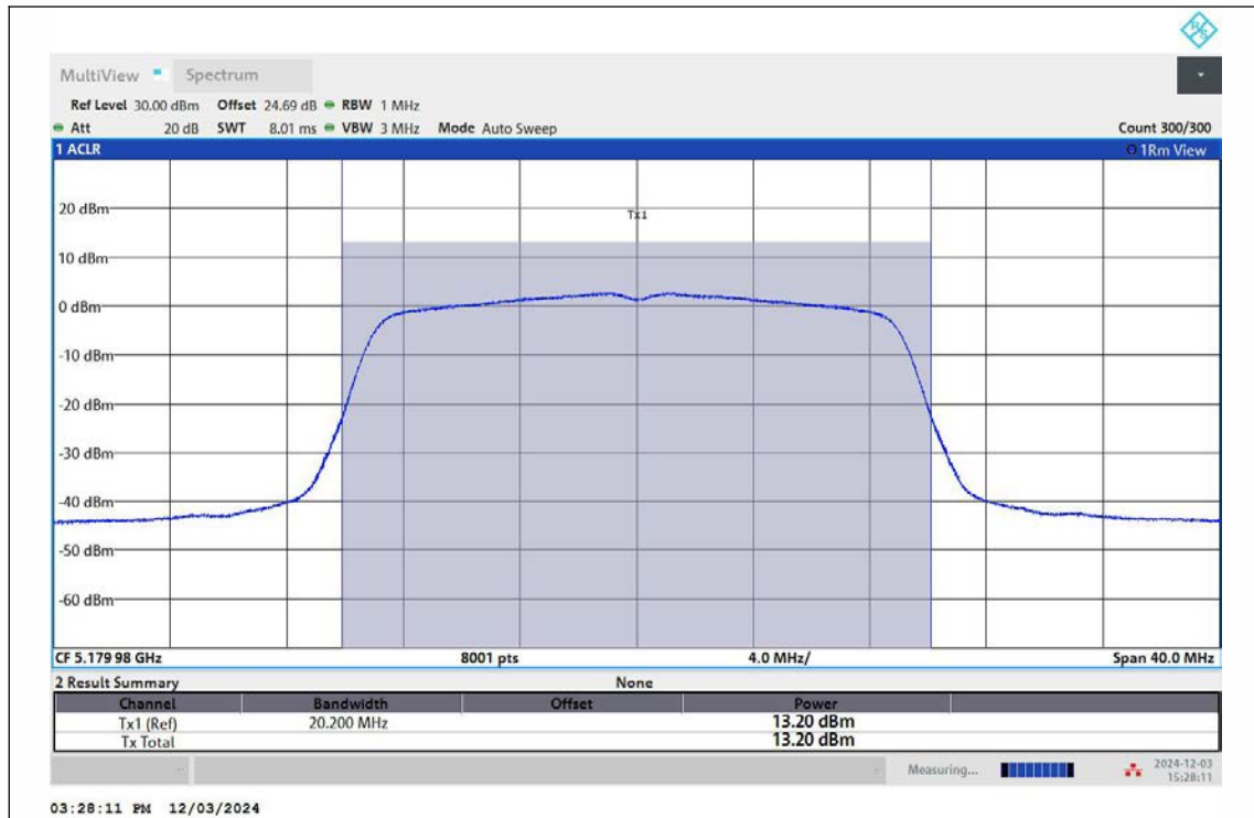
11N20MIMO-Ant1-5180-PASS
