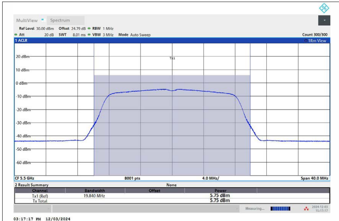
11A-Ant2-5500-TPC_L-PASS
