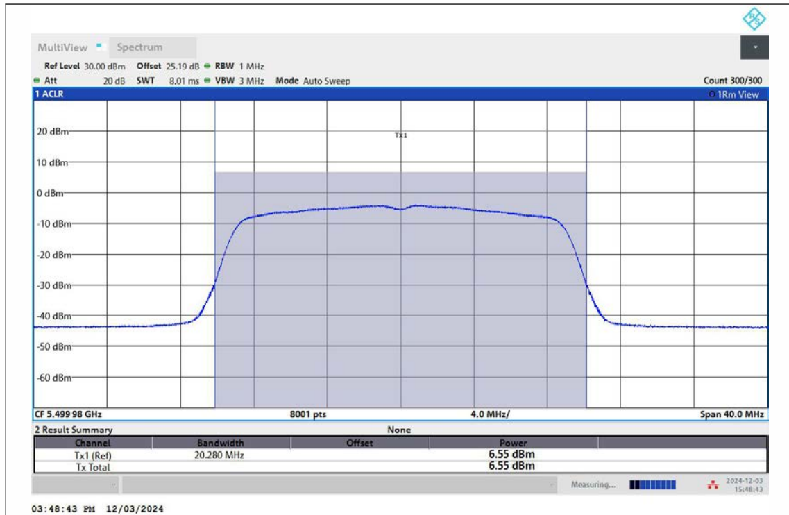
11N20MIMO-Ant1-5500-TPC_H-PASS
