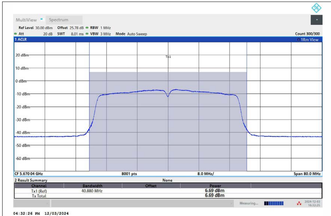
11N40MIMO-Ant1-5670-TPC_H-PASS
