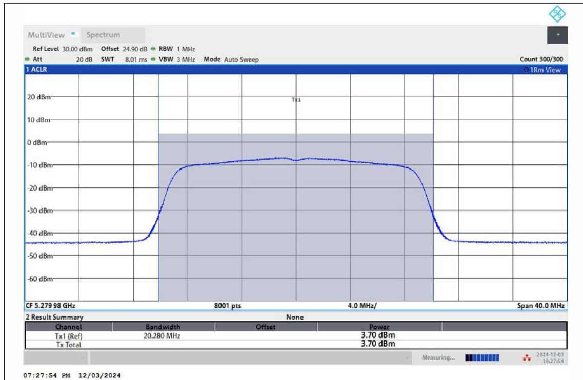
11N20MIMO-Ant1-5280-TPC_L-PASS
