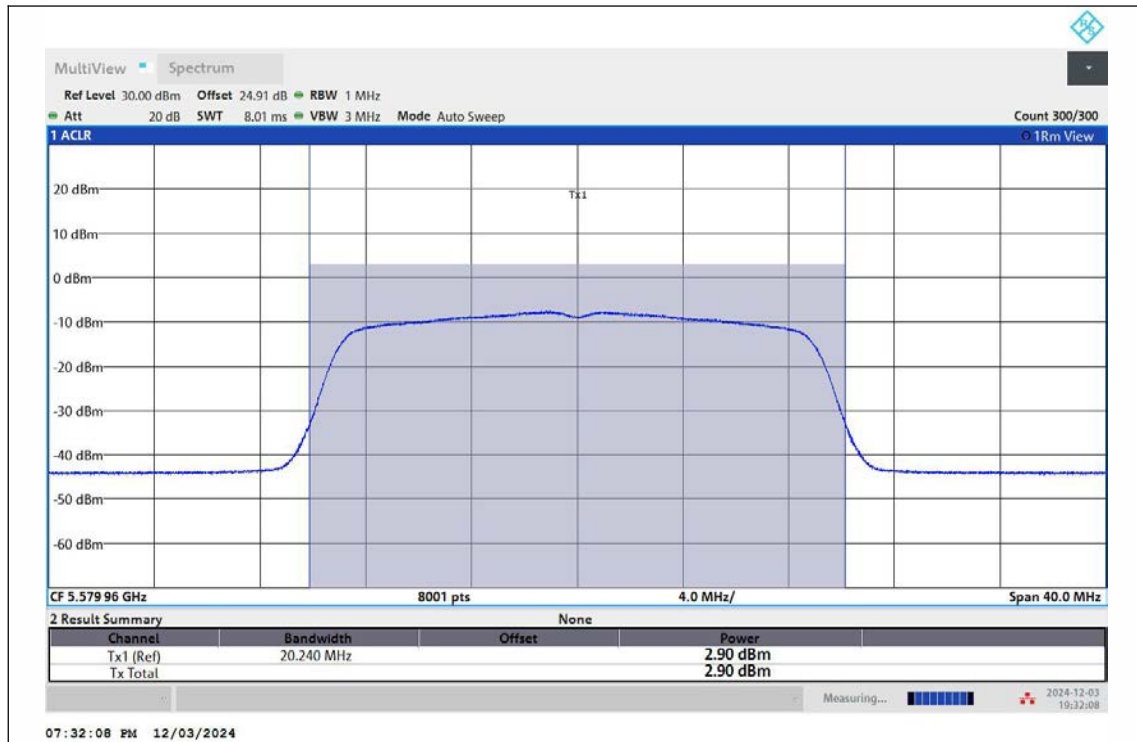
11N20MIMO-Ant1-5580-TPC_L-PASS
