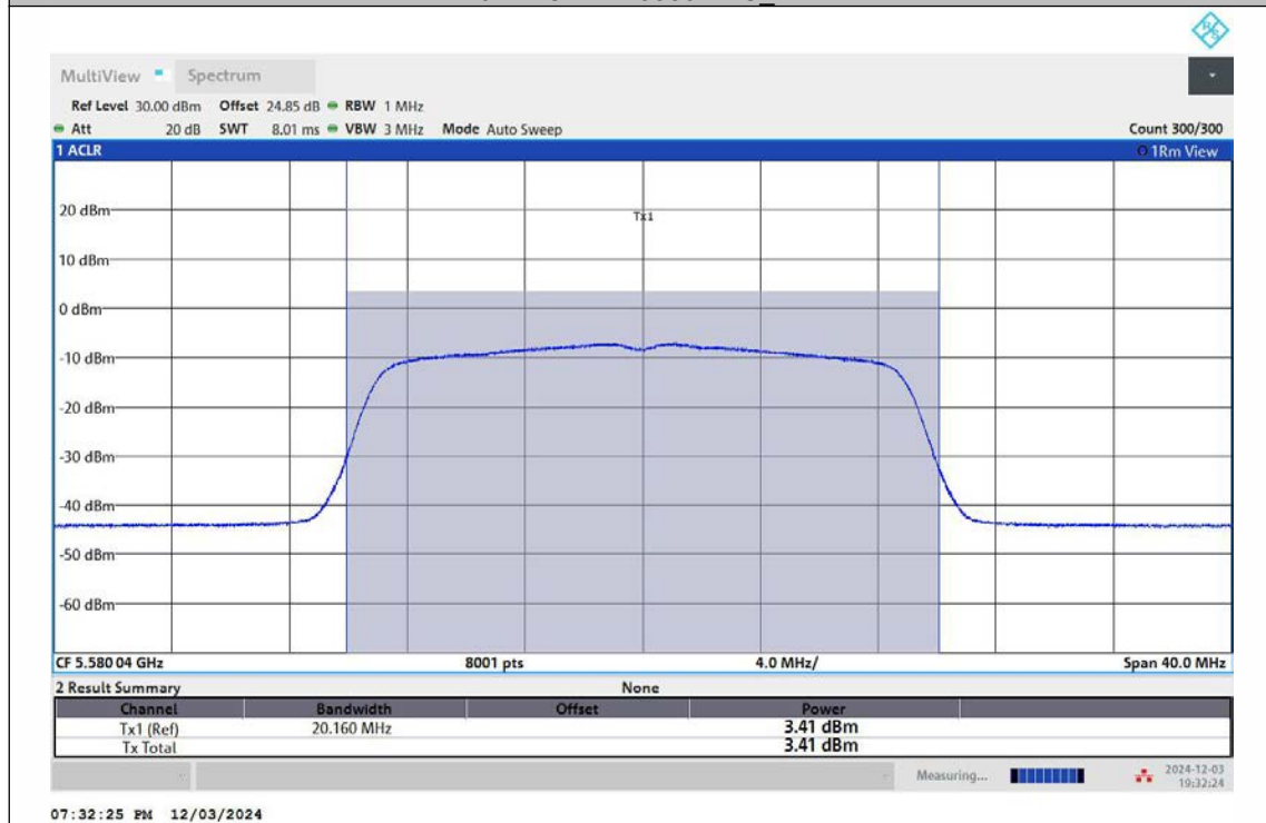
11N20MIMO-Ant2-5580-TPC_L-PASS
