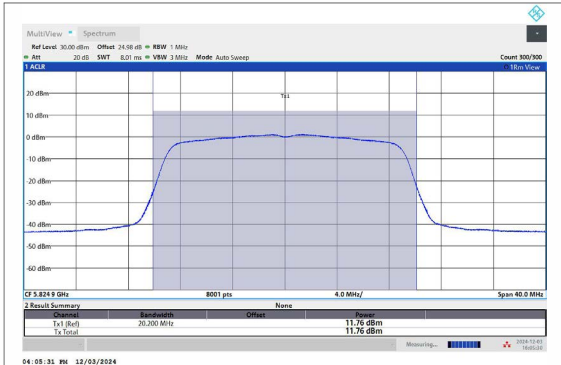
11N20MIMO-Ant1-5825-PASS
