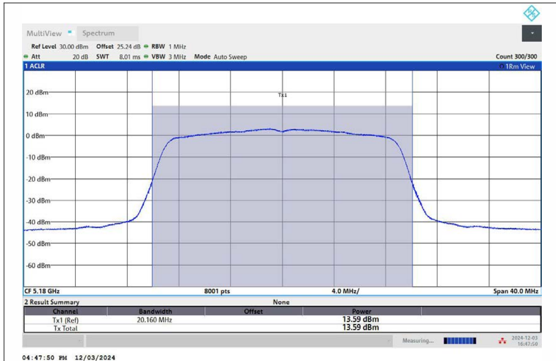
11AC20MIMO-Ant1-5180-PASS
