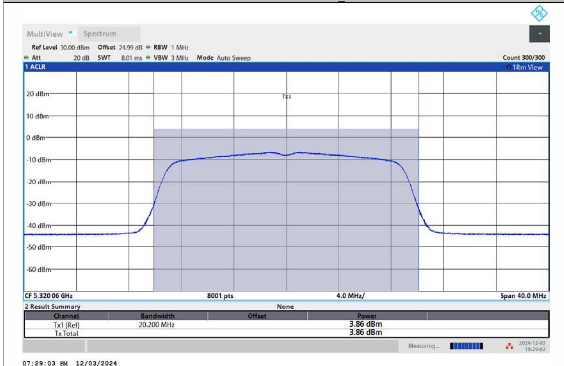
11N20MIMO-Ant2-5320-TPC_L-PASS
