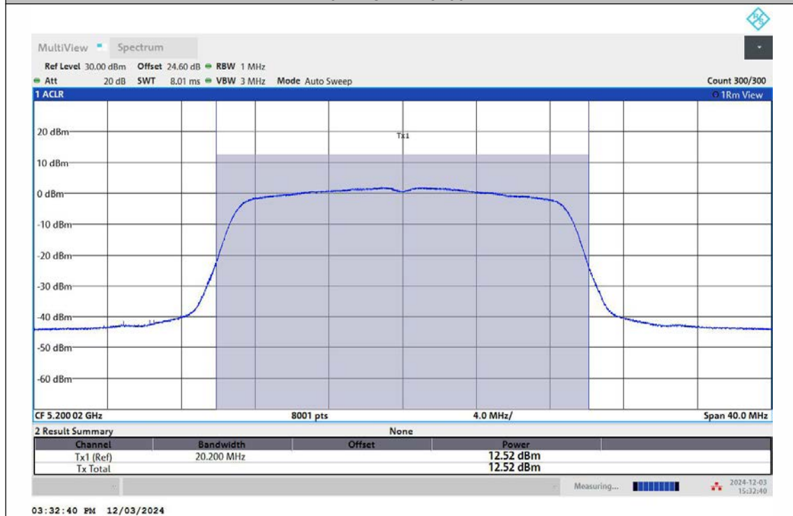
11N20MIMO-Ant2-5200-PASS
