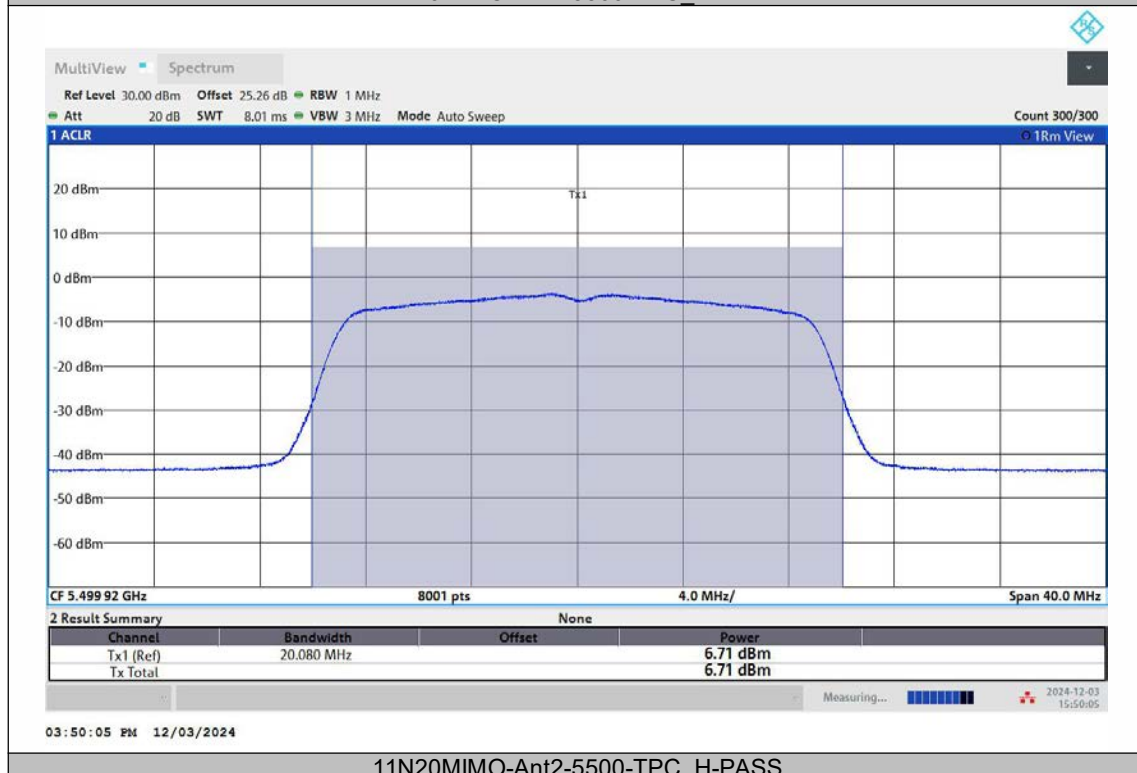
11N20MIMO-Ant2-5500-TPC_H-PASS
