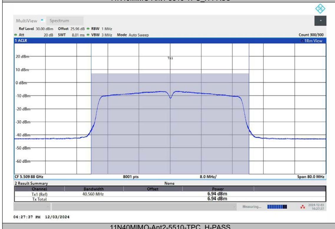
11N40MIMO-Ant2-5510-TPC_H-PASS
