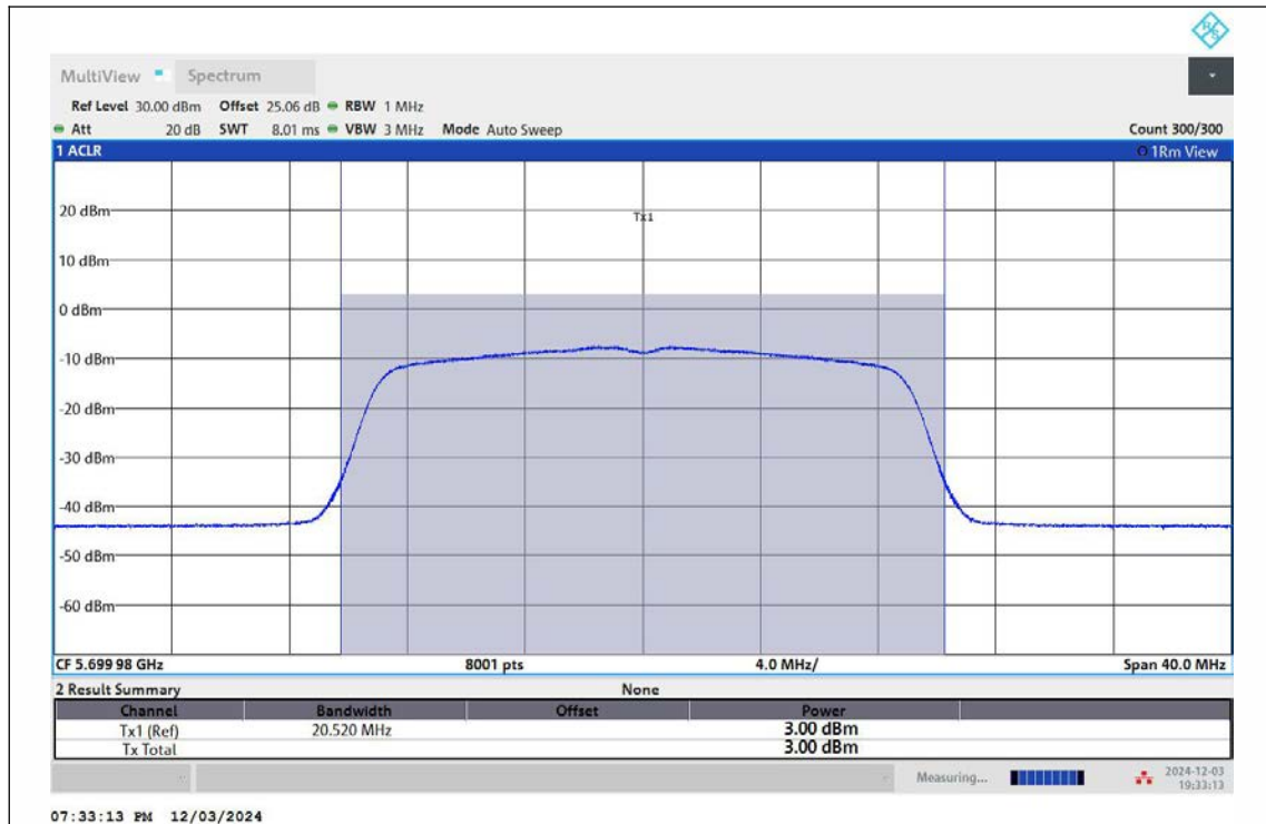
11N20MIMO-Ant1-5700-TPC_L-PASS
