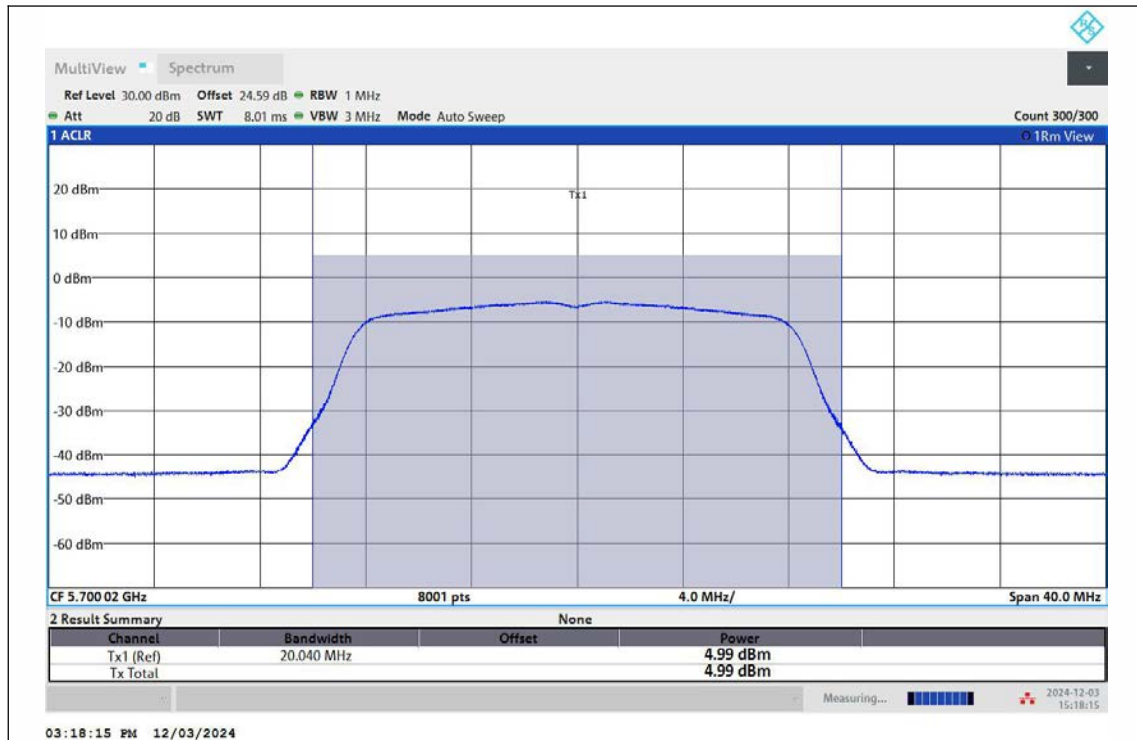
11A-Ant2-5700-TPC_L-PASS
