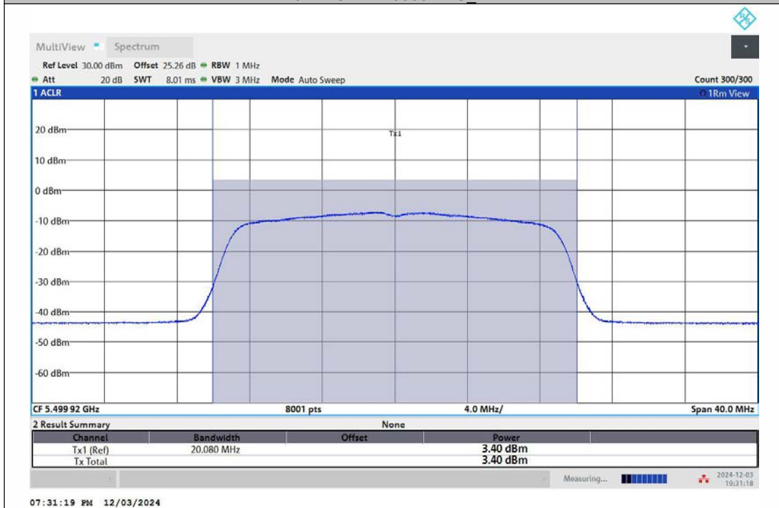
11N20MIMO-Ant2-5500-TPC_L-PASS
