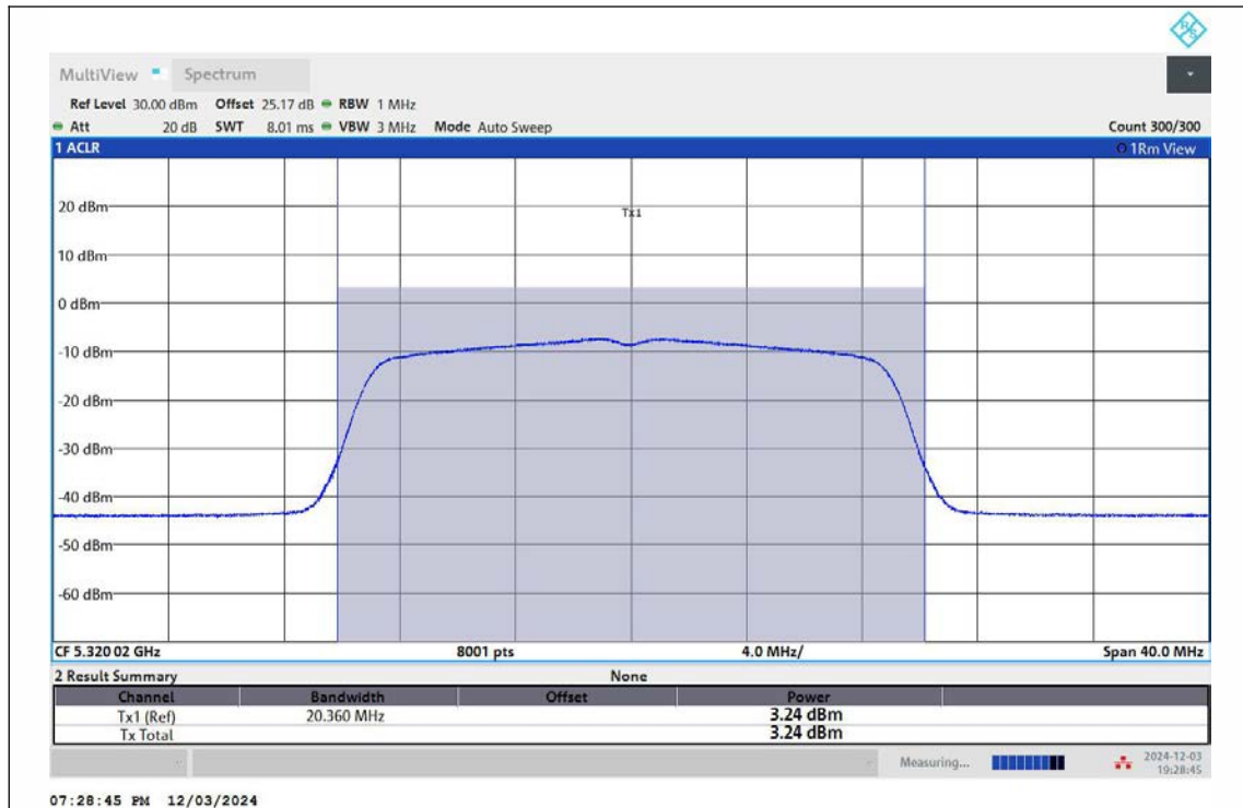
11N20MIMO-Ant1-5320-TPC_L-PASS
