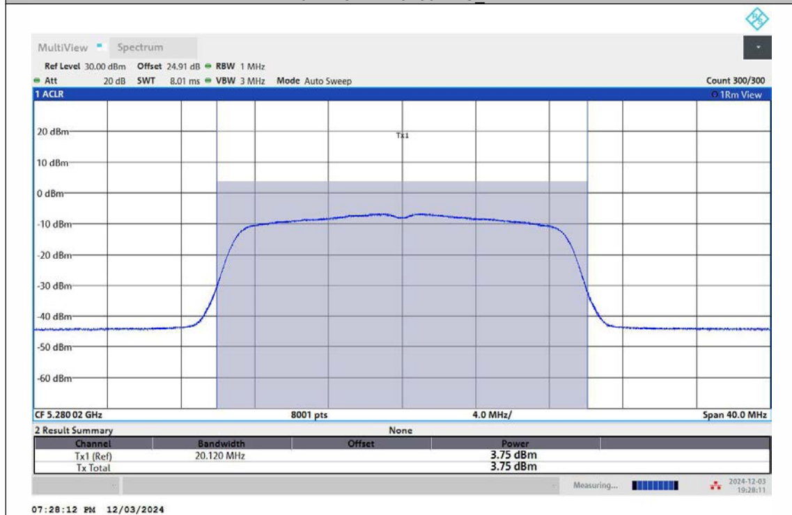
11N20MIMO-Ant2-5280-TPC_L-PASS
