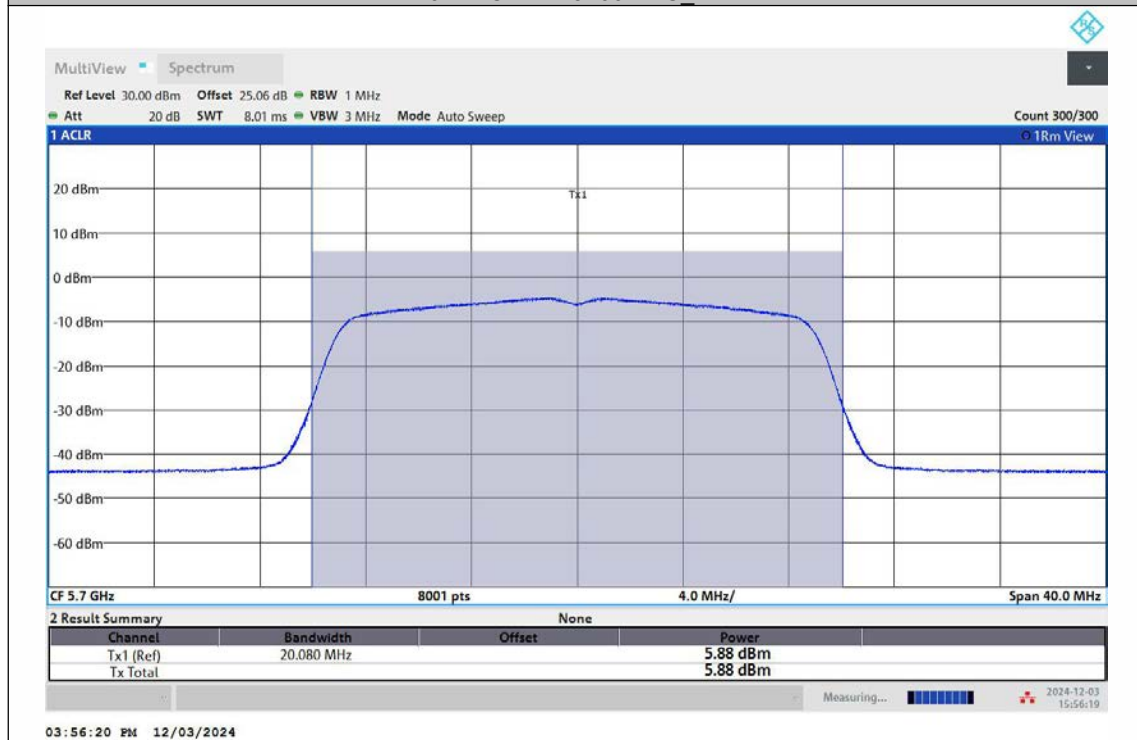
11N20MIMO-Ant2-5700-TPC_H-PASS
