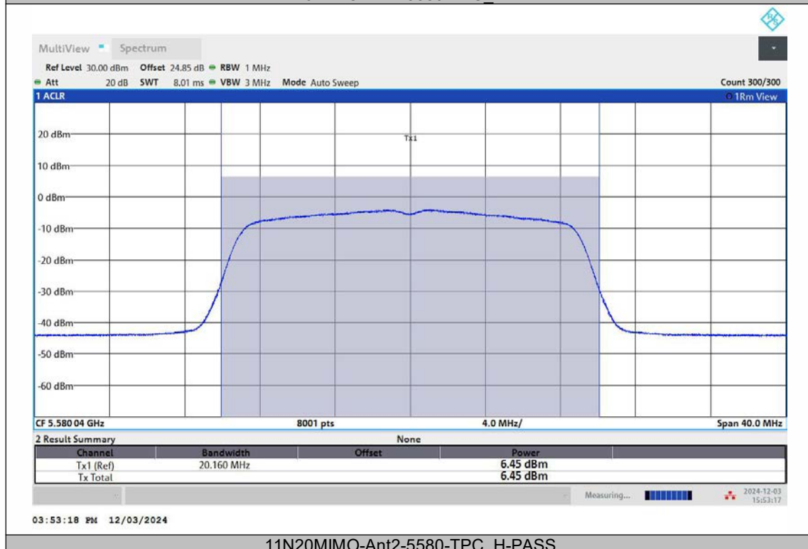
11N20MIMO-Ant2-5580-TPC_H-PASS
