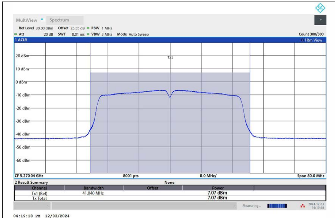
11N40MIMO-Ant1-5270-TPC_H-PASS
