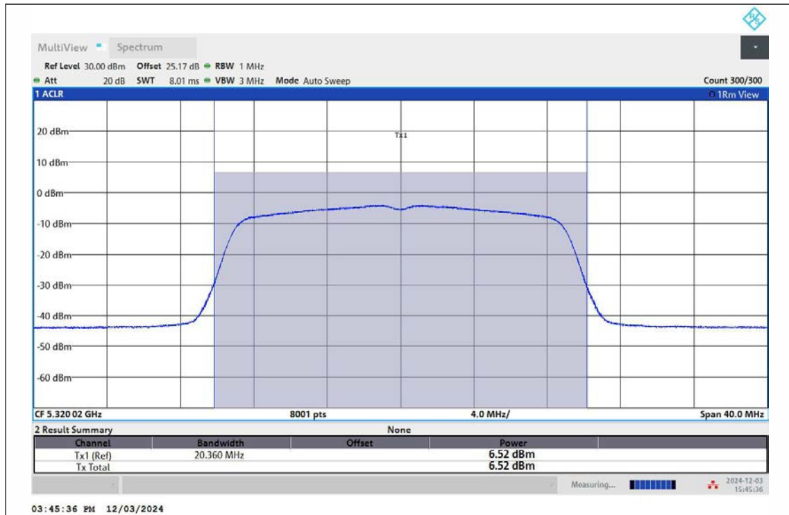
11N20MIMO-Ant1-5320-TPC_H-PASS
