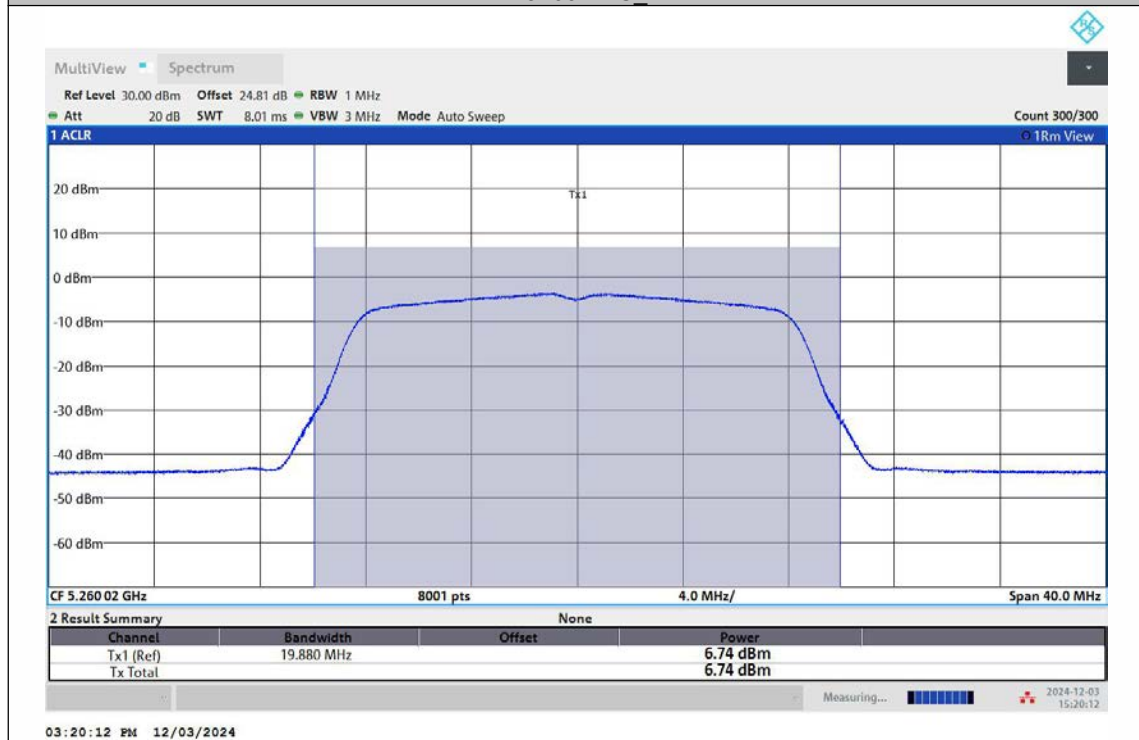
11A-Ant1-5260-TPC_L-PASS
