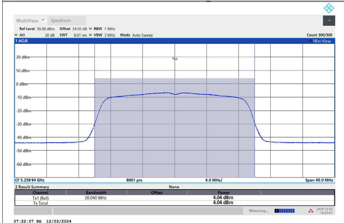
11N20MIMO-Ant2-5260-TPC_L-PASS
