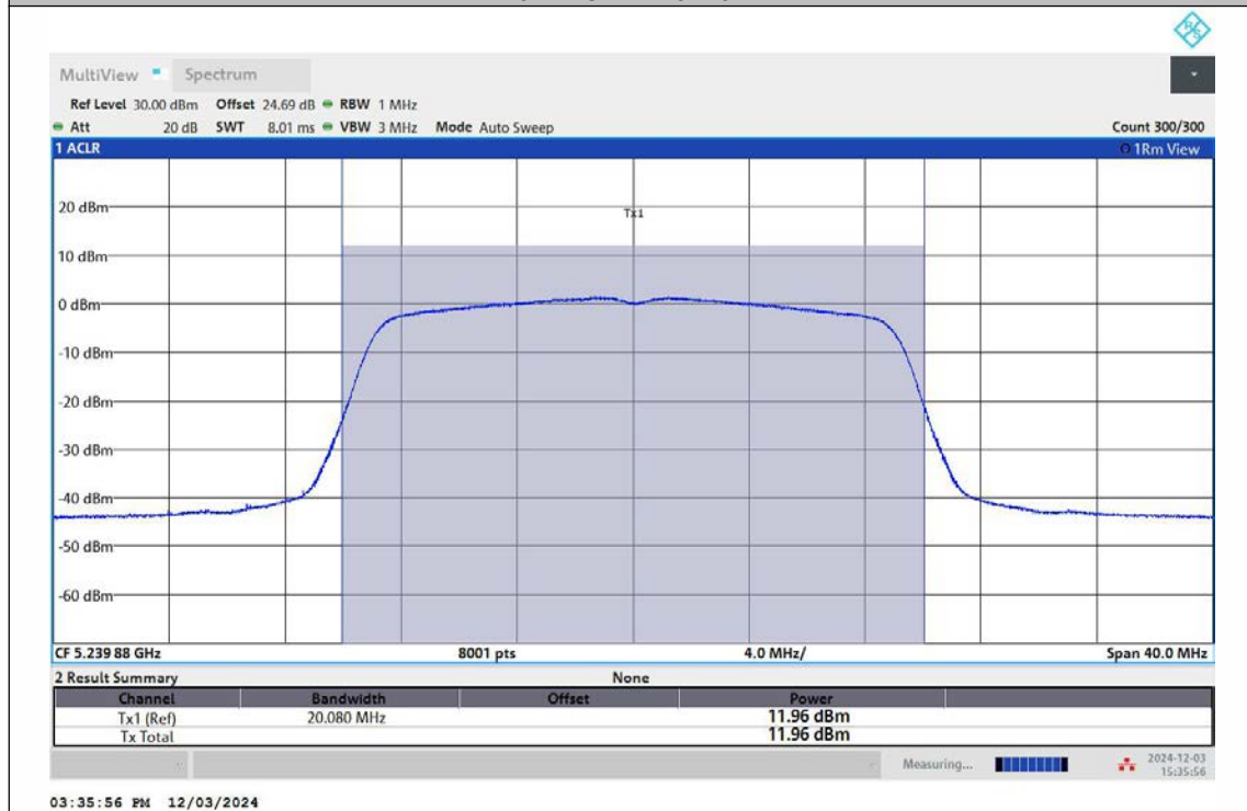
11N20MIMO-Ant2-5240-PASS
