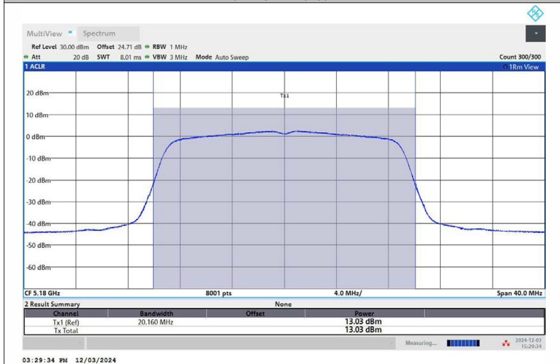
11N20MIMO-Ant2-5180-PASS
