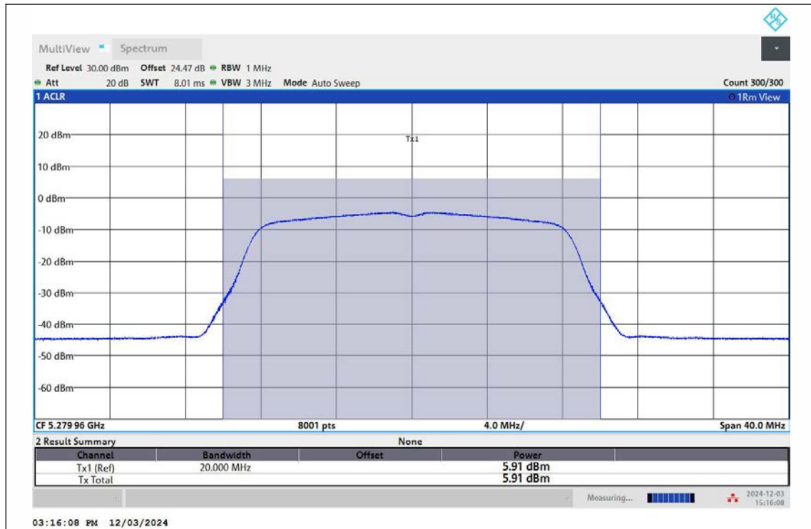
11A-Ant2-5280-TPC_L-PASS
