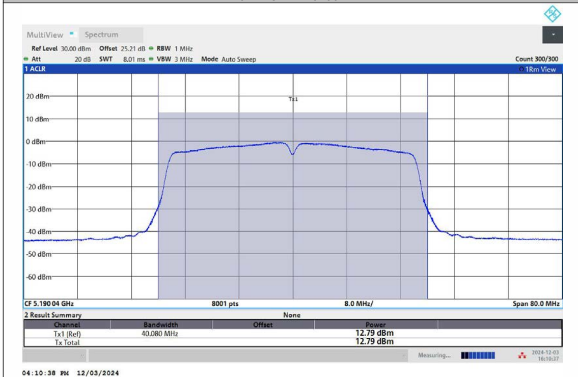
11N40MIMO-Ant2-5190-PASS
