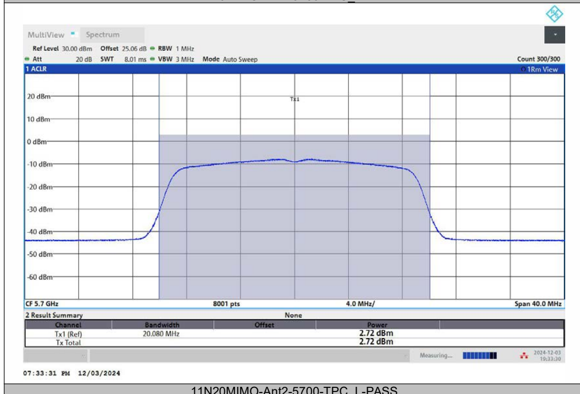
11N20MIMO-Ant2-5700-TPC_L-PASS
