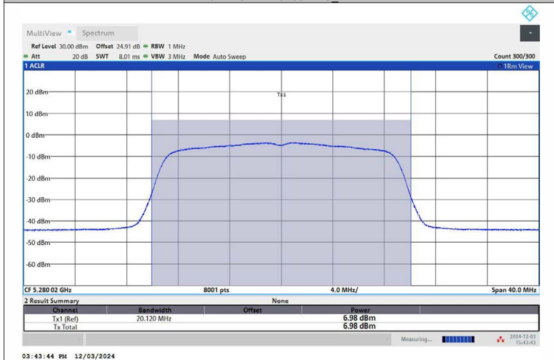
11N20MIMO-Ant2-5280-TPC_H-PASS
