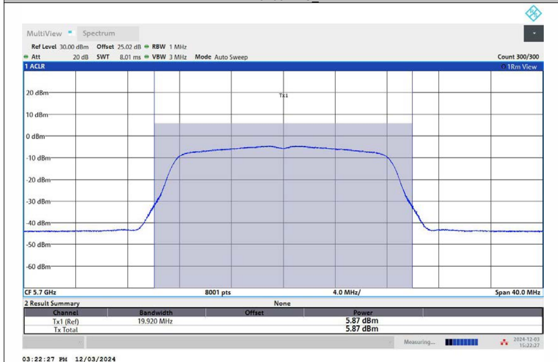
11A-Ant1-5700-TPC_L-PASS
