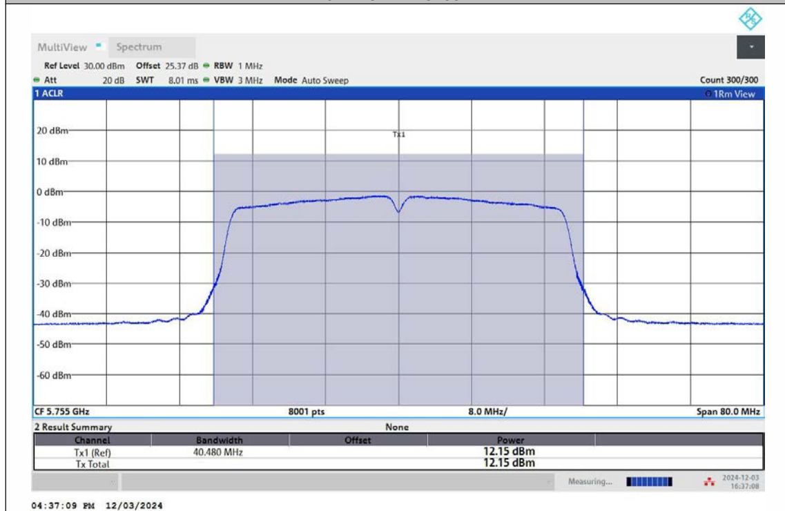
11N40MIMO-Ant2-5755-PASS
