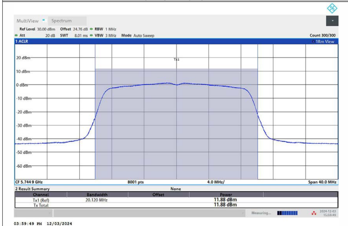
11N20MIMO-Ant2-5745-PASS
