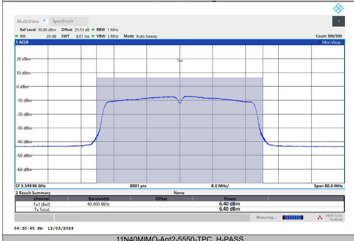
11N40MIMO-Ant2-5550-TPC_H-PASS
