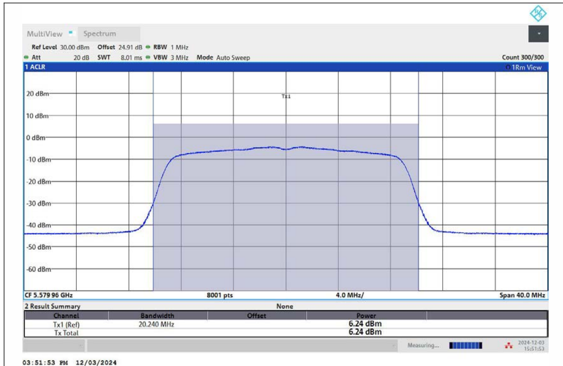
11N20MIMO-Ant1-5580-TPC_H-PASS
