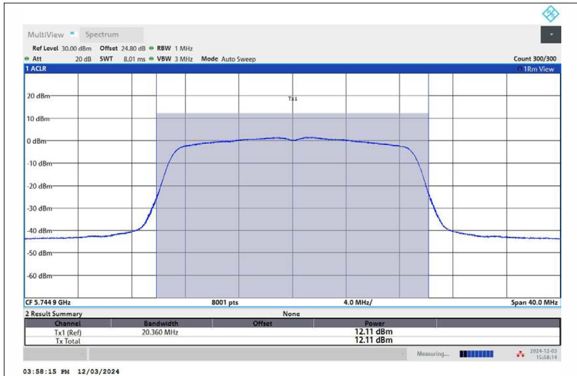
11N20MIMO-Ant1-5745-PASS
