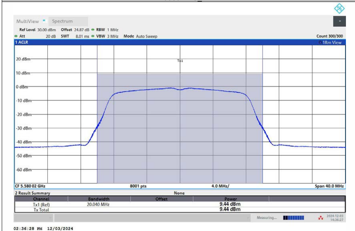
11A-Ant1-5580-TPC_H-PASS
