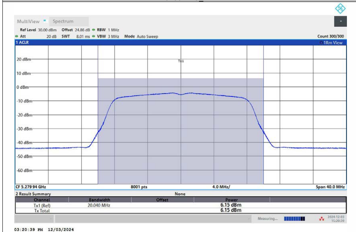
11A-Ant1-5280-TPC_L-PASS
