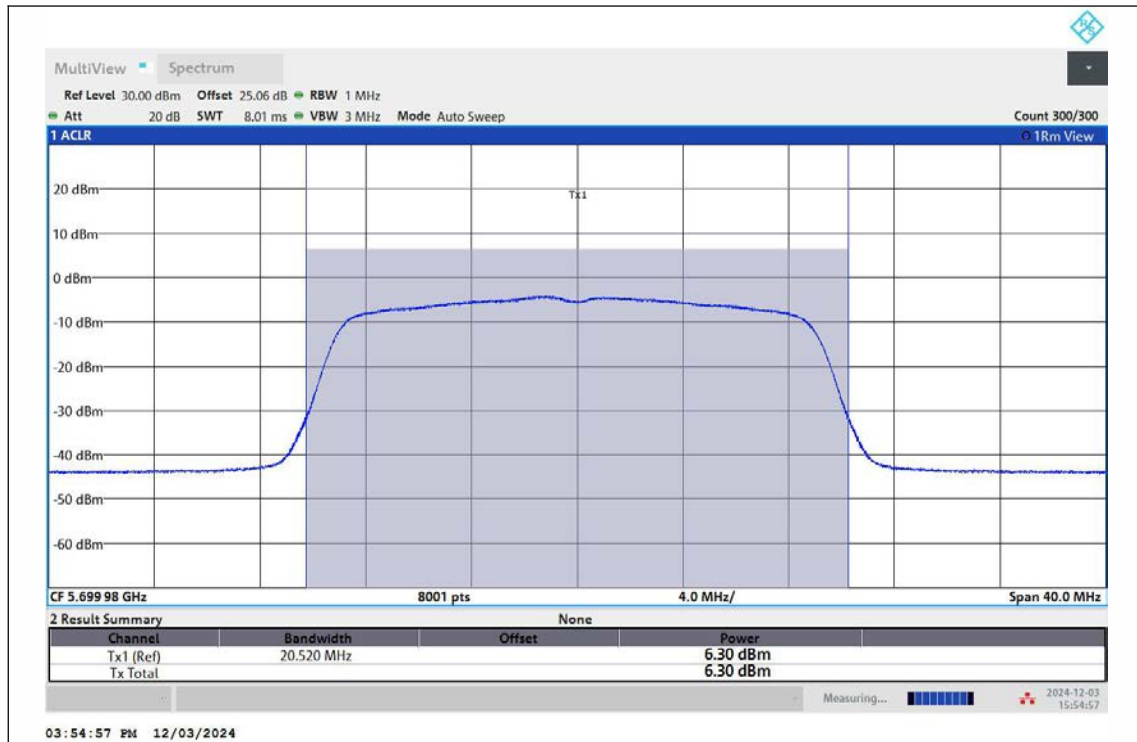
11N20MIMO-Ant1-5700-TPC_H-PASS
