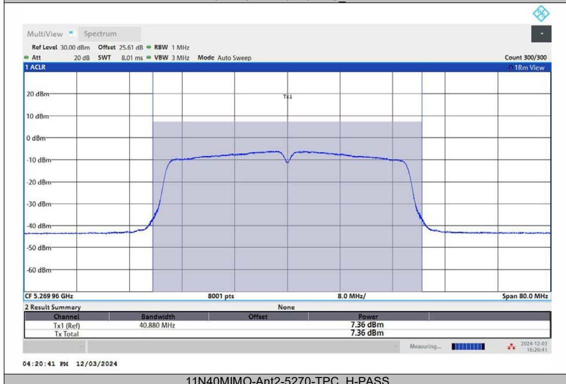
11N40MIMO-Ant2-5270-TPC_H-PASS
