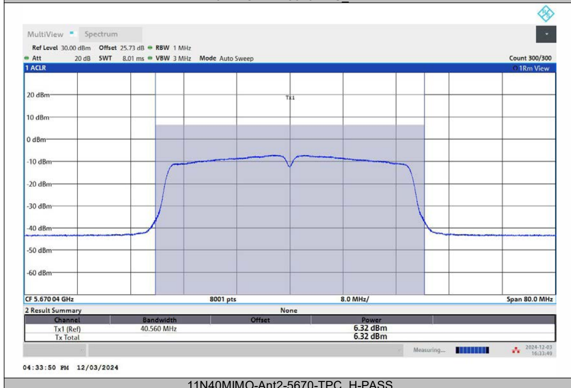
11N40MIMO-Ant2-5670-TPC_H-PASS
