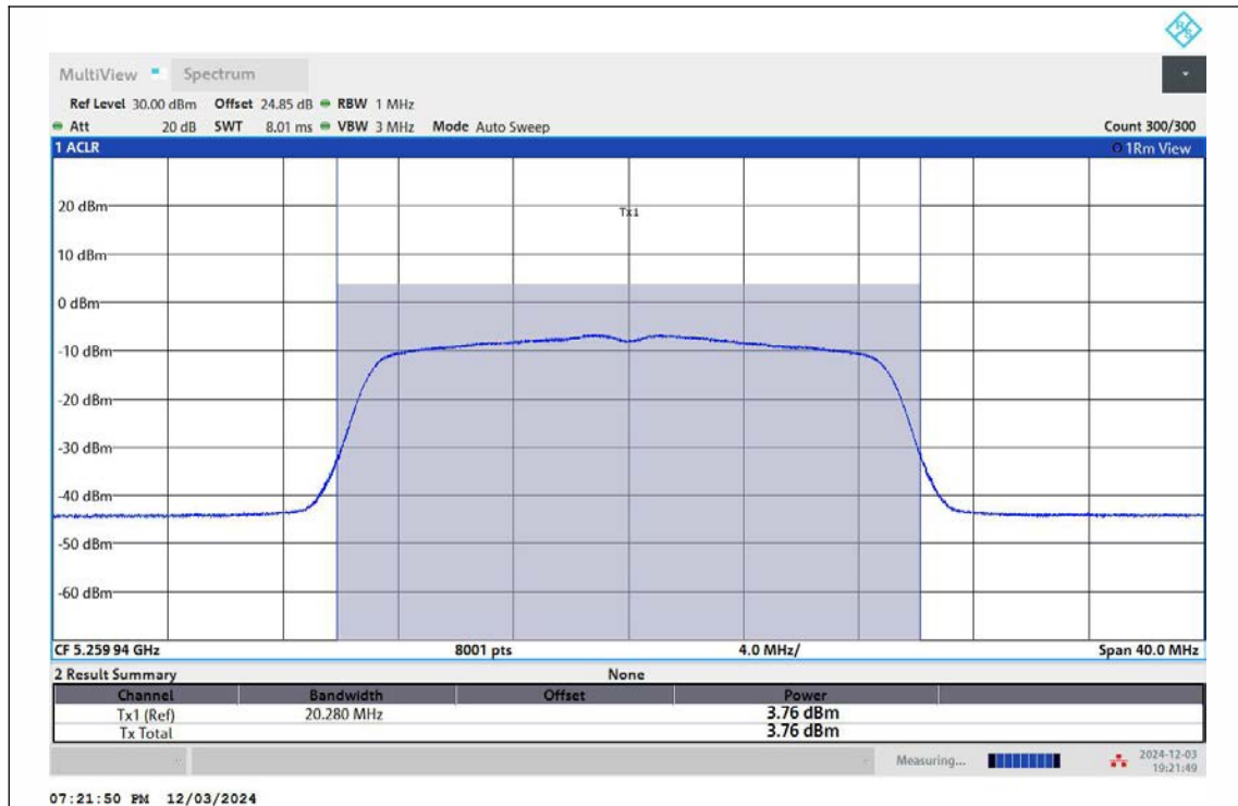
11N20MIMO-Ant1-5260-TPC_L-PASS
