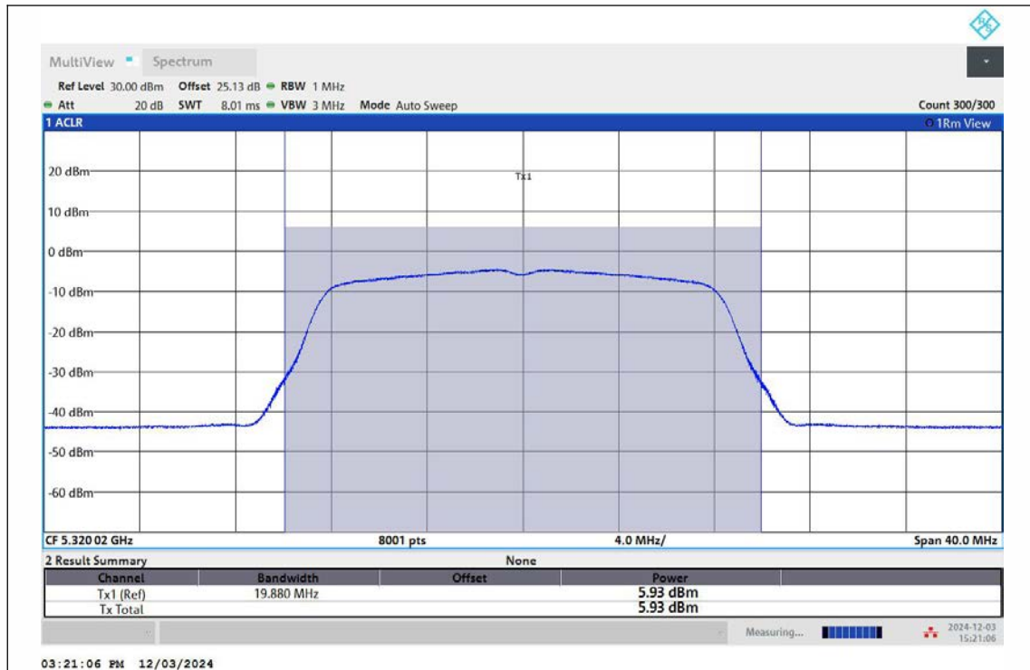
11A-Ant1-5320-TPC_L-PASS
