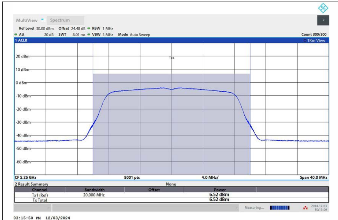
11A-Ant2-5260-TPC_L-PASS
