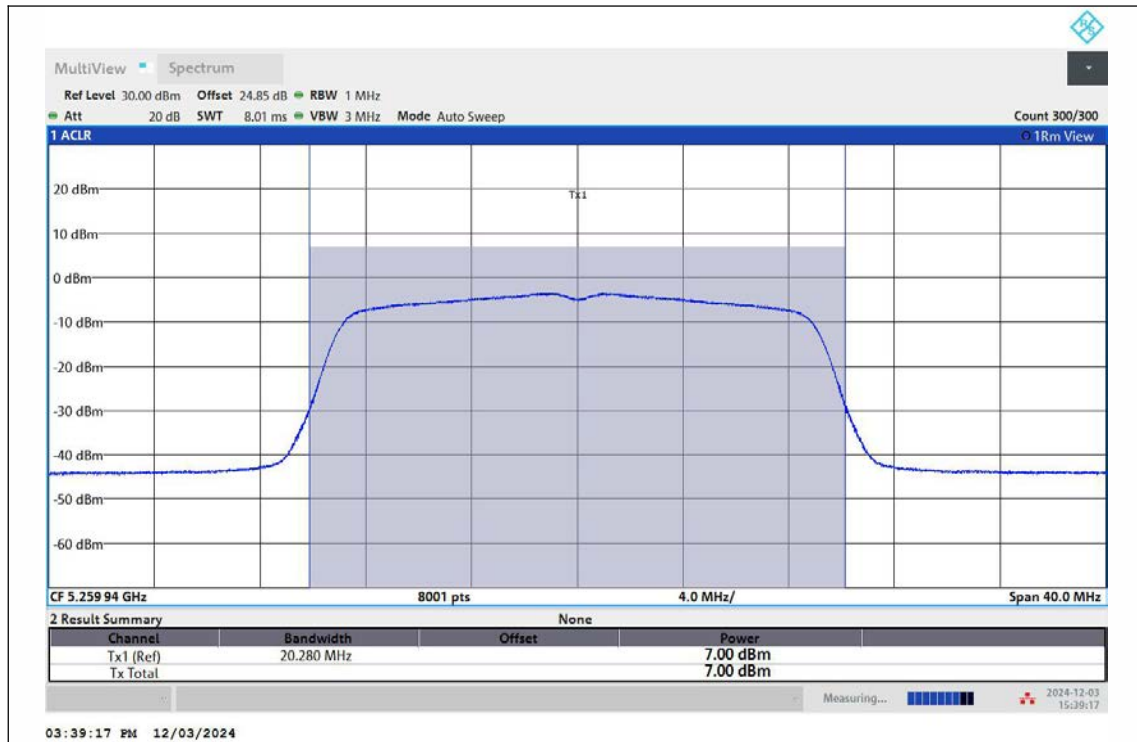
11N20MIMO-Ant1-5260-TPC_H-PASS
