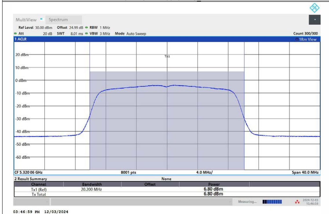
11N20MIMO-Ant2-5320-TPC_H-PASS
