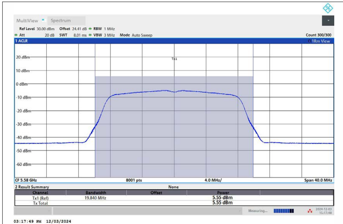
11A-Ant2-5580-TPC_L-PASS
