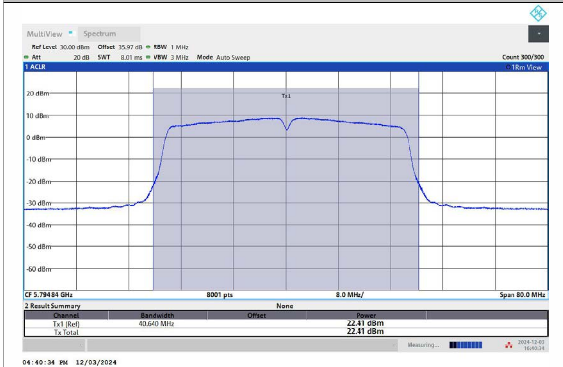
11N40MIMO-Ant2-5795-PASS
