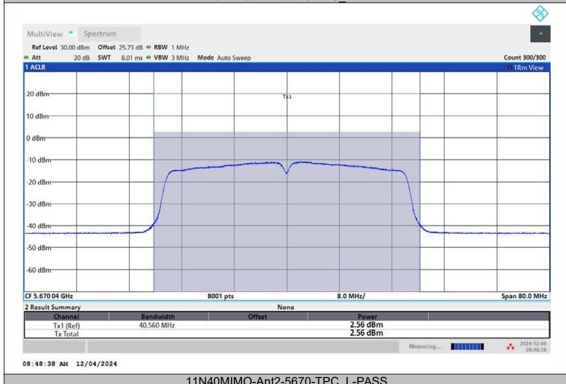
11N40MIMO-Ant2-5670-TPC_L-PASS
