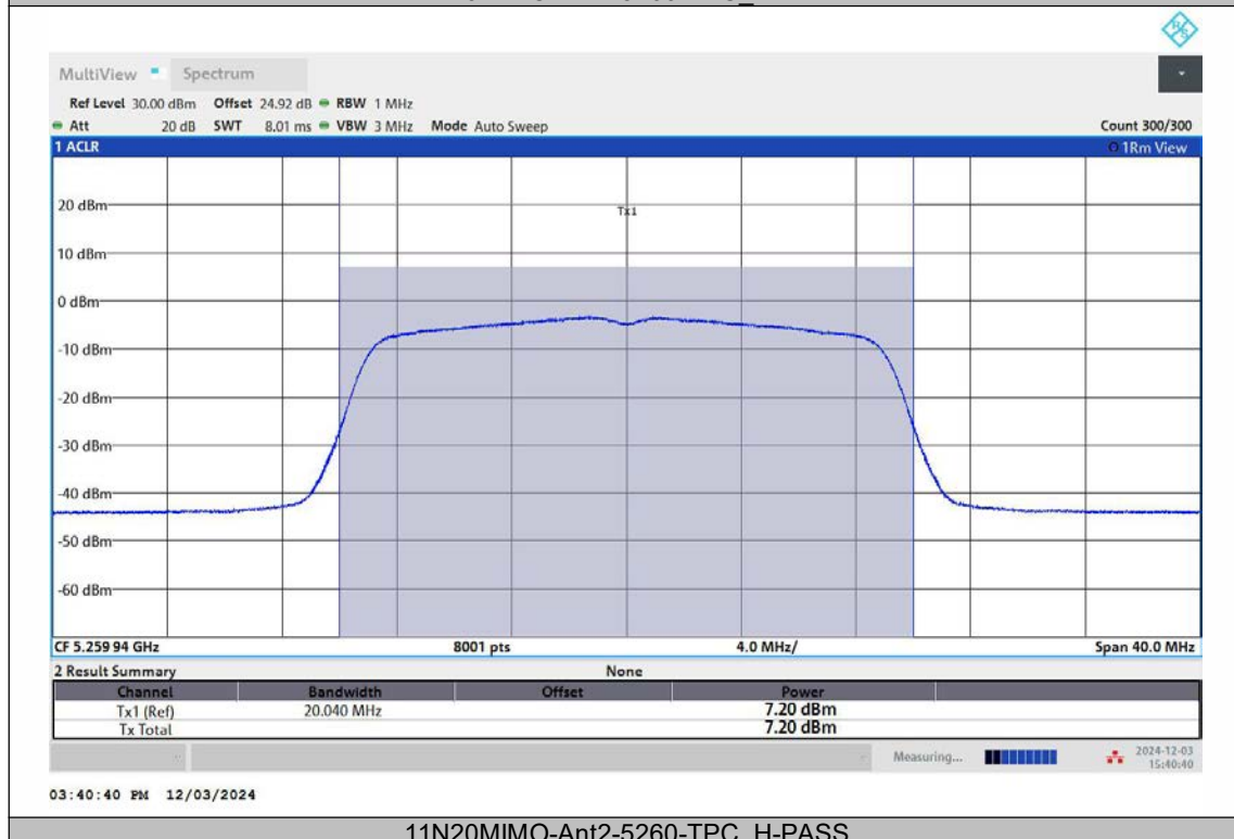
11N20MIMO-Ant2-5260-TPC_H-PASS
