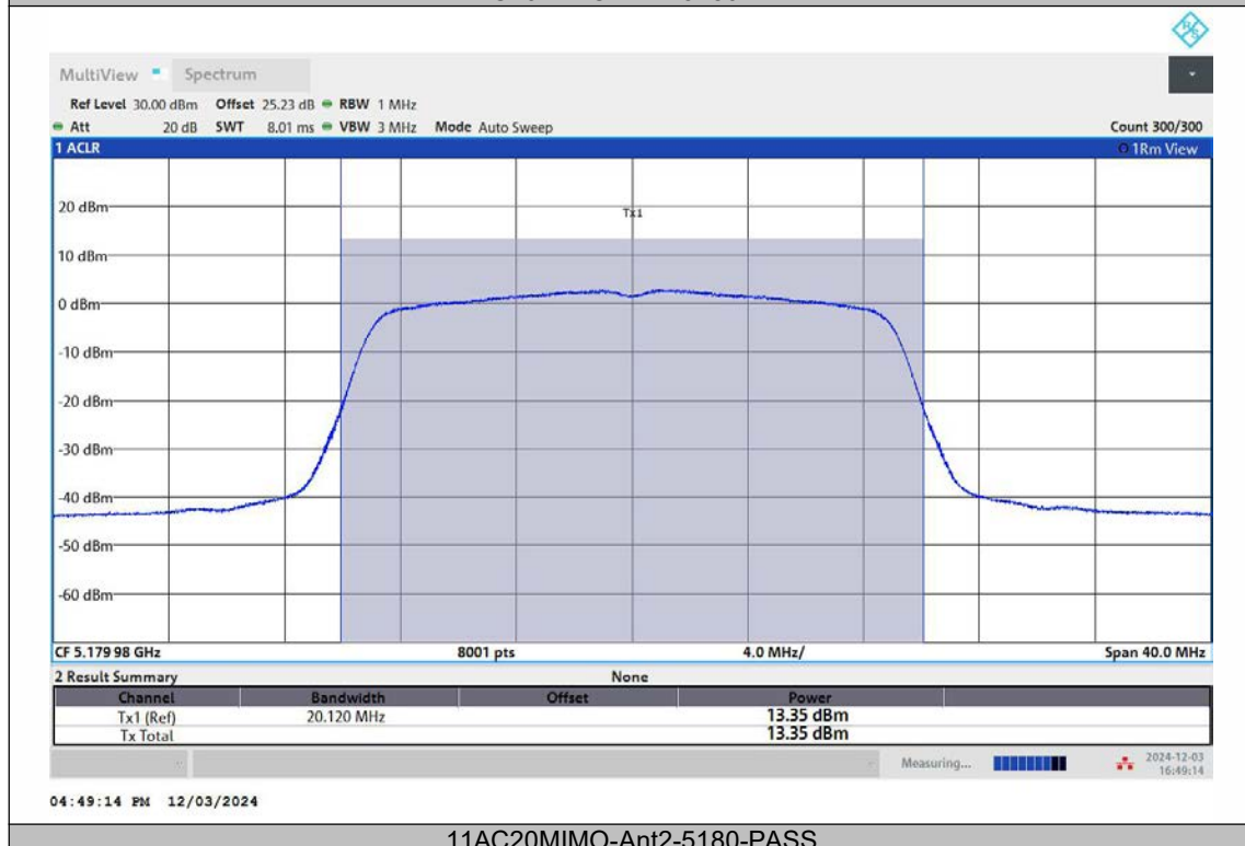
11AC20MIMO-Ant2-5180-PASS
