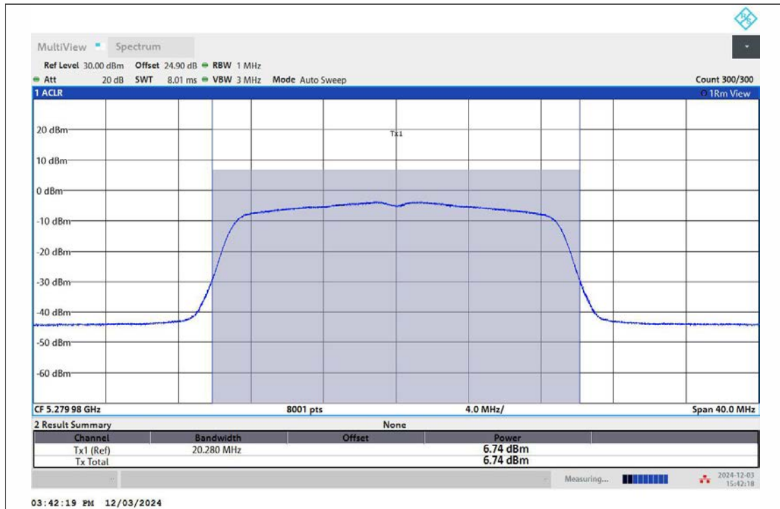
11N20MIMO-Ant1-5280-TPC_H-PASS
