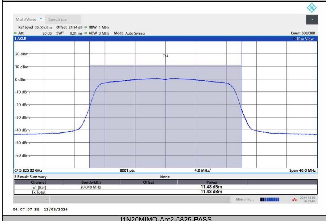
11N20MIMO-Ant2-5825-PASS
