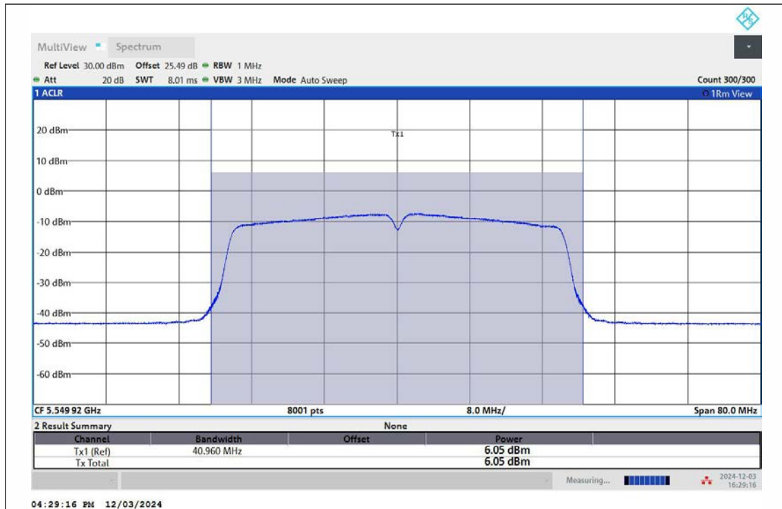
11N40MIMO-Ant1-5550-TPC_H-PASS
