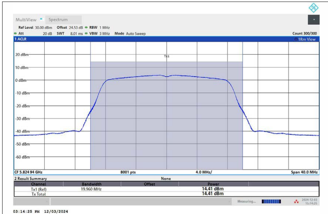
11A-Ant2-5825-PASS
