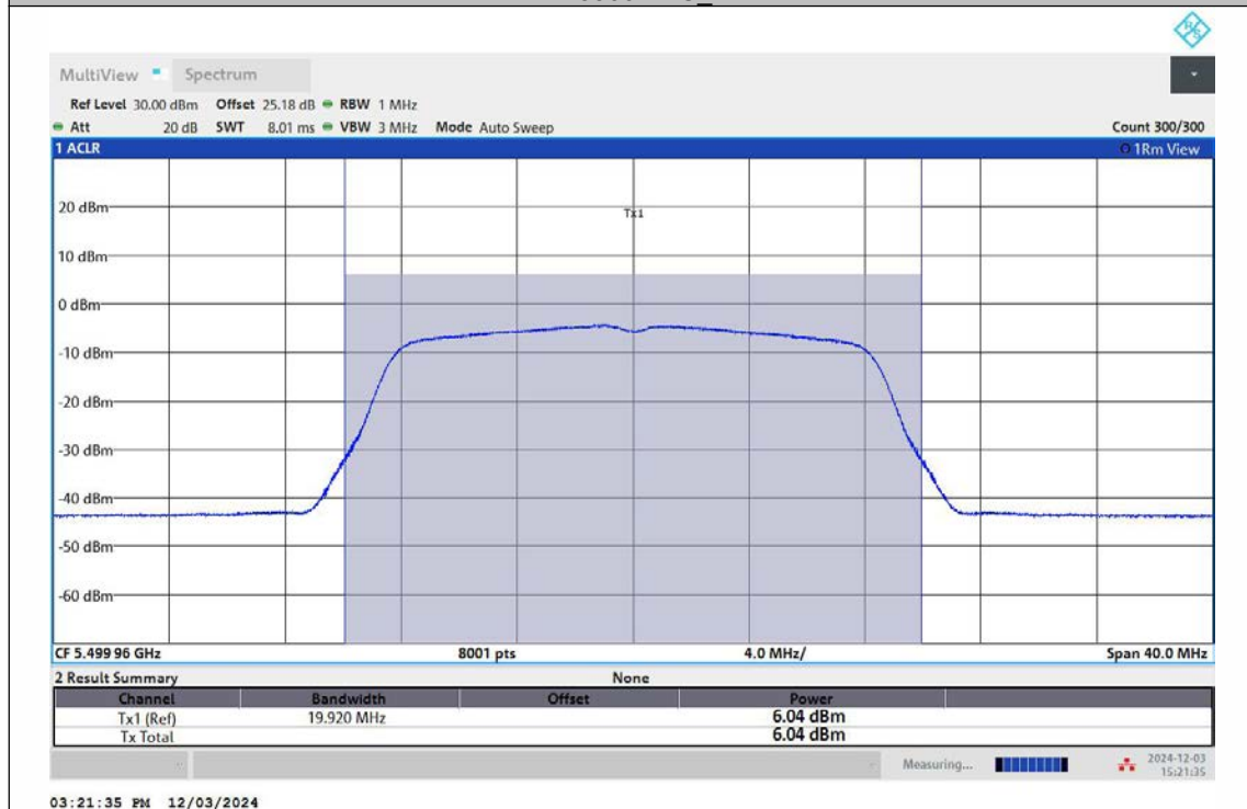
11A-Ant1-5500-TPC_L-PASS
