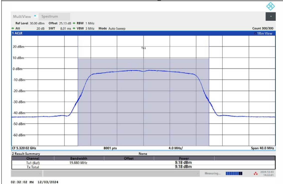
11A-Ant1-5320-TPC_H-PASS
