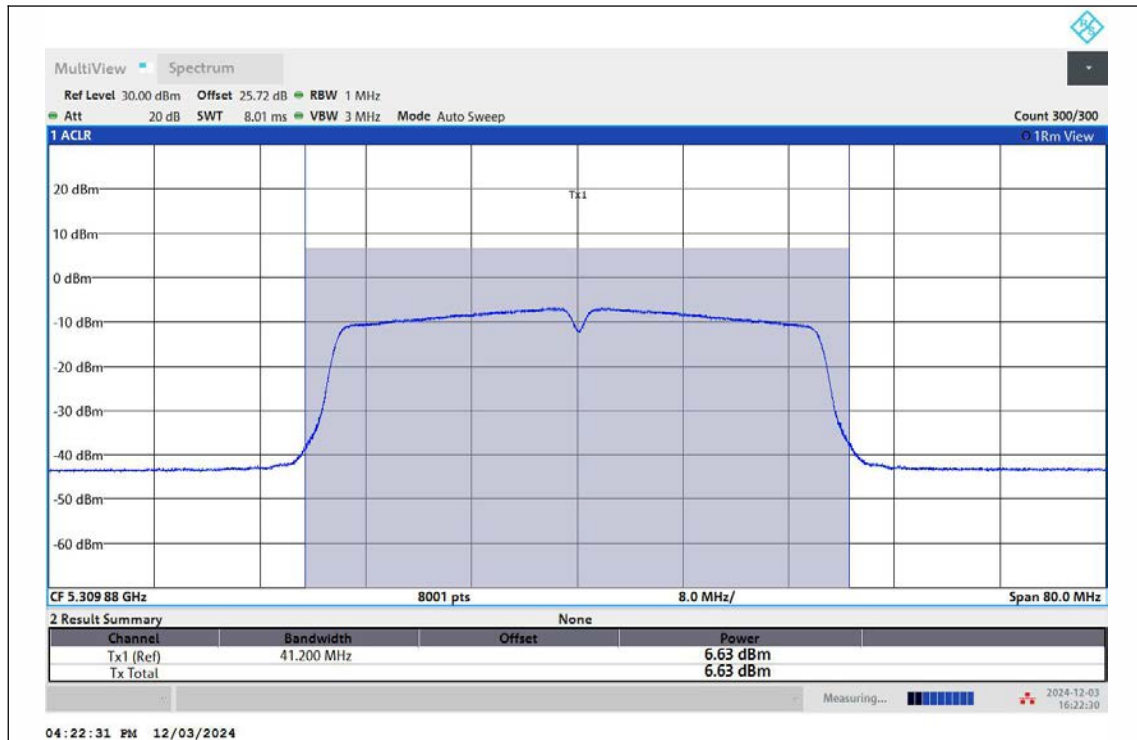
11N40MIMO-Ant1-5310-TPC_H-PASS
