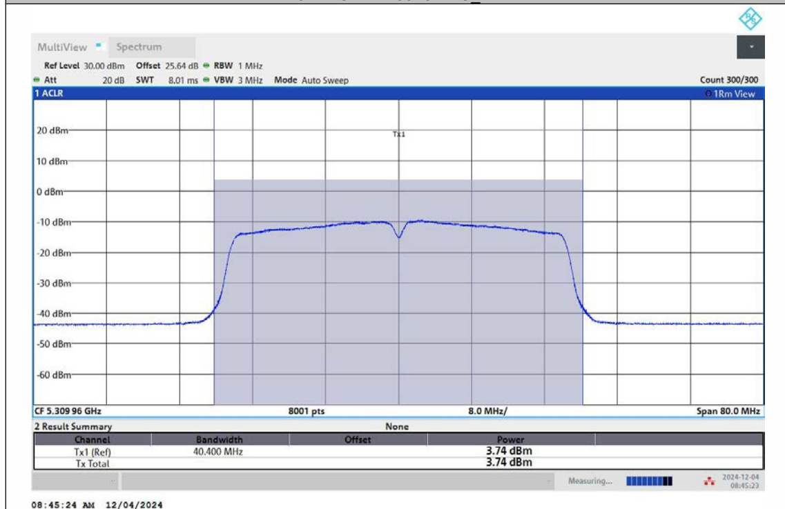
11N40MIMO-Ant2-5310-TPC_L-PASS
