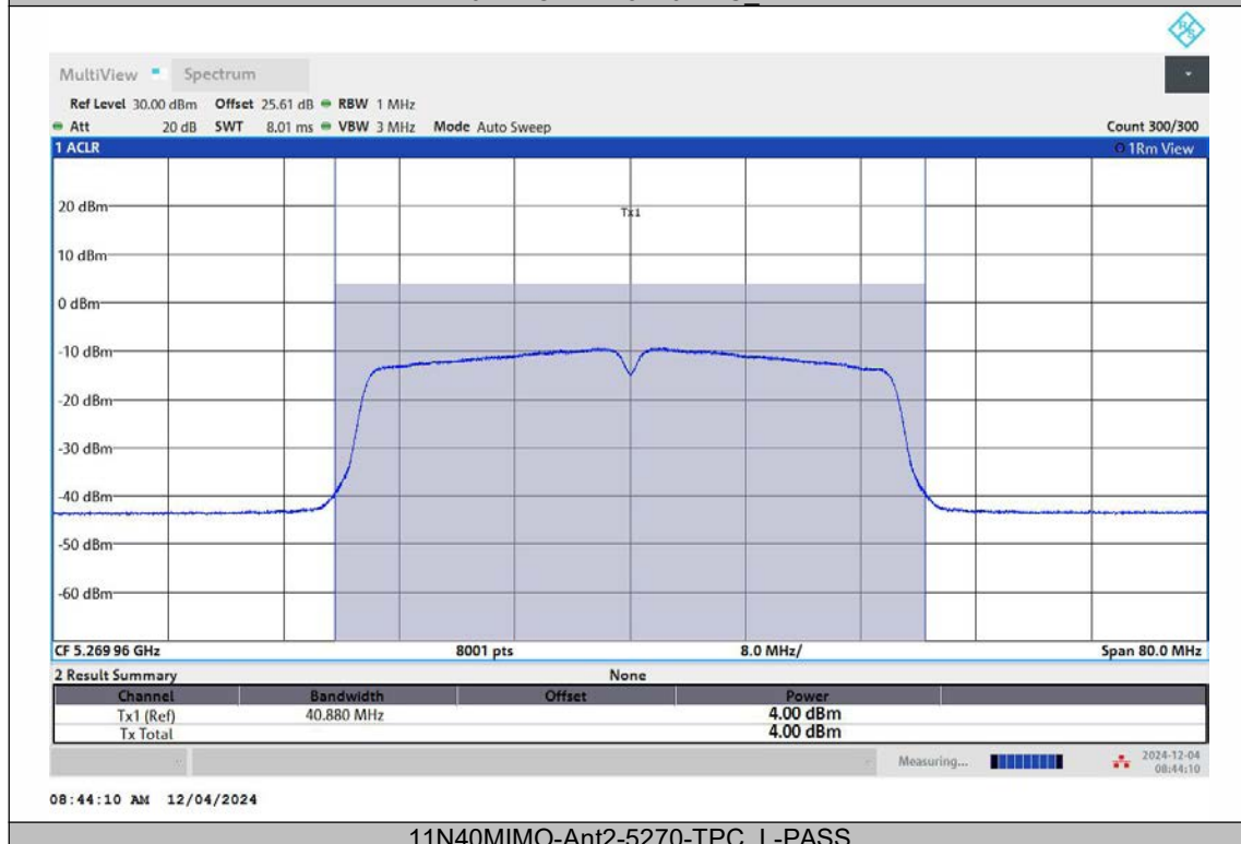
11N40MIMO-Ant2-5270-TPC_L-PASS
