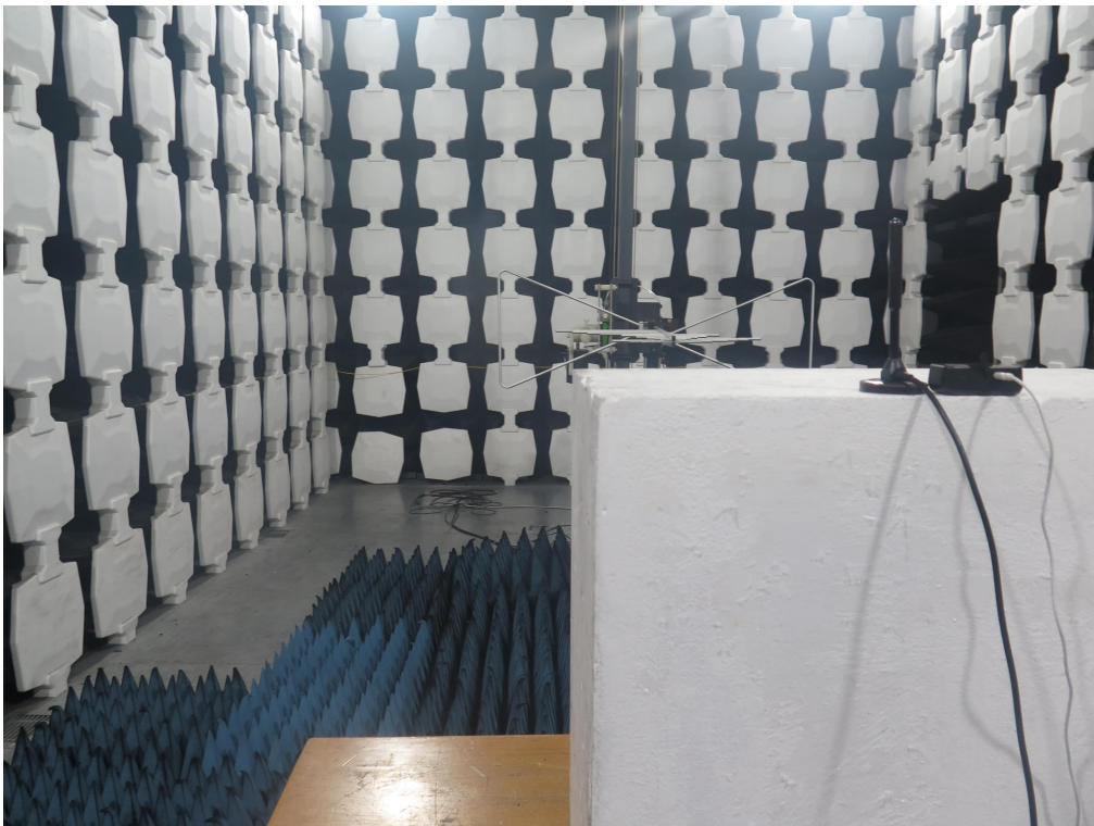
RSE_1G-3GHz
