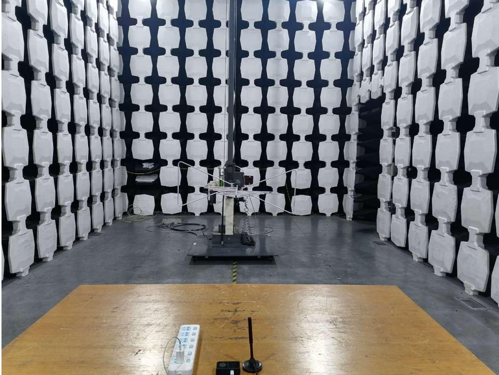
RSE_30M-1GHz
