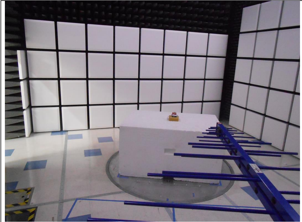
RF Radiated 30 MHz-1GHz
