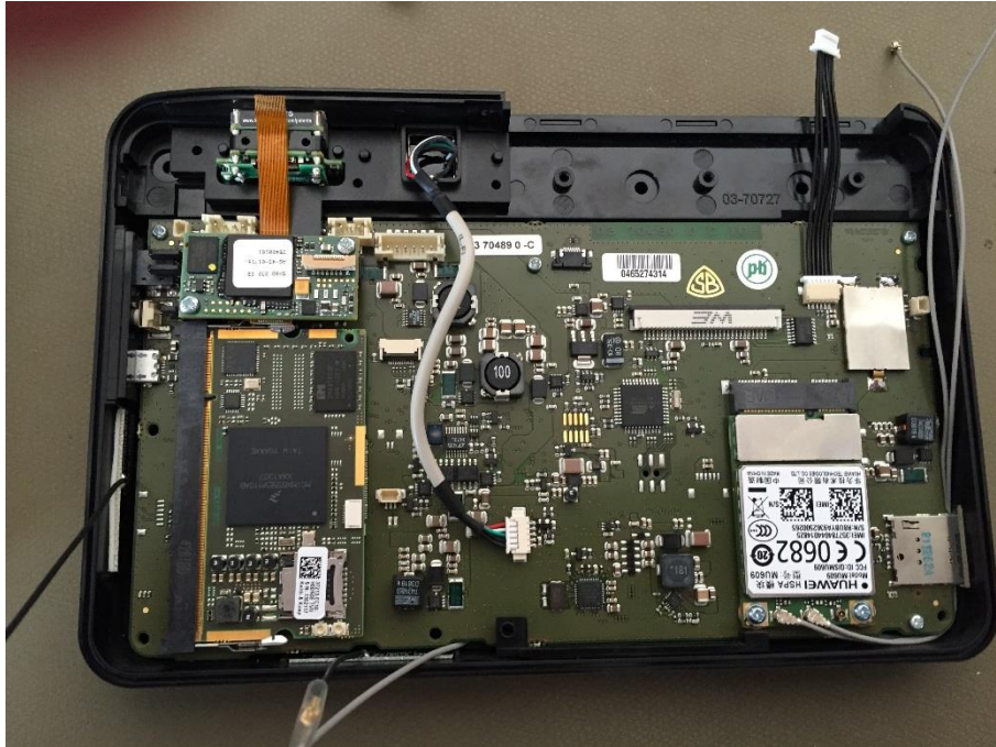
Photo 3 - PCB view:
