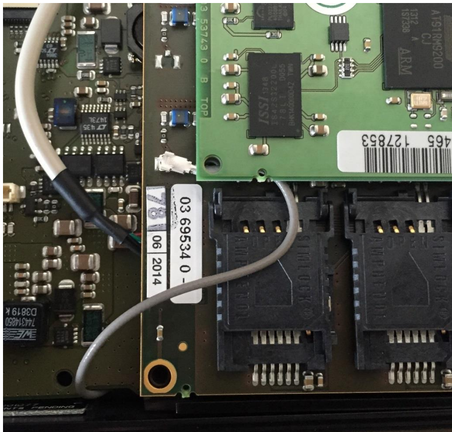
Photo 8 - SCR3:
