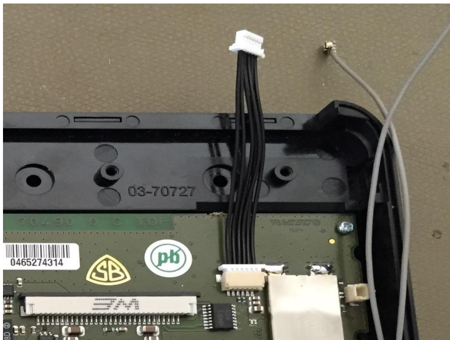
Photo 6 - SCR:
