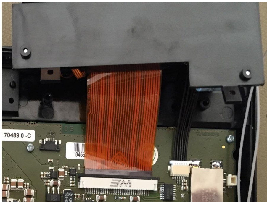
Photo 5 - Printer:
