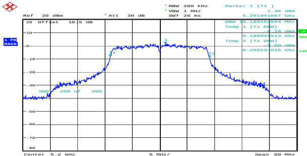
n20_5200MHz_Chain 0 18.189MHz
