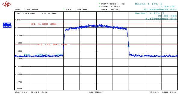
ax40_5190MHz_RU_Full_Chain 0 39.888MHz
