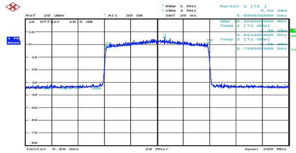
ax80_5690MHz_RU_Full_Chain 0 76.960MHz
