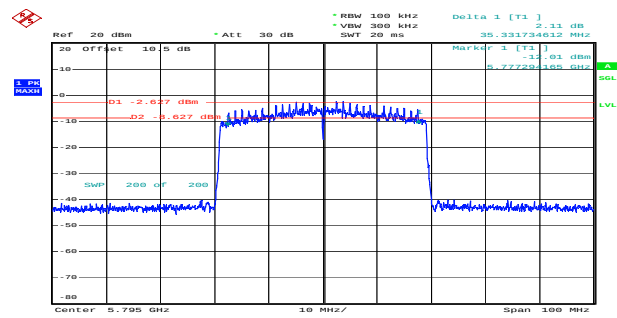
ax40_5795MHz_RU_Full_Chain 0 35.332MHz
