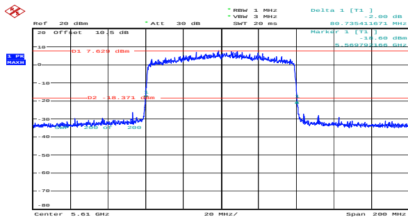
ax80_5610MHz_RU_Full_Chain 0 80.735MHz
