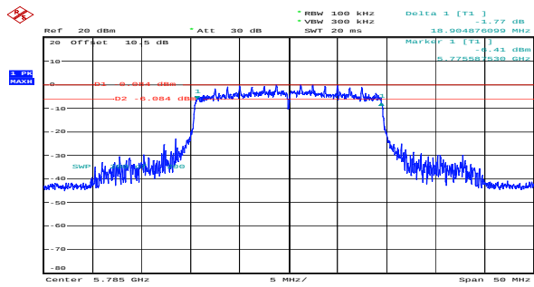
ax20_5785MHz_RU_Full_Chain 0 18.905MHz
