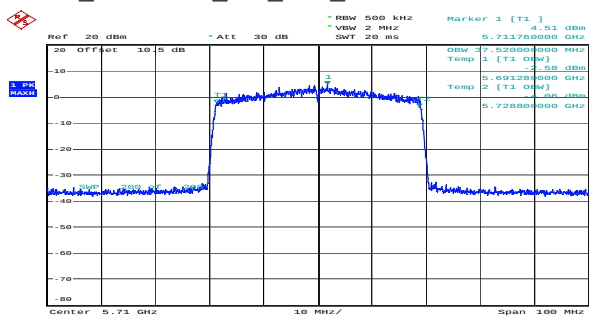
ax40_5710MHz_RU_Full_Chain 0 37.520MHz
