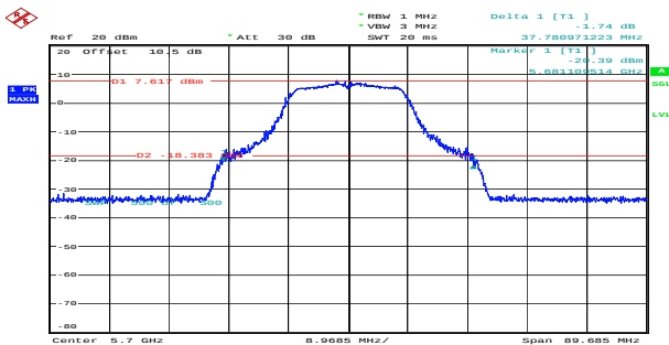
n20_5700MHz_Chain 0 37.781MHz
