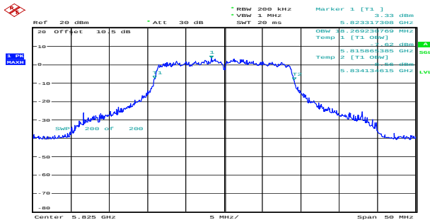
n20_5825MHz_Chain 0 18.269MHz
