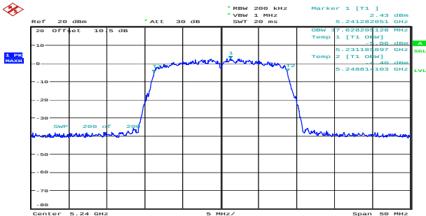
n20_5240MHz_Chain 0 17.628MHz
