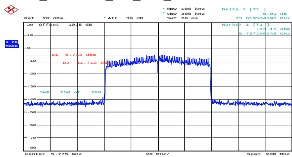
ax80_5775MHz_RU_Full_Chain_0_75.620MHz
