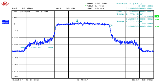
ax20_5200MHz_RU_Full_Chain 0 19.120MHz
