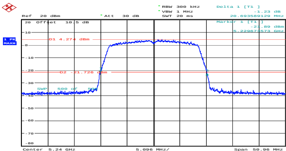
n20_5240MHz_Chain 0 20.694MHz
