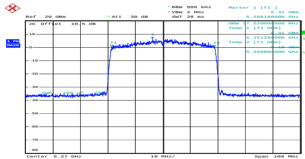
ax40_5270MHz_RU_Full_Chain 0 37.520MHz
