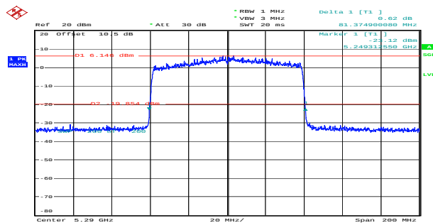
ax80_5290MHz_RU_Full_Chain 0 81.375MHz
