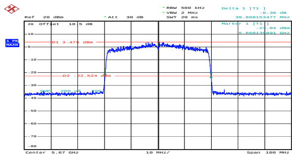
ax40_5670MHz_RU_Full_Chain 0 39.808MHz
