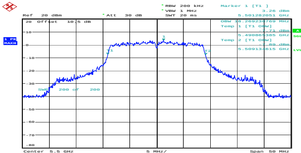
n20_5500MHz_Chain 0 18.269MHz
