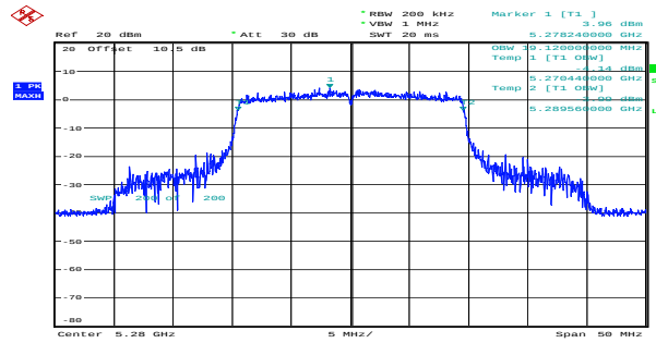
ax20_5280MHz_RU_Full_Chain 0 19.120MHz
