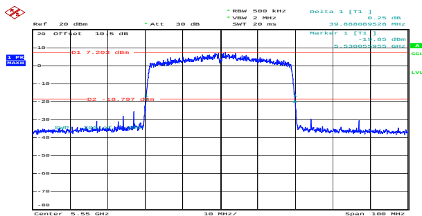
ax40_5550MHz_RU_Full_Chain 0 39.888MHz
