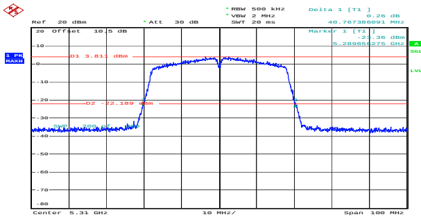
n40_5310MHz_Chain 0 40.767MHz
