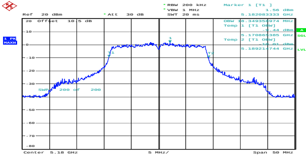
n20_5180MHz_Chain 0 18.349MHz
