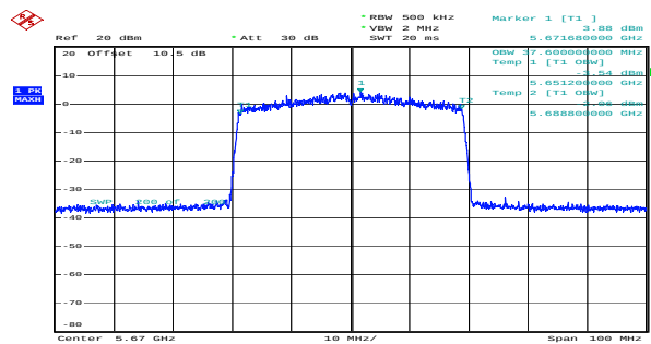
ax40_5670MHz_RU_Full_Chain 0 37.600MHz
