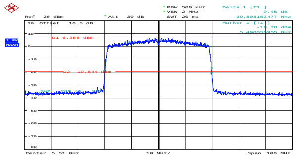
ax40_5510MHz_RU_Full_Chain 0 39.808MHz
