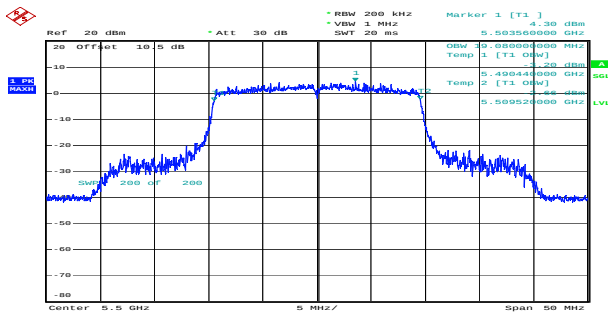
ax20_5500MHz_RU_Full_Chain 0 19.080MHz
