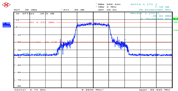
ax20_5720MHz_RU_Full_Chain 0 36.812MHz
