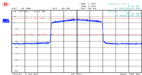
ax80_5530MHz_RU_Full_Chain 0 81.055MHz
