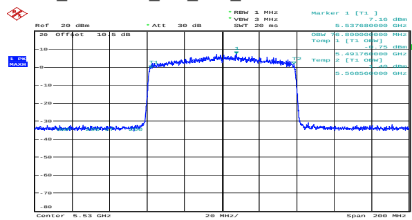
ax80_5530MHz_RU_Full_Chain 0 76.800MHz
