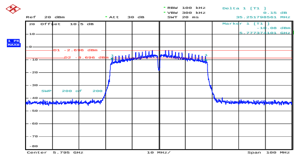
n40_5795MHz_Chain 0 35.252MHz
