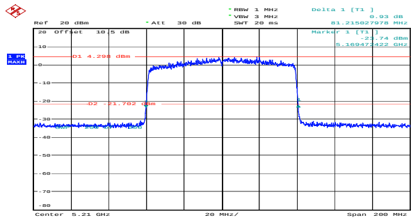
ax80_5210MHz_RU_Full_Chain 0 81.215MHz
