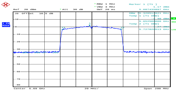
ac80_5690MHz_Chain 0 75.321MHz
