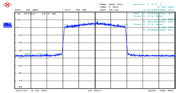
ax40_5510MHz_RU_Full_Chain 0 37.600MHz
