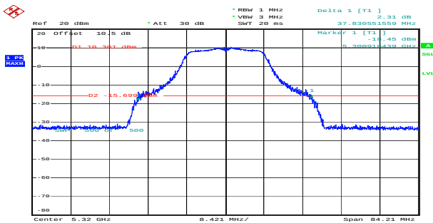
n20_5320MHz_Chain 0 37.831MHz
