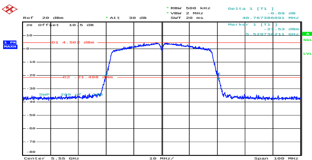
n40_5550MHz_Chain 0 40.767MHz
