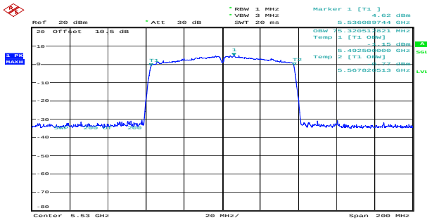
ac80_5530MHz_Chain 0 75.321MHz
