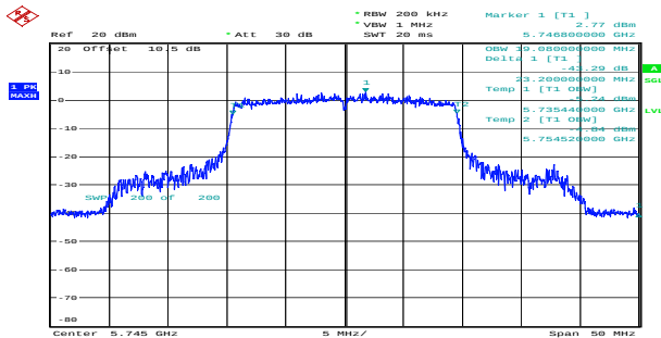
ax20_5745MHz_RU_Full Chain 0 19.080MHz
