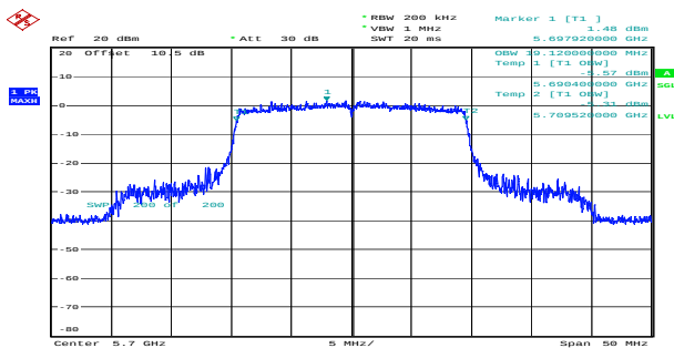
ax20_5700MHz_RU_Full_Chain 0 19.120MHz
