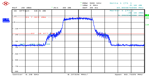
ax20_5280MHz_RU_Full_Chain 0 34.805MHz
