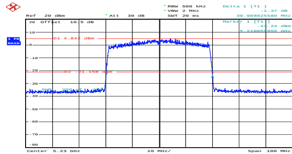
ax40_5230MHz_RU_Full_Chain 0 39.968MHz
