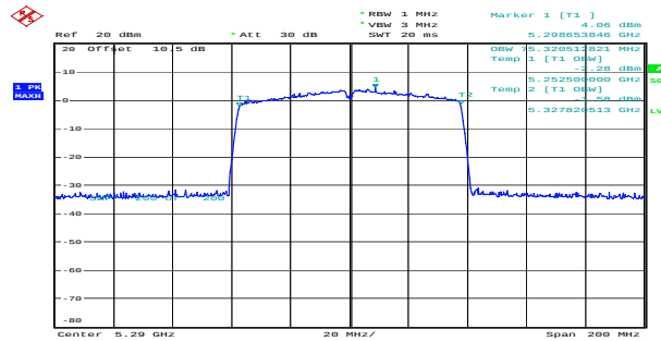
ac80_5290MHz_Chain 0 75.321MHz
