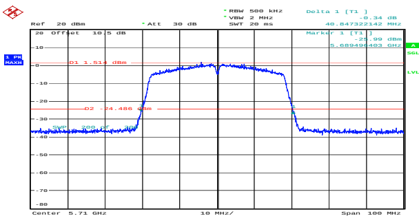
n40_5710MHz_Chain 0 40.847MHz
