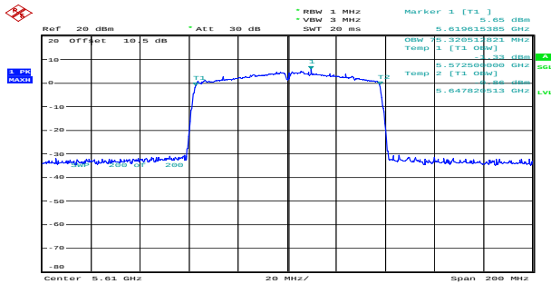
ac80_5610MHz_Chain 0 75.321MHz
