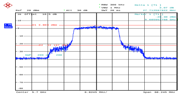
ax20_5700MHz_RU_Full_Chain 0 27.713MHz
