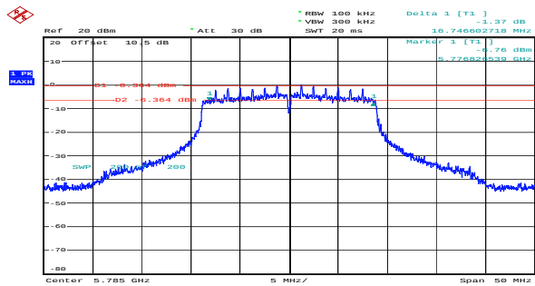
n20_5785MHz_Chain 0 16.747MHz
