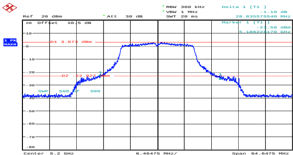
n20_5200MHz_Chain 0 28.836MHz
