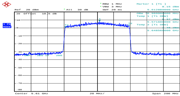
ax80_5610MHz_RU_Full_Chain 0 76.960MHz
