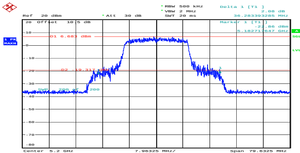
ax20_5200MHz_RU_Full_Chain 0 36.283MHz
