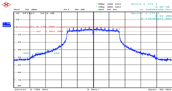
a_5785MHz_Chain 0 16.387MHz
