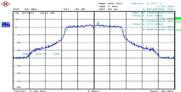
n20_5580MHz_Chain 0 18.189MHz
