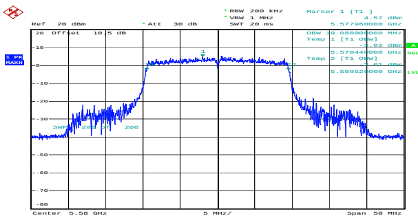
ax20_5580MHz_RU_Full_Chain 0 19.080MHz
