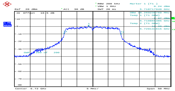
n20_5720MHz_Chain 0 18.269MHz
