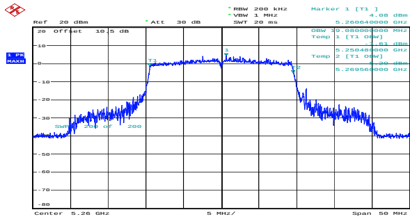
ax20_5260MHz_RU_Full_Chain 0 19.080MHz
