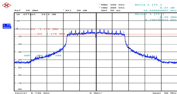
n20_5745MHz_Chain 0 16.667MHz
