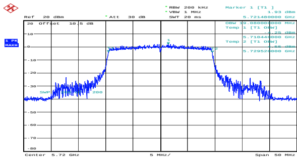
ax20_5720MHz_RU_Full_Chain 0 19.080MHz
