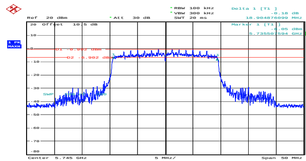
ax20_5745MHz_RU_Full_Chain_0_18.905MHz
