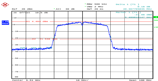
n40_5510MHz_Chain 0 40.368MHz
