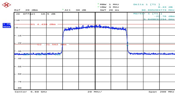
ax80_5690MHz_RU_Full_Chain 0 80.895MHz
