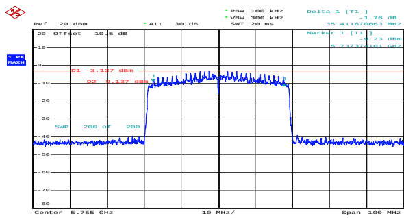
ax40_5755MHz_RU_Full_Chain 0 35.412MHz
