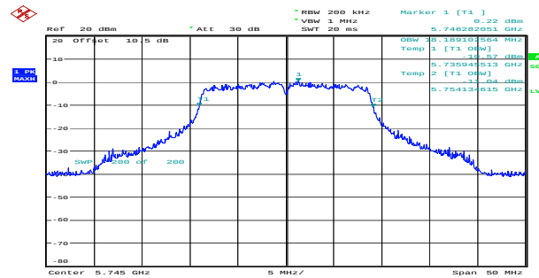
n20_5745MHz_Chain 0 18.189MHz
