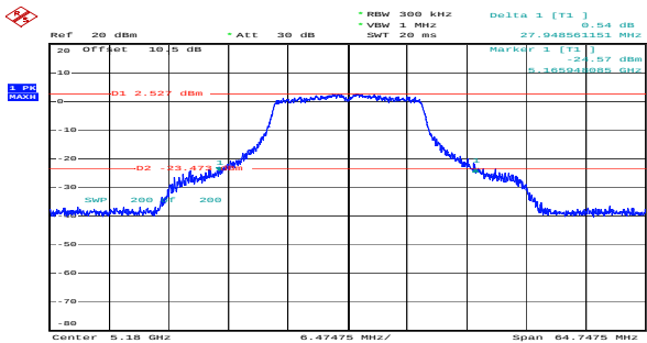
a_5180MHz_Chain 0 27.949MHz
