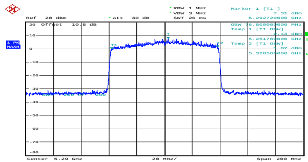
ax80_5290MHz_RU_Full_Chain_0_76.800MHz
