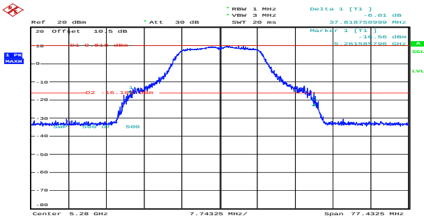
n20_5280MHz_Chain 0 37.819MHz
