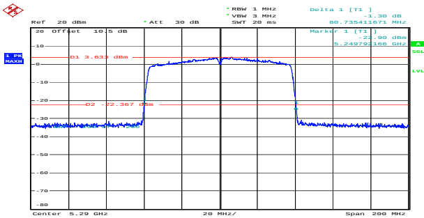
ac80_5290MHz_Chain 0 80.735MHz
