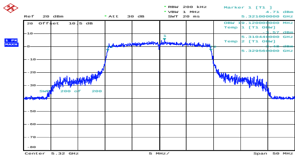
ax20_5320MHz_RU_Full_Chain 0 19.120MHz
