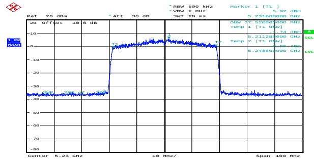
ax40_5230MHz_RU_Full_Chain 0 37.520MHz
