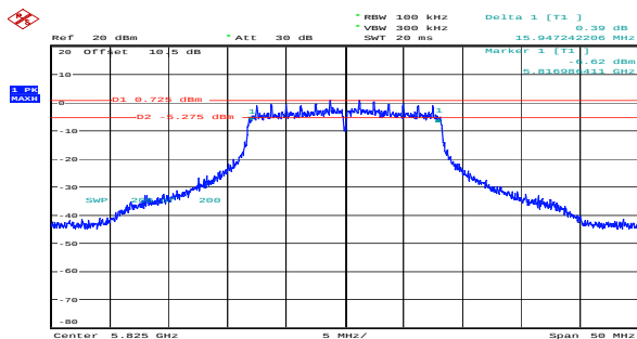
a_5825MHz_Chain 0 15.947MHz
