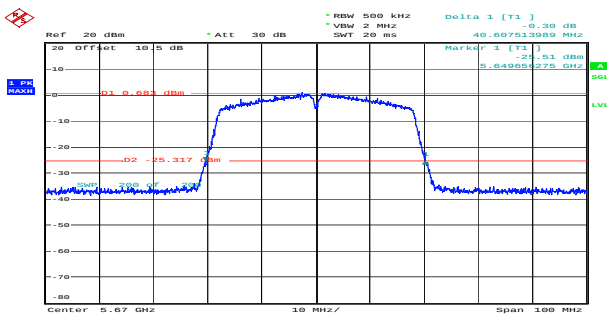
n40_5670MHz_Chain 0 40.608MHz
