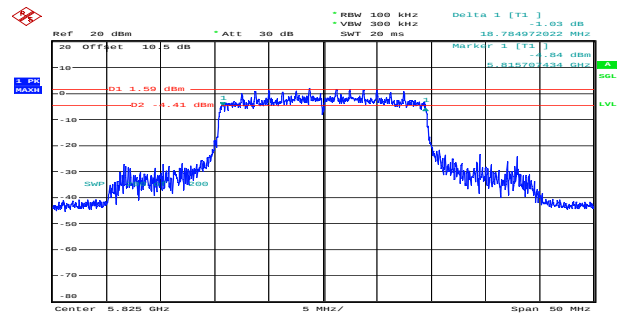
ax20_5825MHz_RU_Full_Chain 0 18.785MHz
