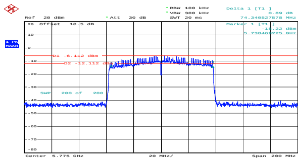
ac80_5775MHz_Chain 0 74.341MHz
