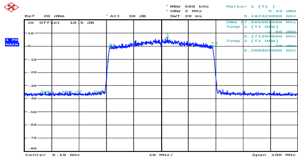
ax40_5190MHz_RU_Full_Chain 0 37.600MHz
