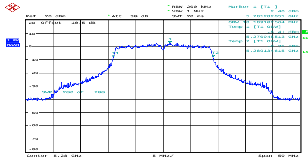
n20_5280MHz_Chain 0 18.189MHz
