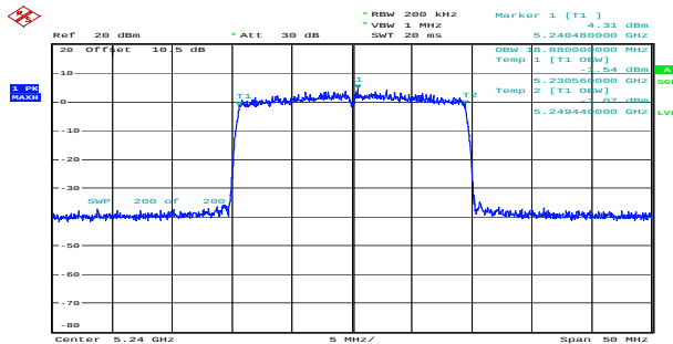
ax20_5240MHz_RU_Full_Chain 0 18.880MHz
