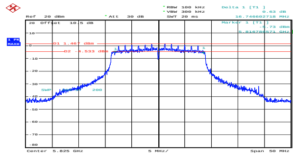
n20_5825MHz_Chain 0 16.747MHz
