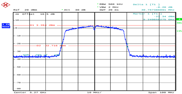
n40_5270MHz_Chain 0 40.767MHz
