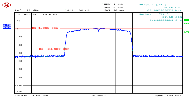
ac80_5690MHz_Chain 0 80.895MHz
