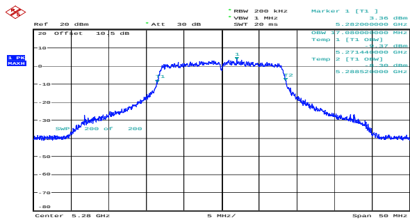
a_5280MHz_Chain 0 17.080MHz
