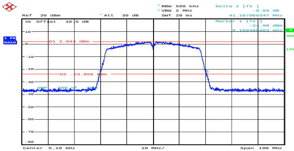
n40_5190MHz_Chain 0 41.167MHz
