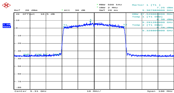
ax40_5310MHz_RU_Full_Chain 0 37.520MHz
