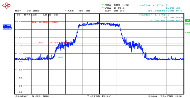
ax20_5580MHz_RU_Full_Chain 0 36.383MHz
