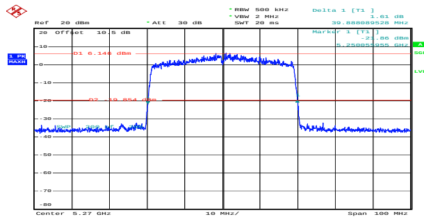
ax40_5270MHz_RU_Full_Chain 0 39.888MHz
