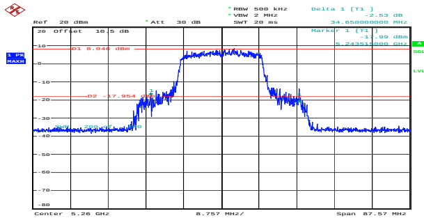
ax20_5260MHz_RU_Full_Chain 0 34.650MHz
