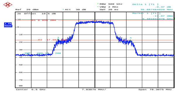
ax20_5500MHz_RU_Full_Chain 0 35.867MHz
