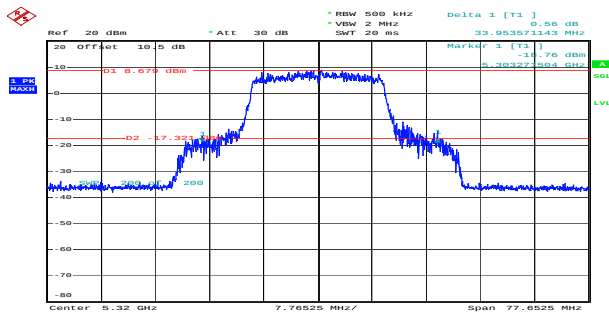
ax20_5320MHz_RU_Full_Chain 0 33.954MHz
