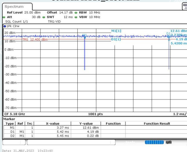
802.11n HT20_5180MHz
