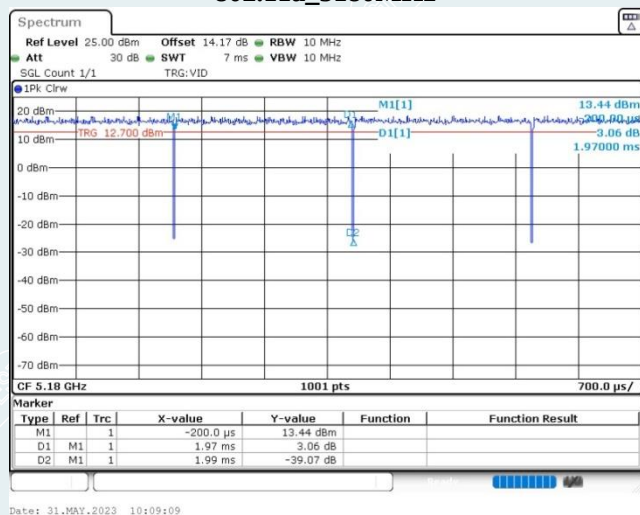
802.11a_5180MHz
