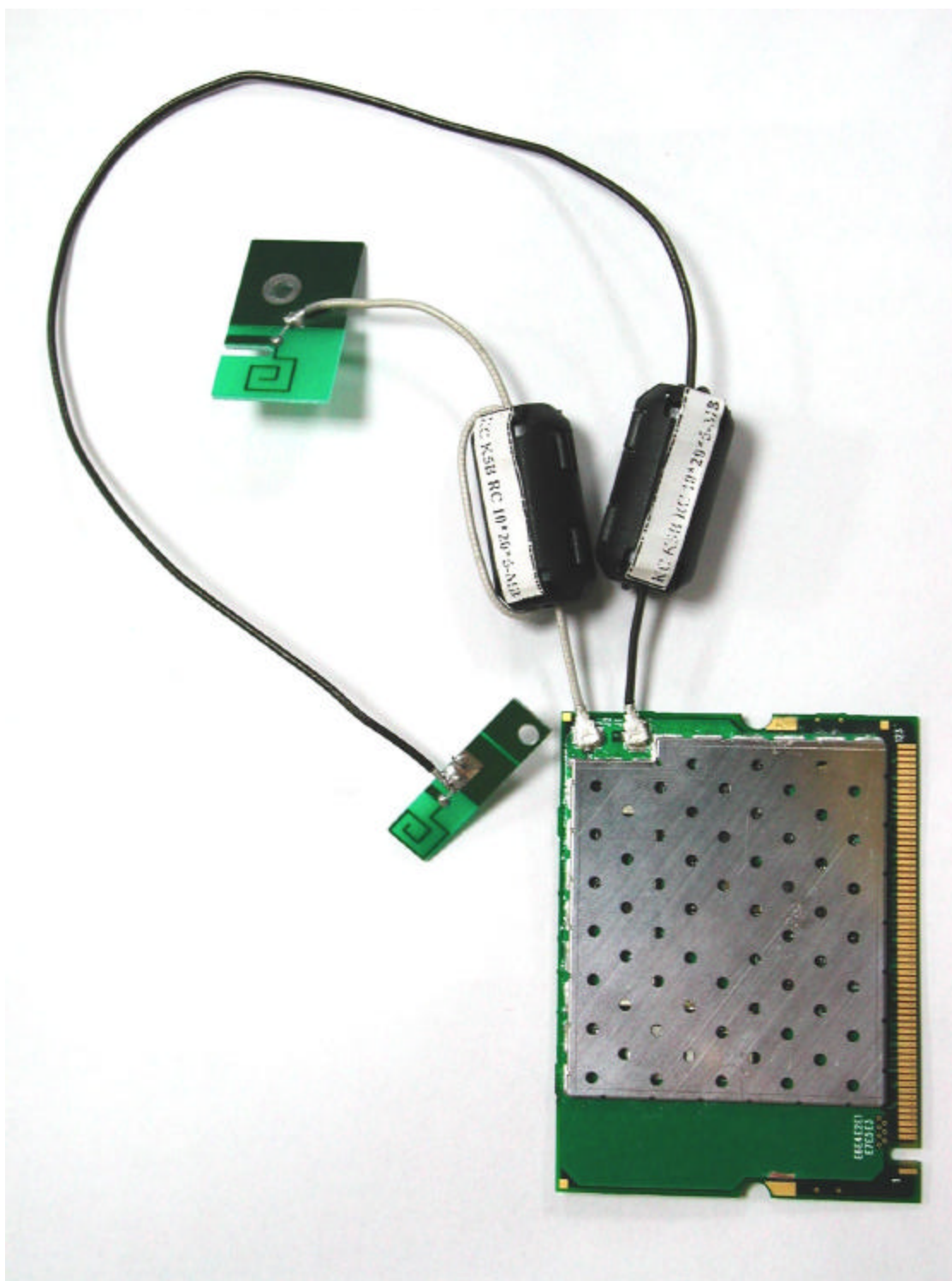
FCC ID: JVPWL200 External Photo includes Antenna and PWBA.
