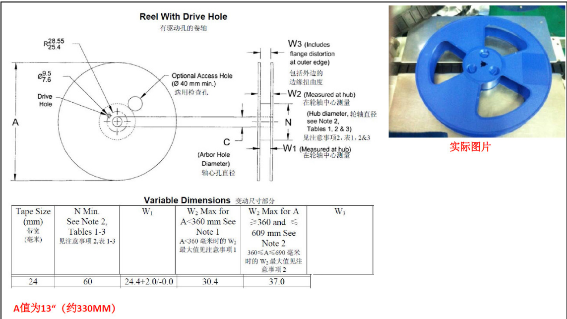
Figure 18: Reel specifications
