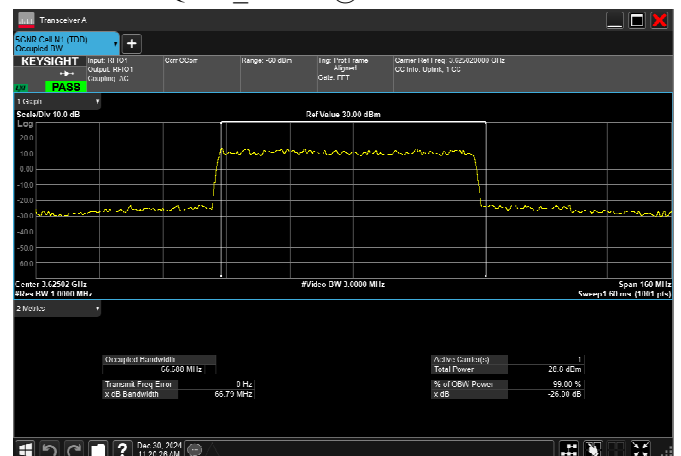
n77_2_70MHz_30kHz_3625MHz_DFT-s-OFDM 16 QAM_RB180@0 66.688MHz
