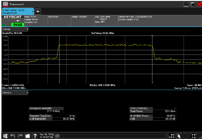
n77_2_60MHz_30kHz_3625MHz_CP-OFDM 256 QAM_RB162@0 57.842MHz
