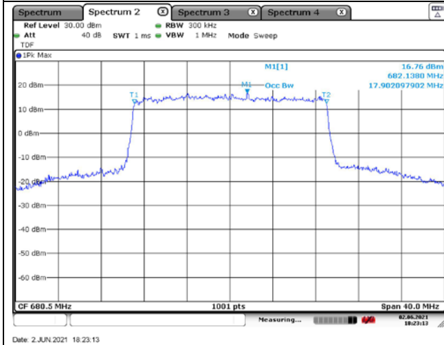
20 MHz QPSK Middle Channel - Full RB
