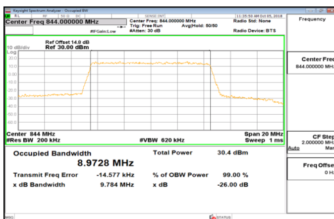
Band5_10MHz_64QAM_50_0_HighCH20600-844
