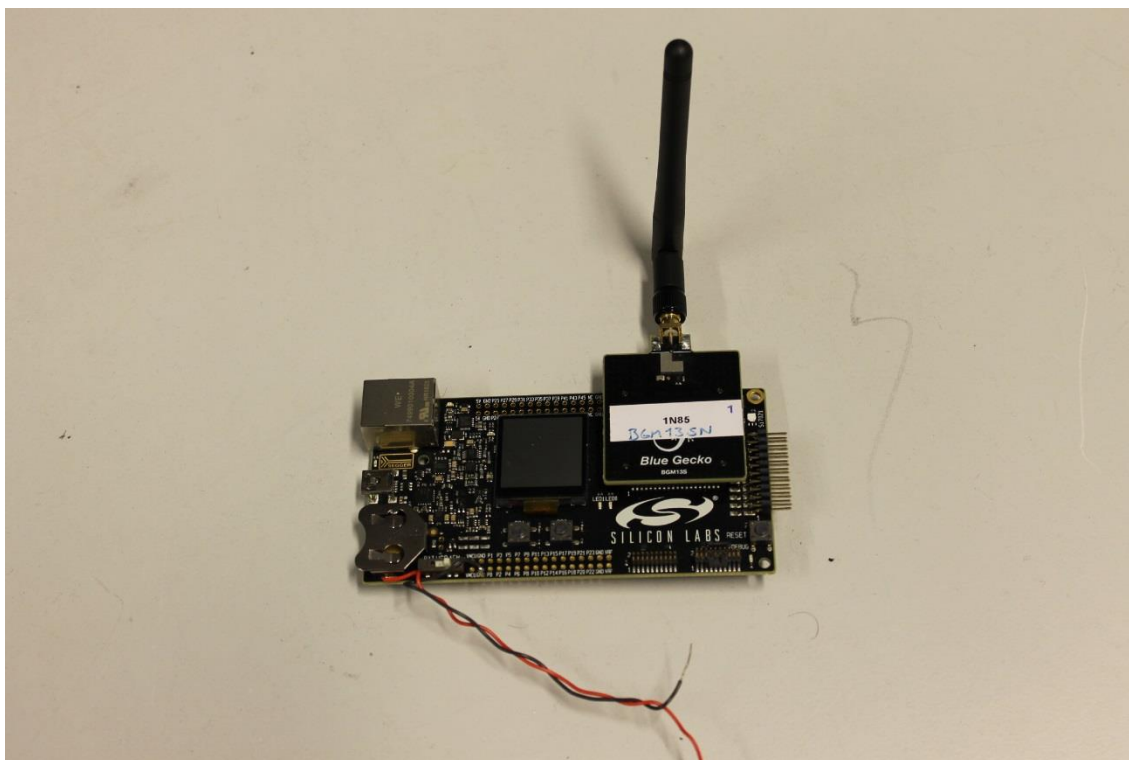
Photograph 1. DUT 1, BGM13SN
